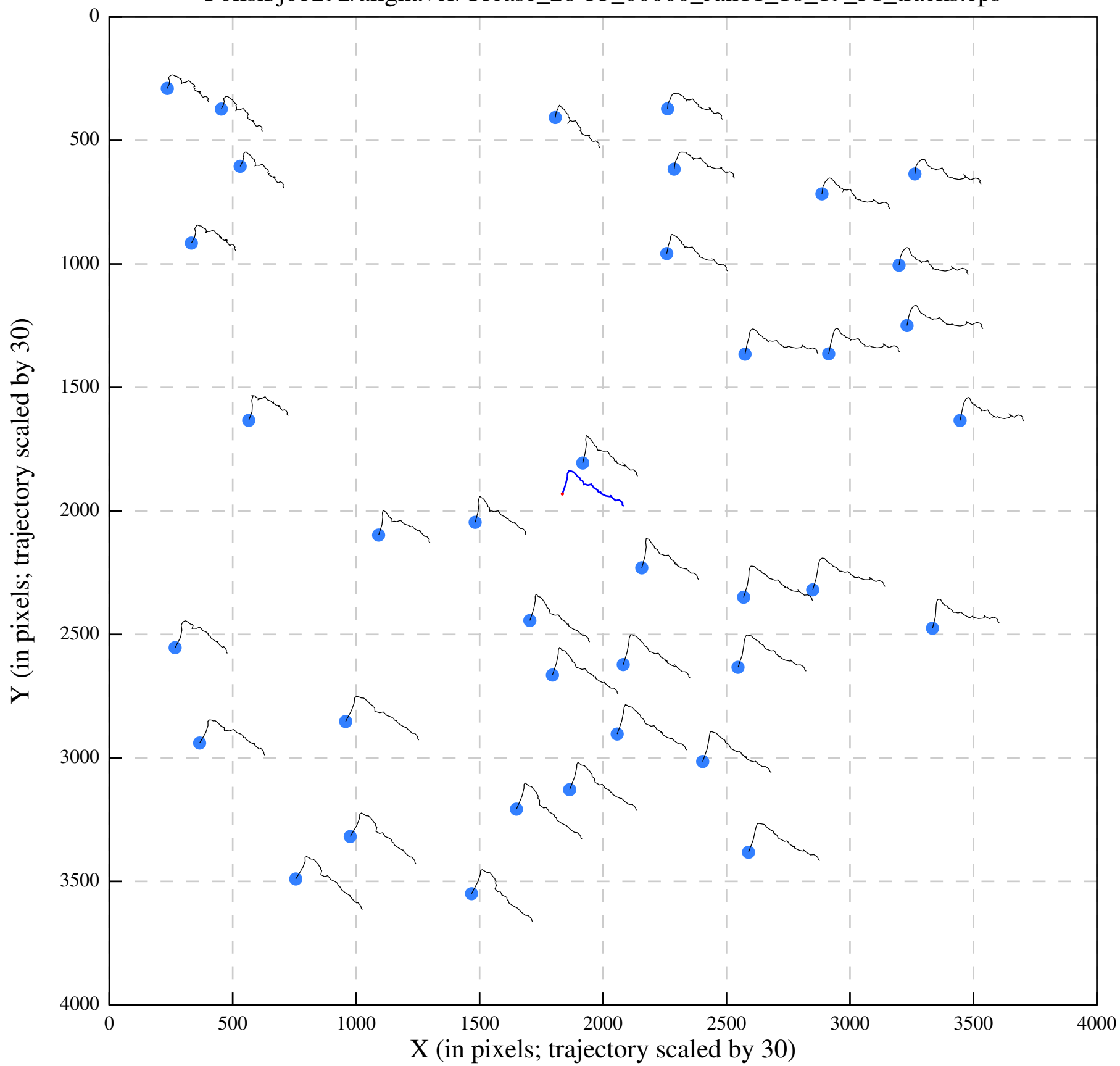
Polish/job292/alignaver/Urease_28-33_00000_Jan11_18_19_31_tracks.eps
