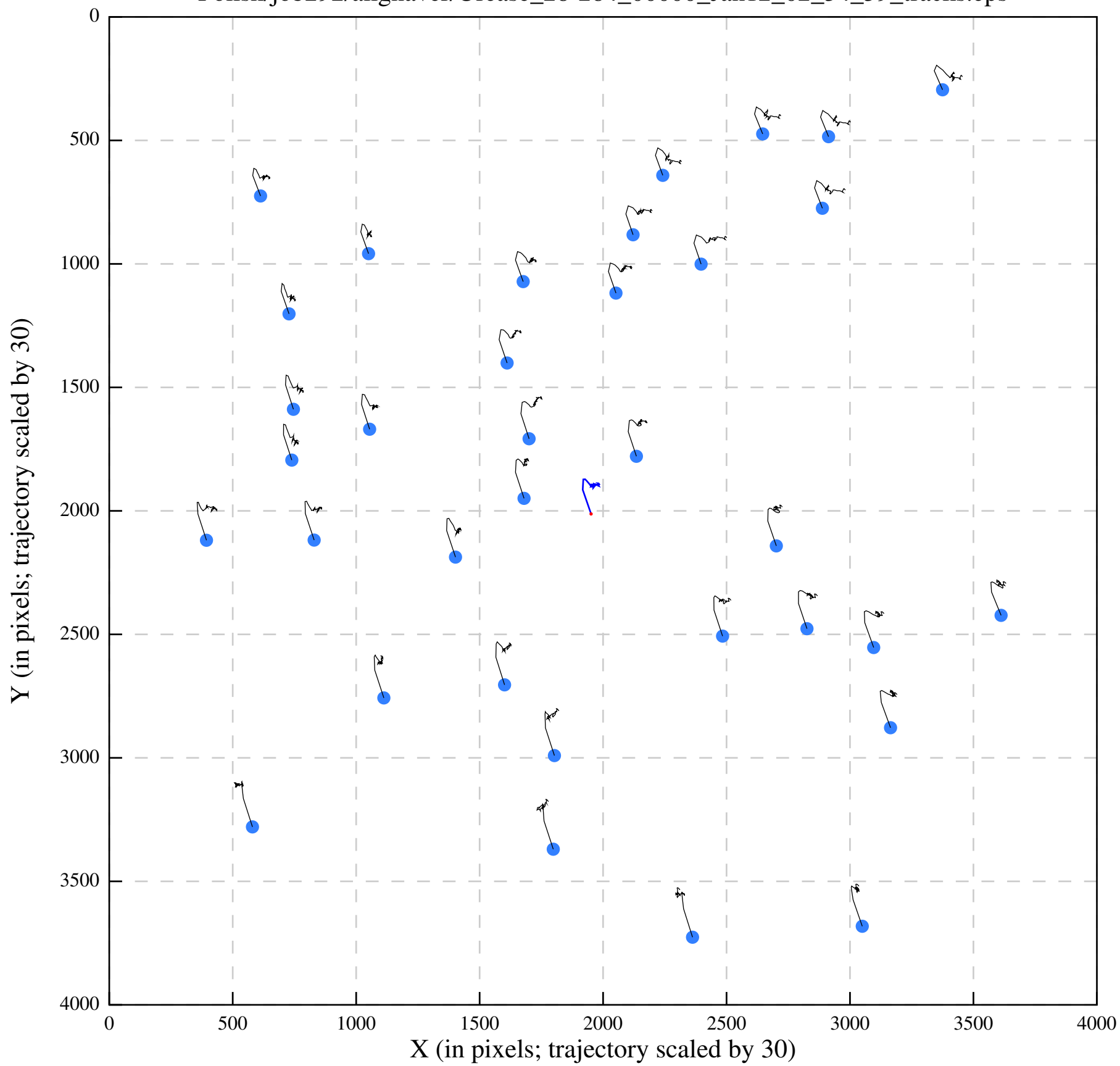
Polish/job292/alignaver/Urease_28-284_00000_Jan12_02_34_59_tracks.eps
