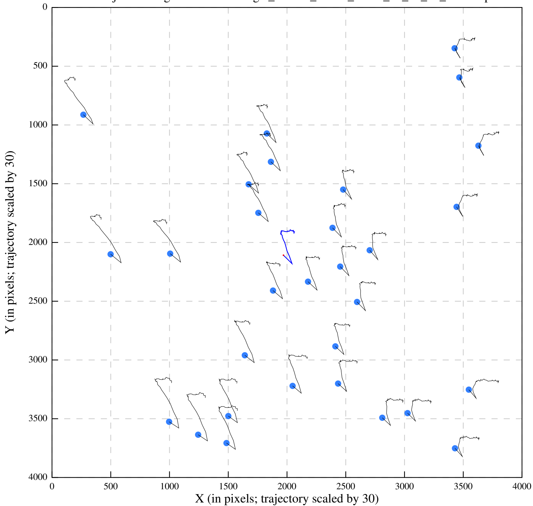
Polish/job292/alignaver/UreaseSingle_47-582_00000_Jan14_14_40_12_tracks.eps
