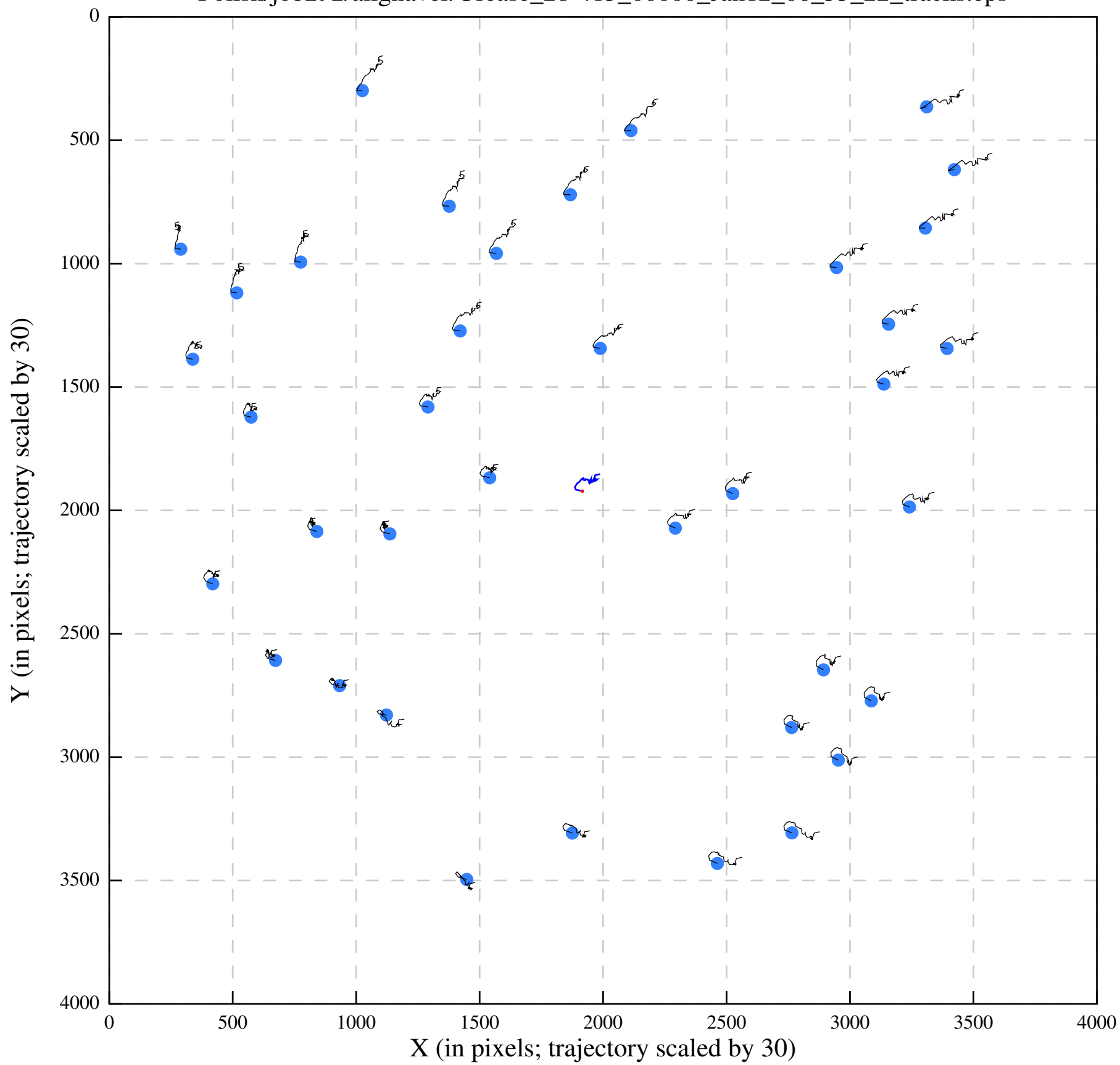
Polish/job292/alignaver/Urease_28-413_00000_Jan12_06_55_22_tracks.eps
