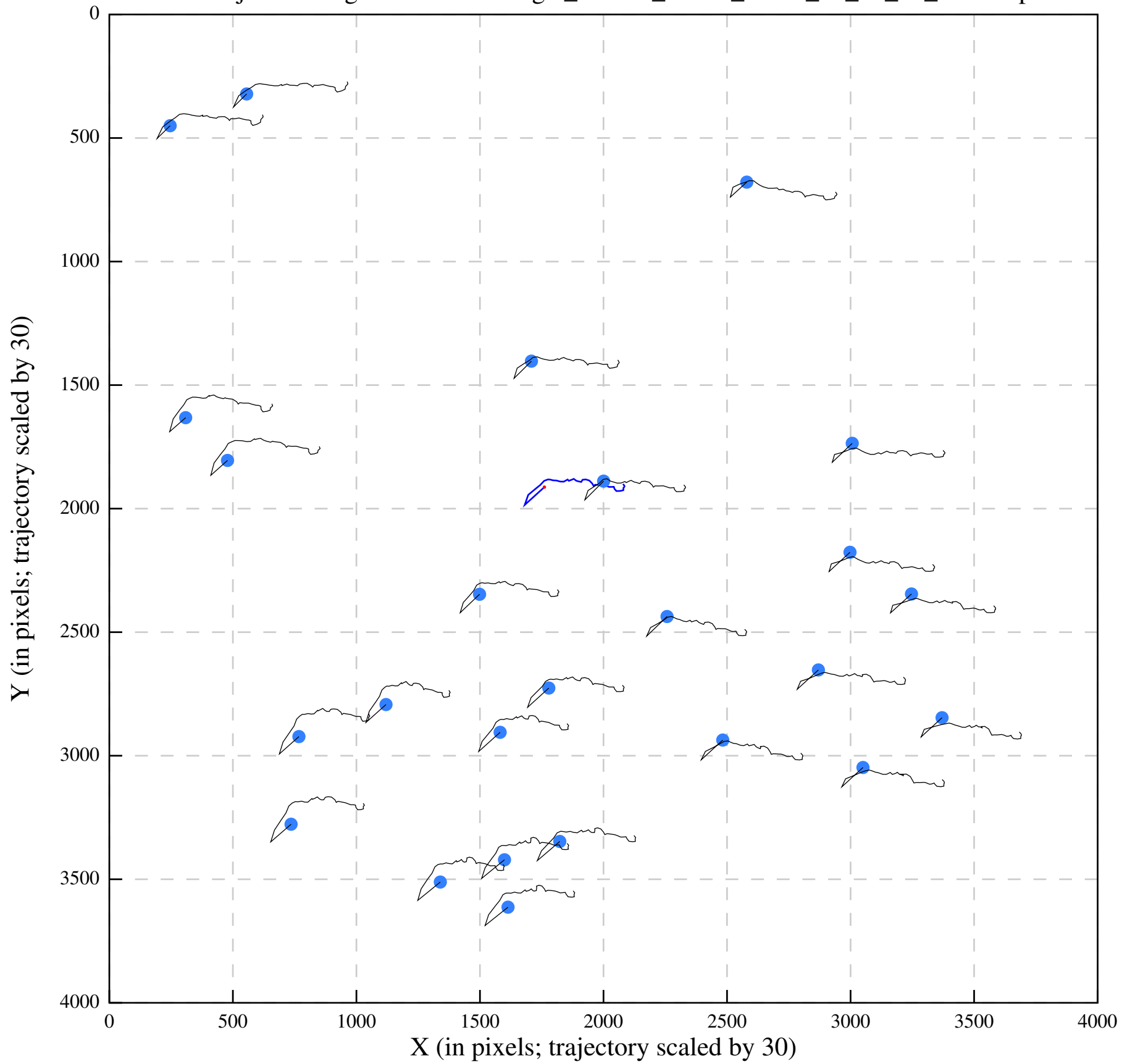
Polish/job292/alignaver/UreaseSingle_47-233_00000_Jan14_10_29_00_tracks.eps
