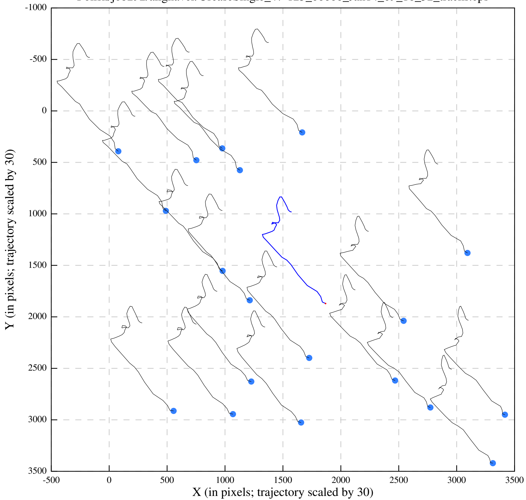
Polish/job292/alignaver/UreaseSingle_47-125_00000_Jan14_09_16_52_tracks.eps
