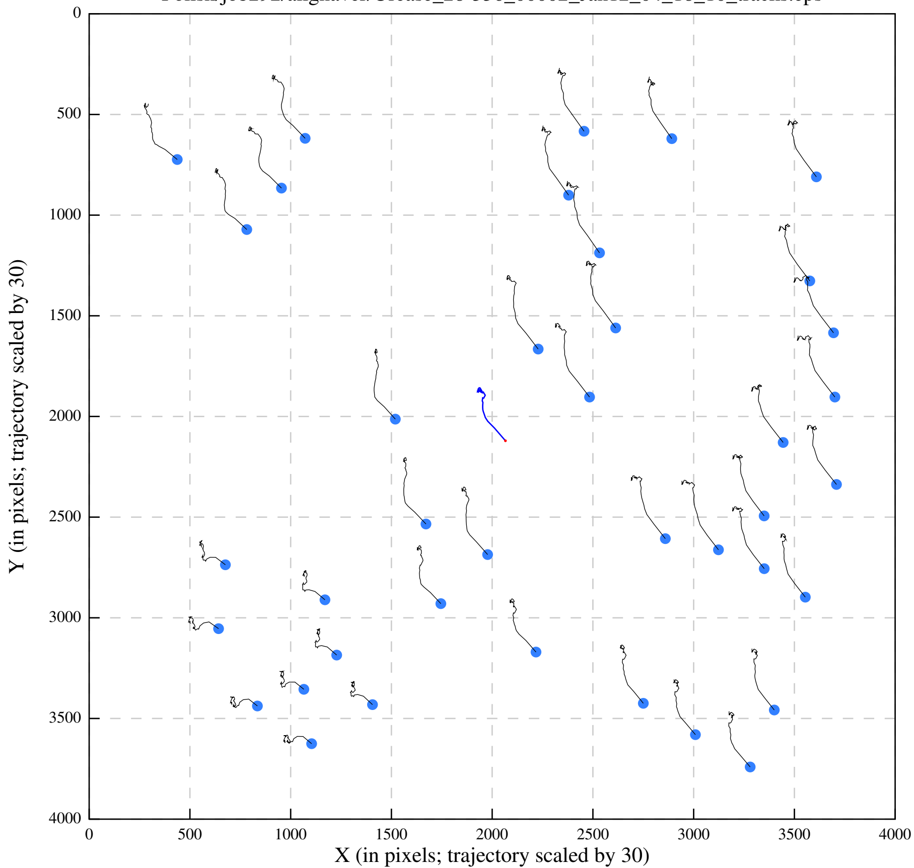
Polish/job292/alignaver/Urease_28-336_00002_Jan12_04_18_10_tracks.eps
