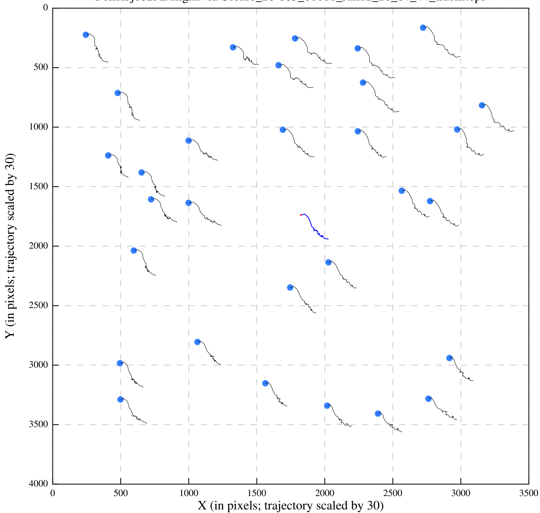
Polish/job292/alignaver/Urease_28-863_00001_Jan12_20_04_44_tracks.eps
