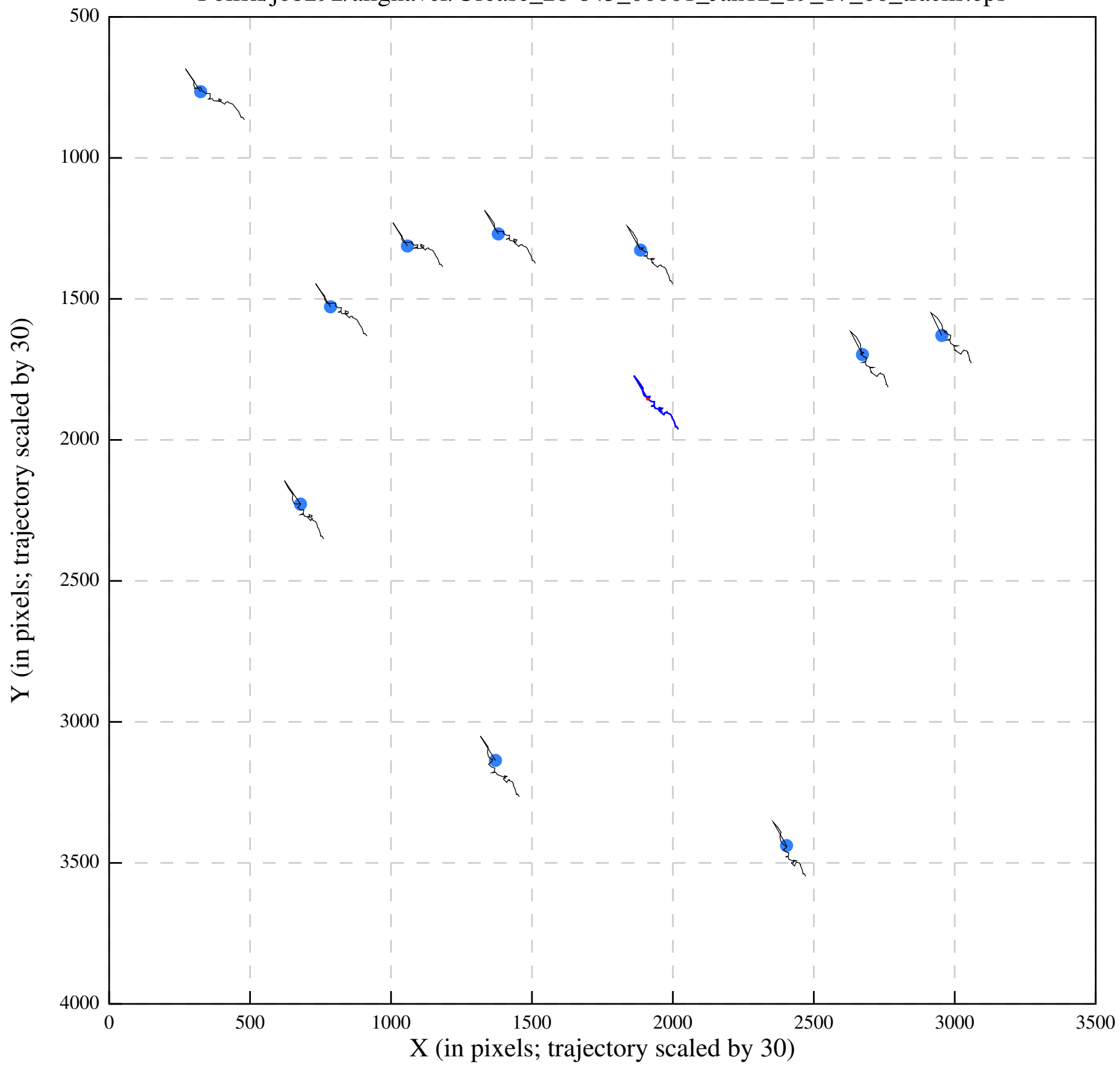
Polish/job292/alignaver/Urease_28-843_00001_Jan12_19_17_00_tracks.eps
