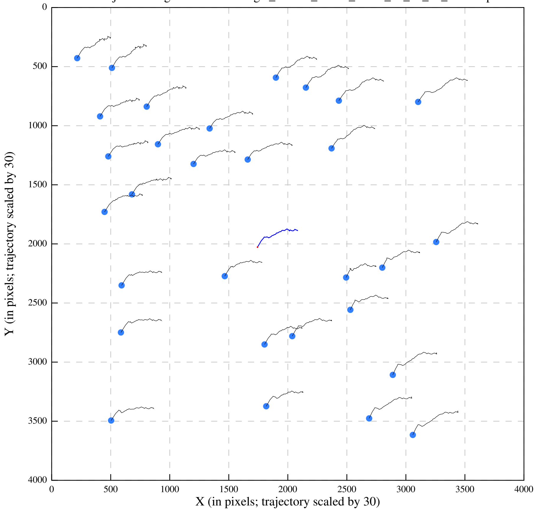
Polish/job292/alignaver/UreaseSingle_35-272_00000_Jan13_15_23_29_tracks.eps
