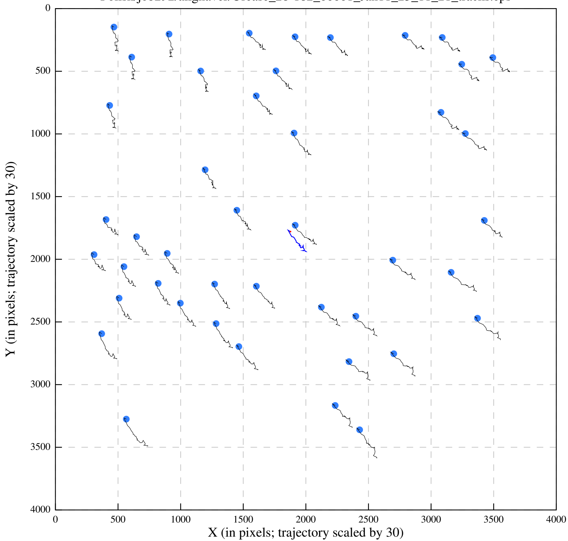
Polish/job292/alignaver/Urease_28-182_00001_Jan11_23_11_21_tracks.eps
