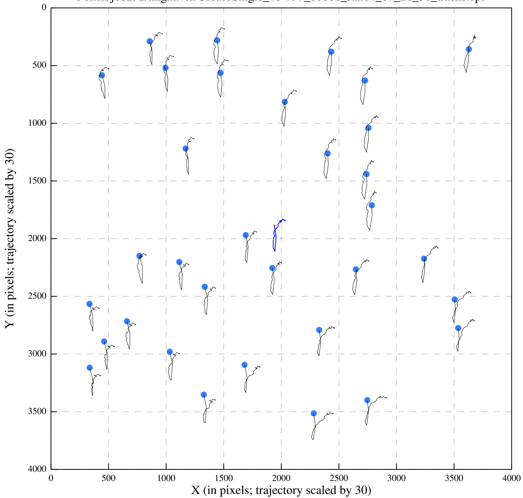
Polish/job292/alignaver/UreaseSingle_41-797_00000_Jan14_07_21_31_tracks.eps
