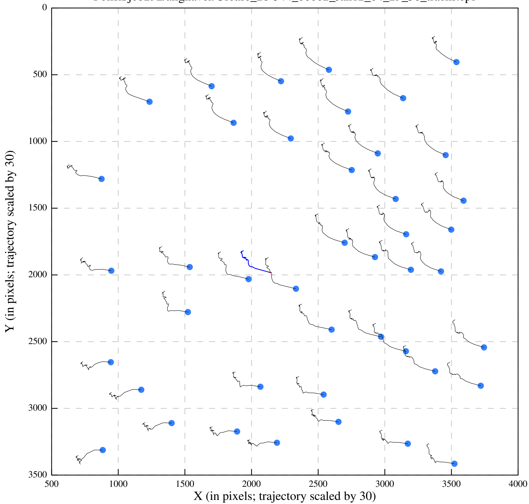
Polish/job292/alignaver/Urease_28-344_00002_Jan12_04_29_56_tracks.eps
