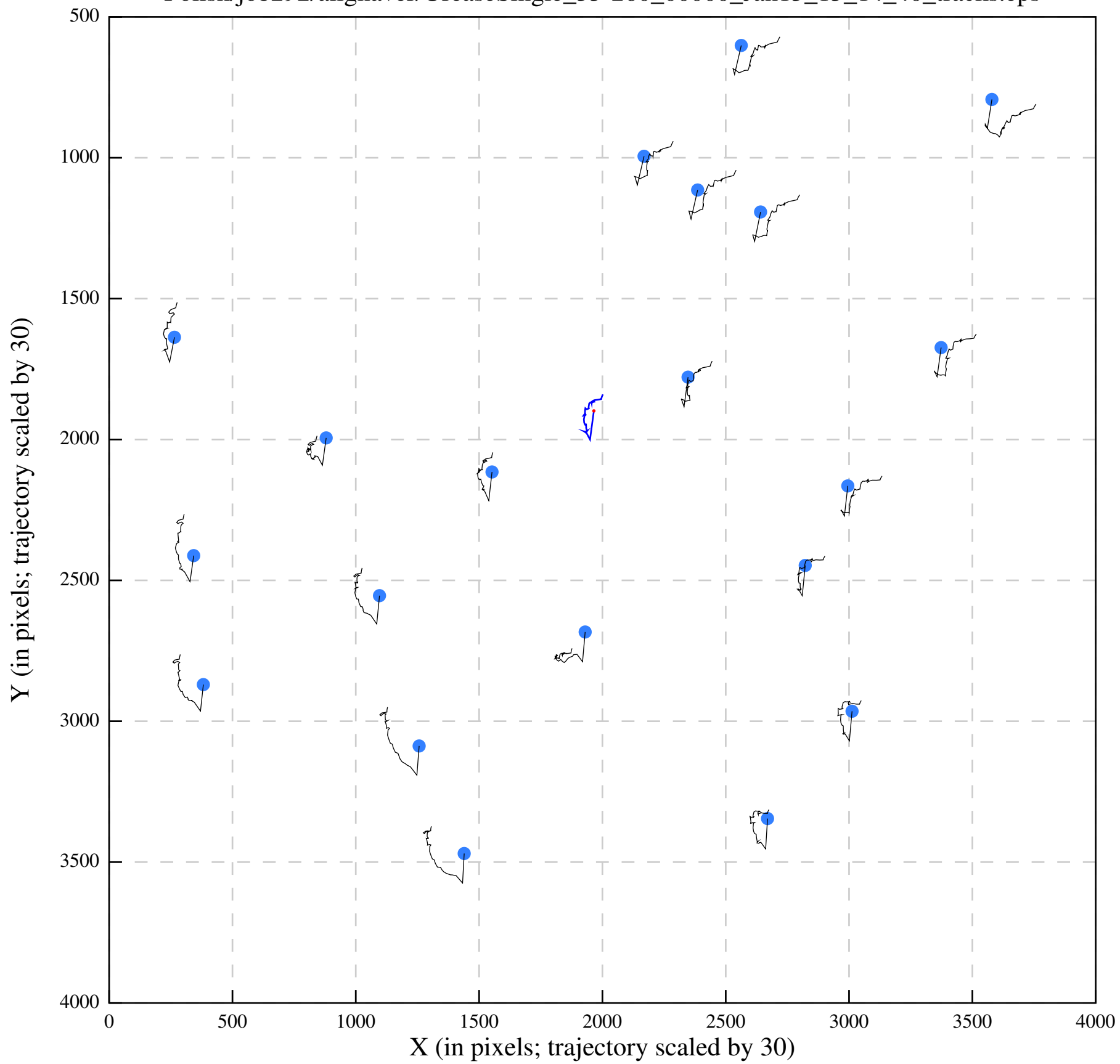
Polish/job292/alignaver/UreaseSingle_35-260_00000_Jan13_15_14_40_tracks.eps
