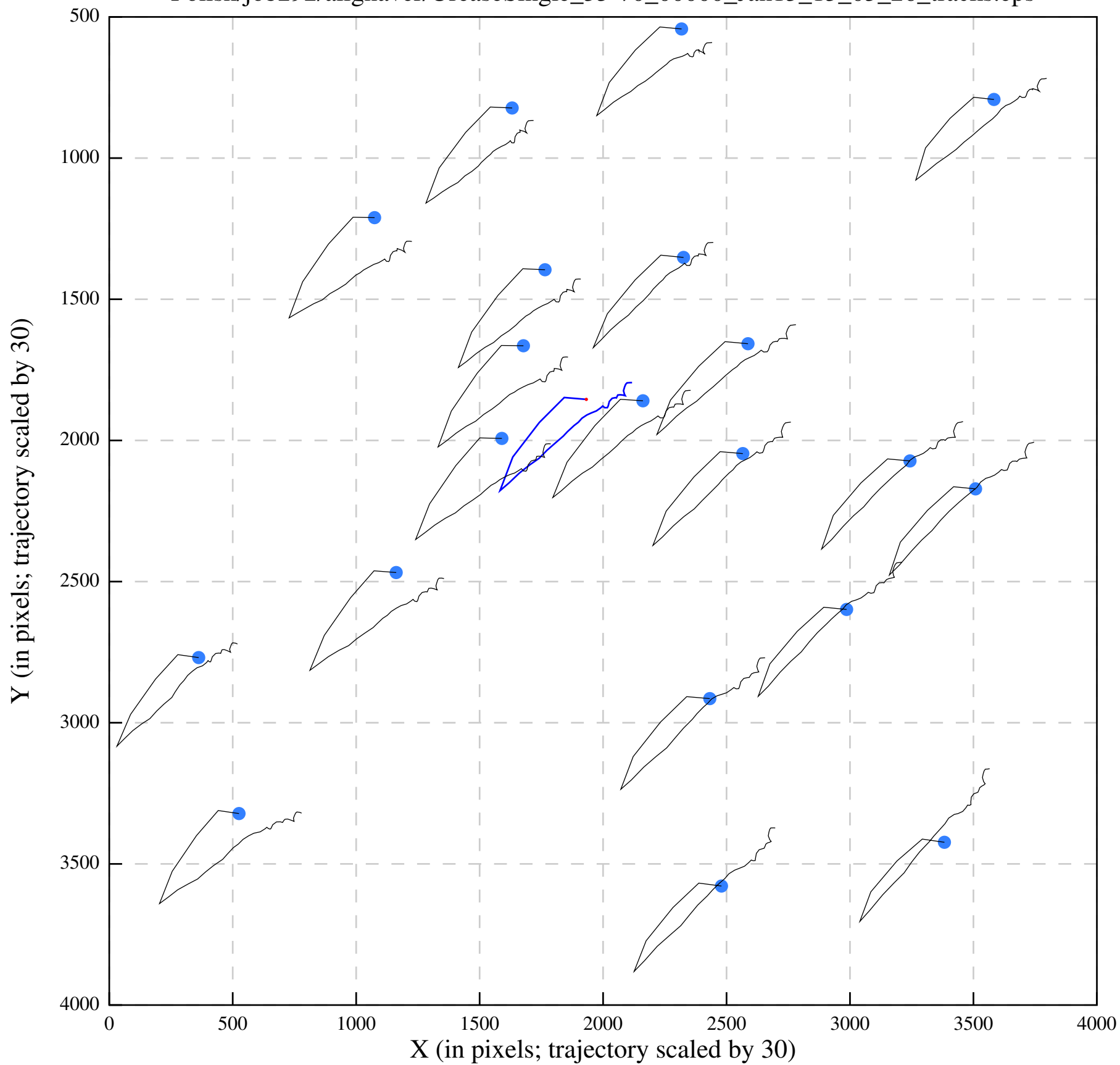
Polish/job292/alignaver/UreaseSingle_35-70_00000_Jan13_13_03_26_tracks.eps
