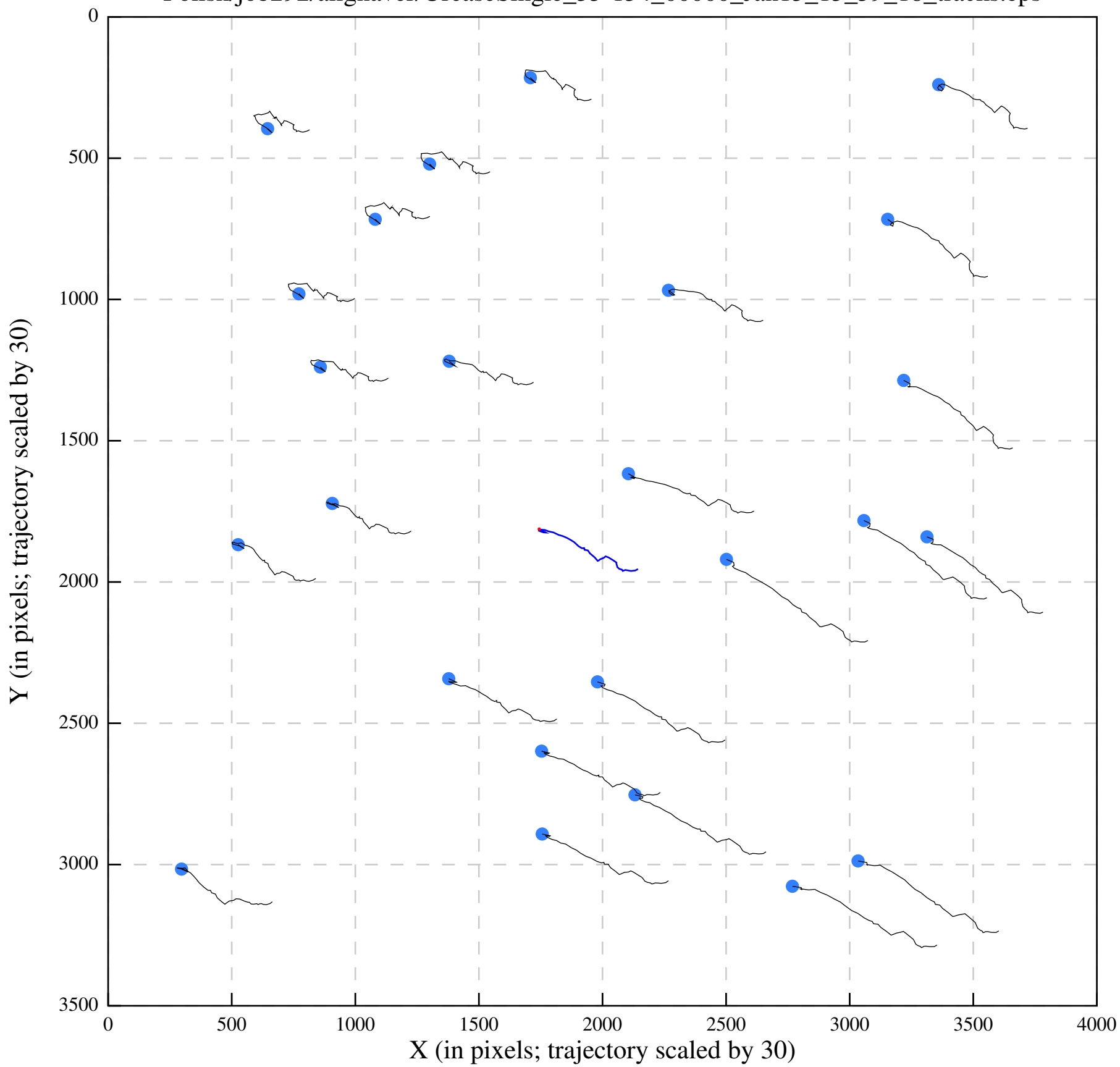
Polish/job292/alignaver/UreaseSingle_35-154_00000_Jan13_13_59_18_tracks.eps
