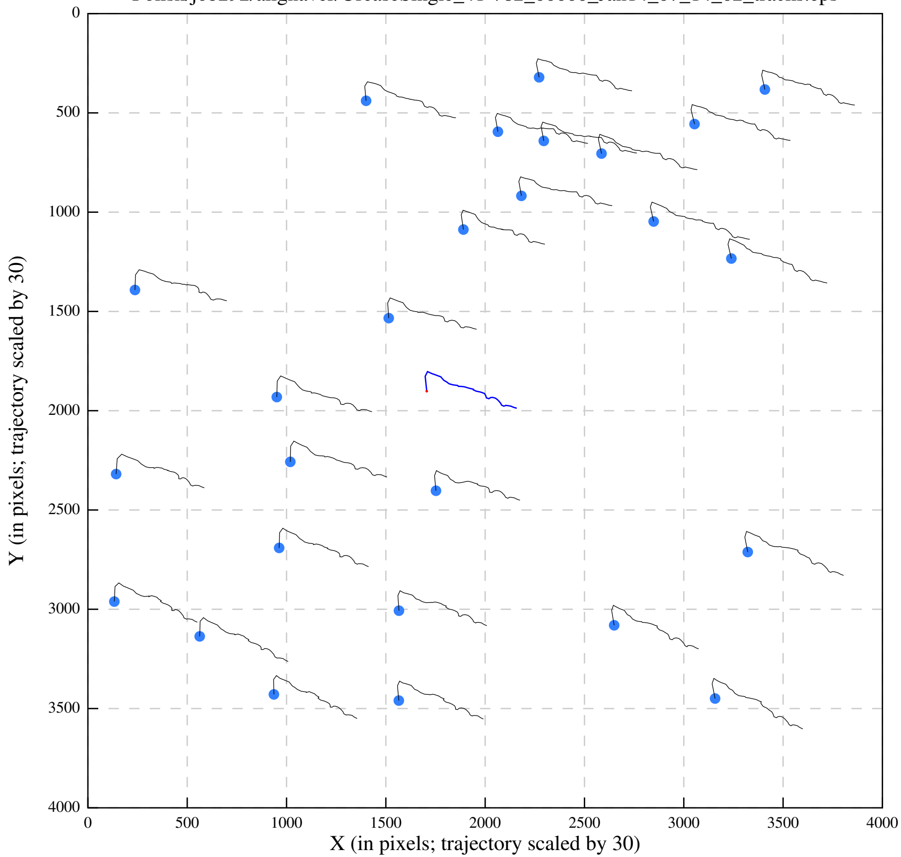
Polish/job292/alignaver/UreaseSingle_41-782_00000_Jan14_07_14_02_tracks.eps
