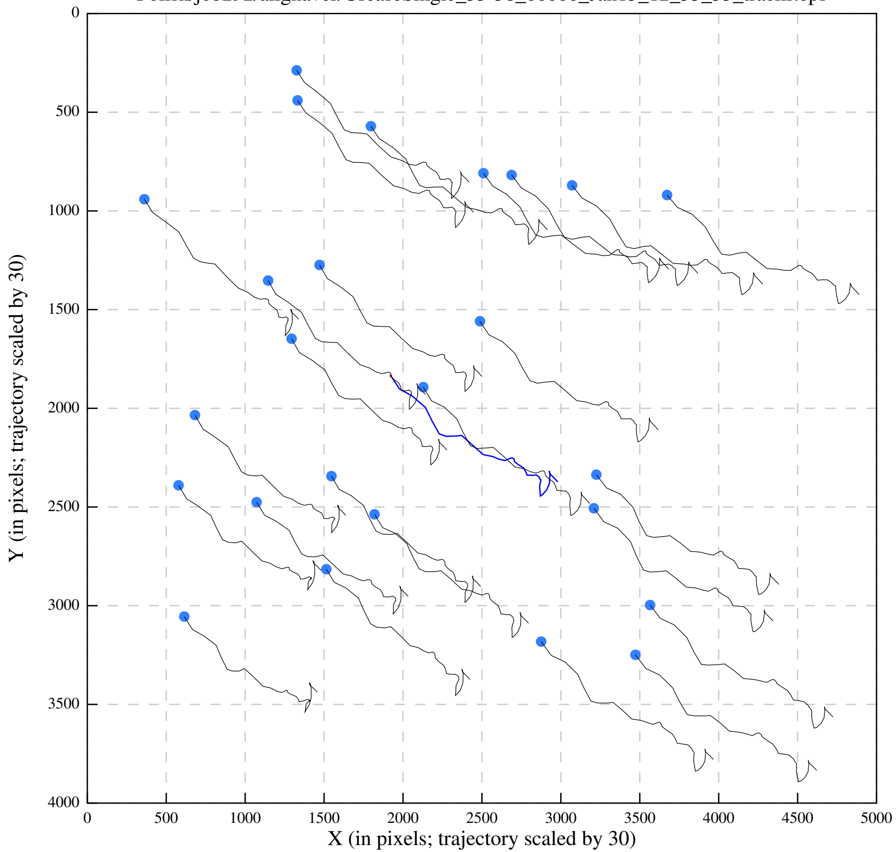
Polish/job292/alignaver/UreaseSingle_35-58_00000_Jan13_12_53_33_tracks.eps
