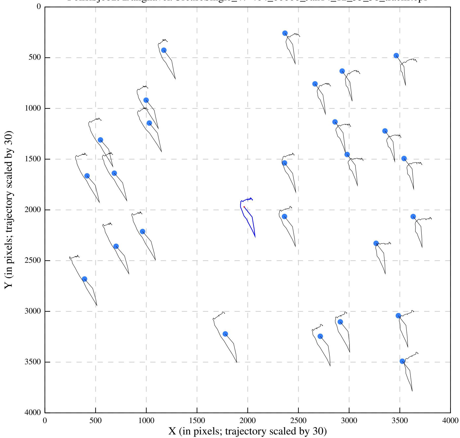
Polish/job292/alignaver/UreaseSingle_47-404_00000_Jan14_12_33_58_tracks.eps
