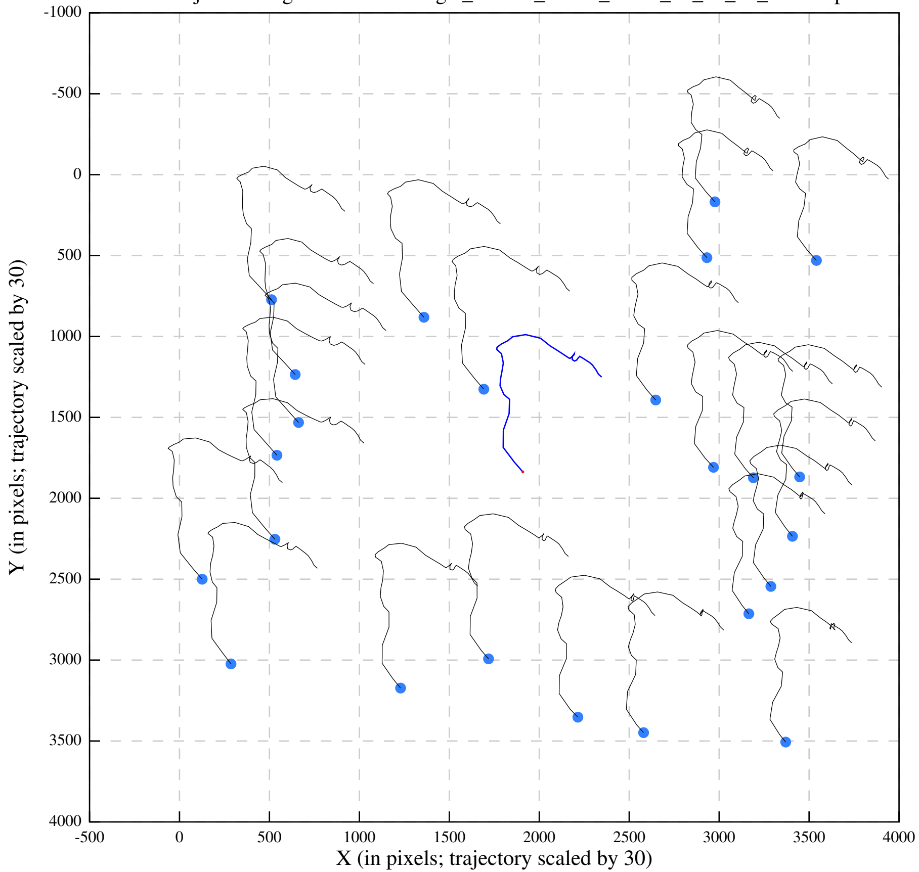
Polish/job292/alignaver/UreaseSingle_47-590_00000_Jan14_14_45_46_tracks.eps
