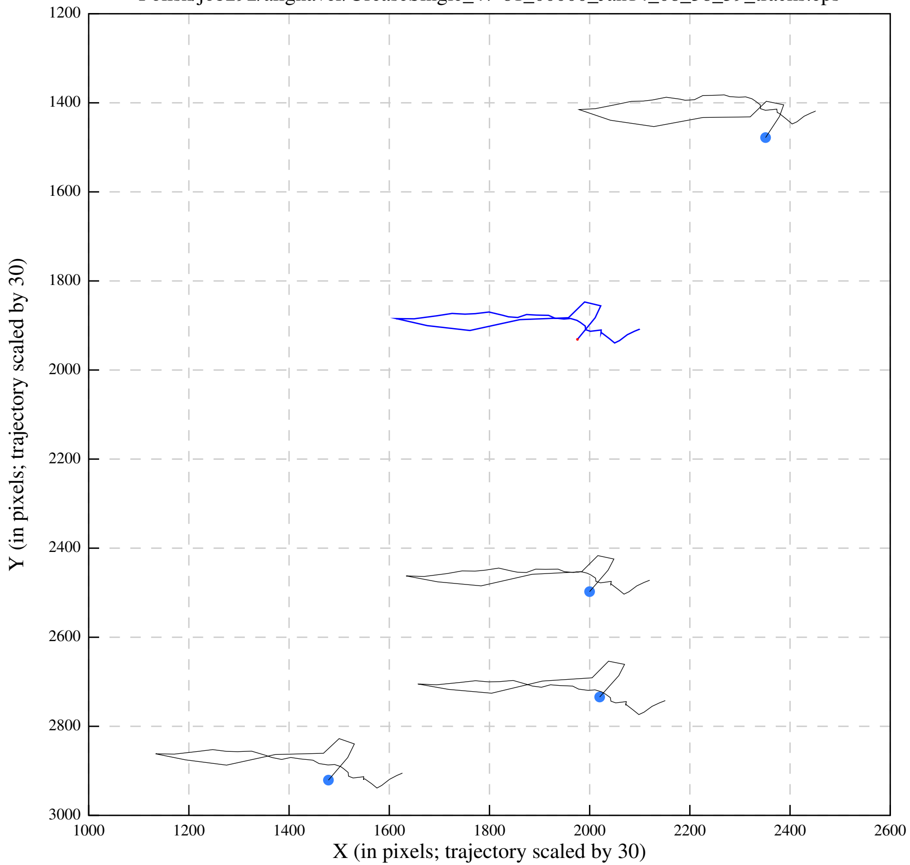
Polish/job292/alignaver/UreaseSingle_47-81_00000_Jan14_08_38_59_tracks.eps
