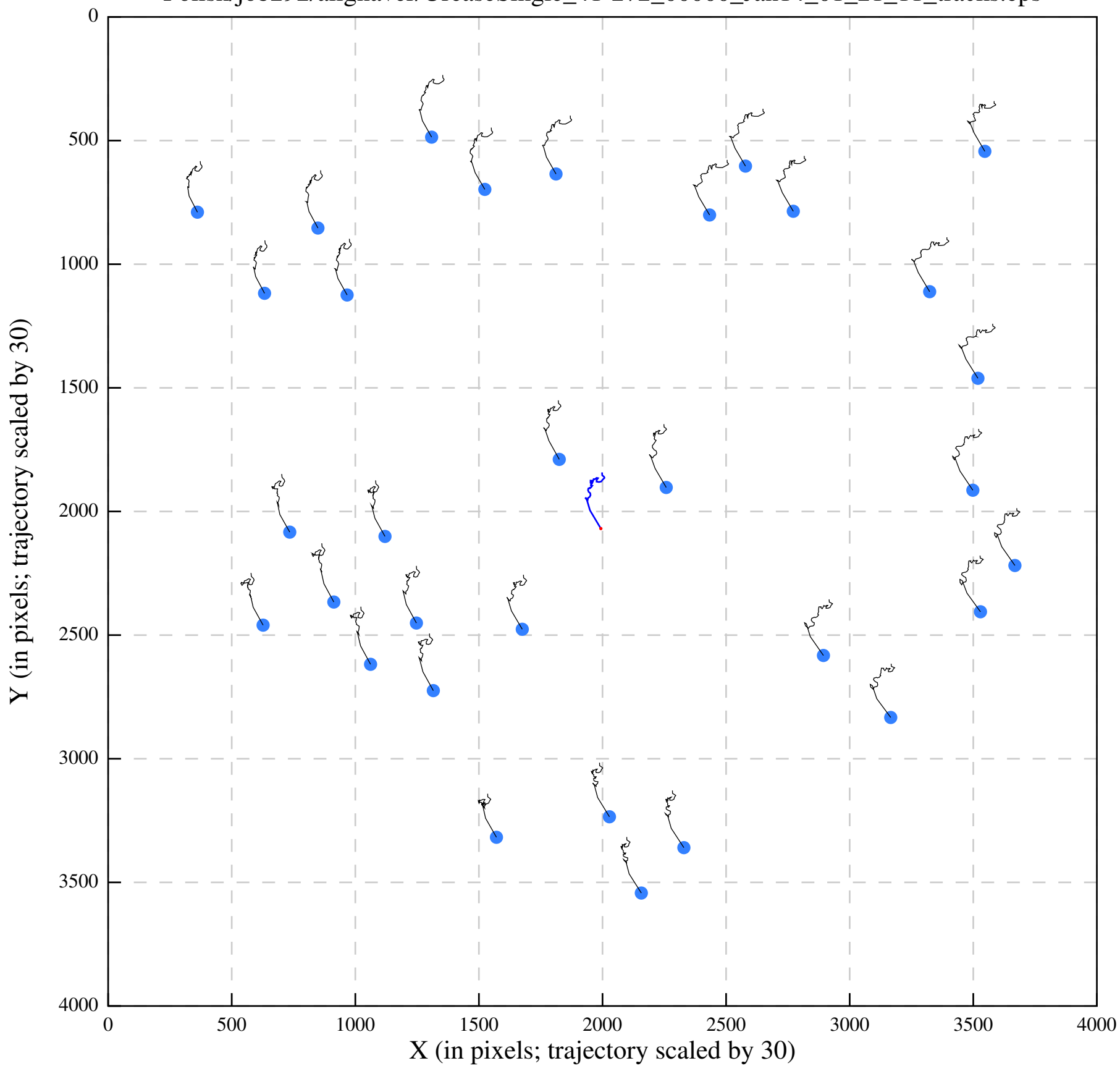
Polish/job292/alignaver/UreaseSingle_41-272_00000_Jan14_01_21_11_tracks.eps
