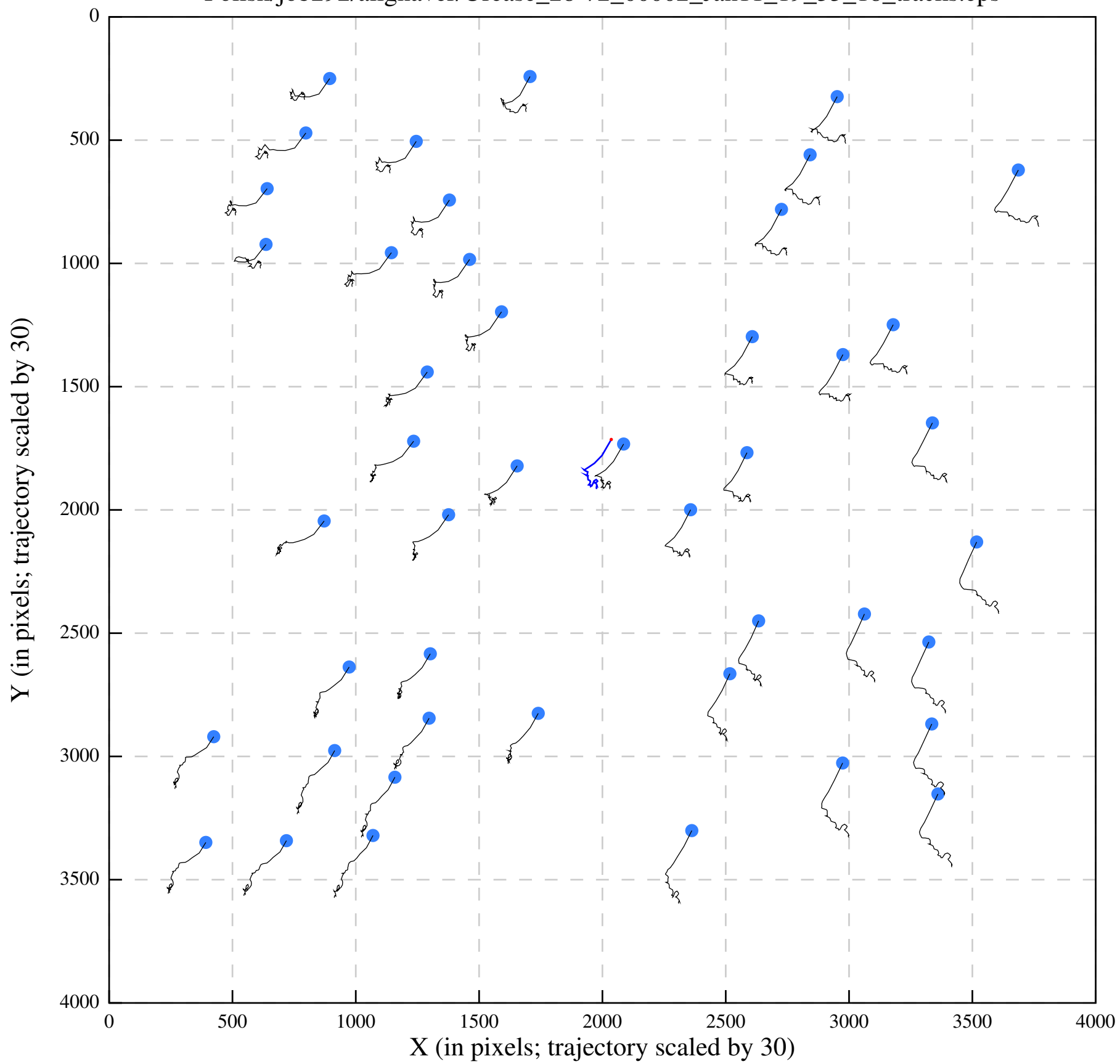
Polish/job292/alignaver/Urease_28-72_00002_Jan11_19_33_18_tracks.eps
