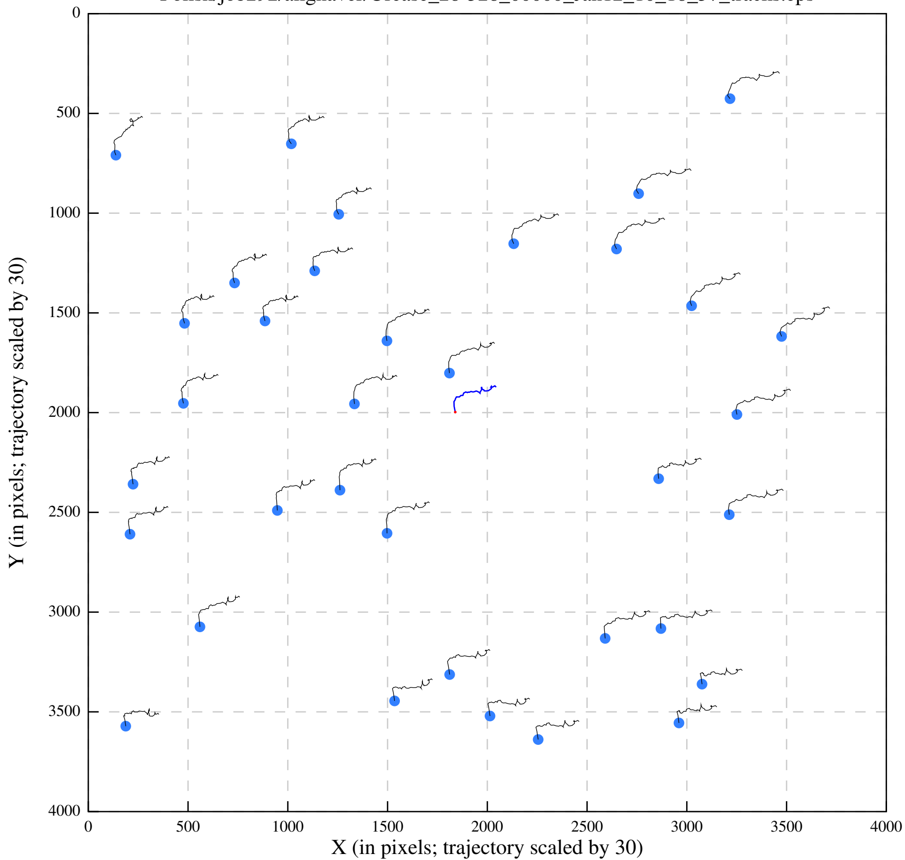
Polish/job292/alignaver/Urease_28-528_00000_Jan12_10_18_57_tracks.eps
