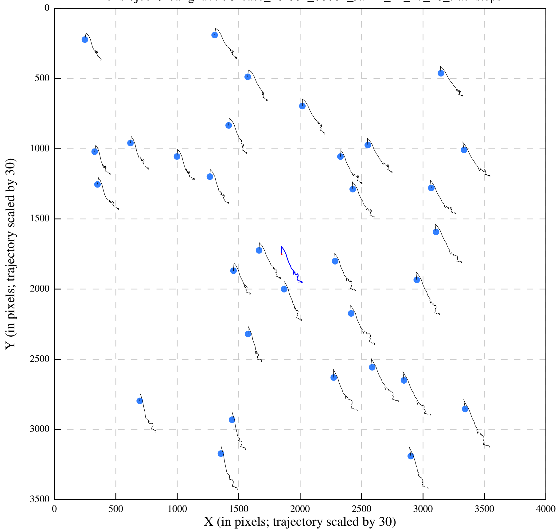
Polish/job292/alignaver/Urease_28-662_00001_Jan12_14_17_18_tracks.eps
