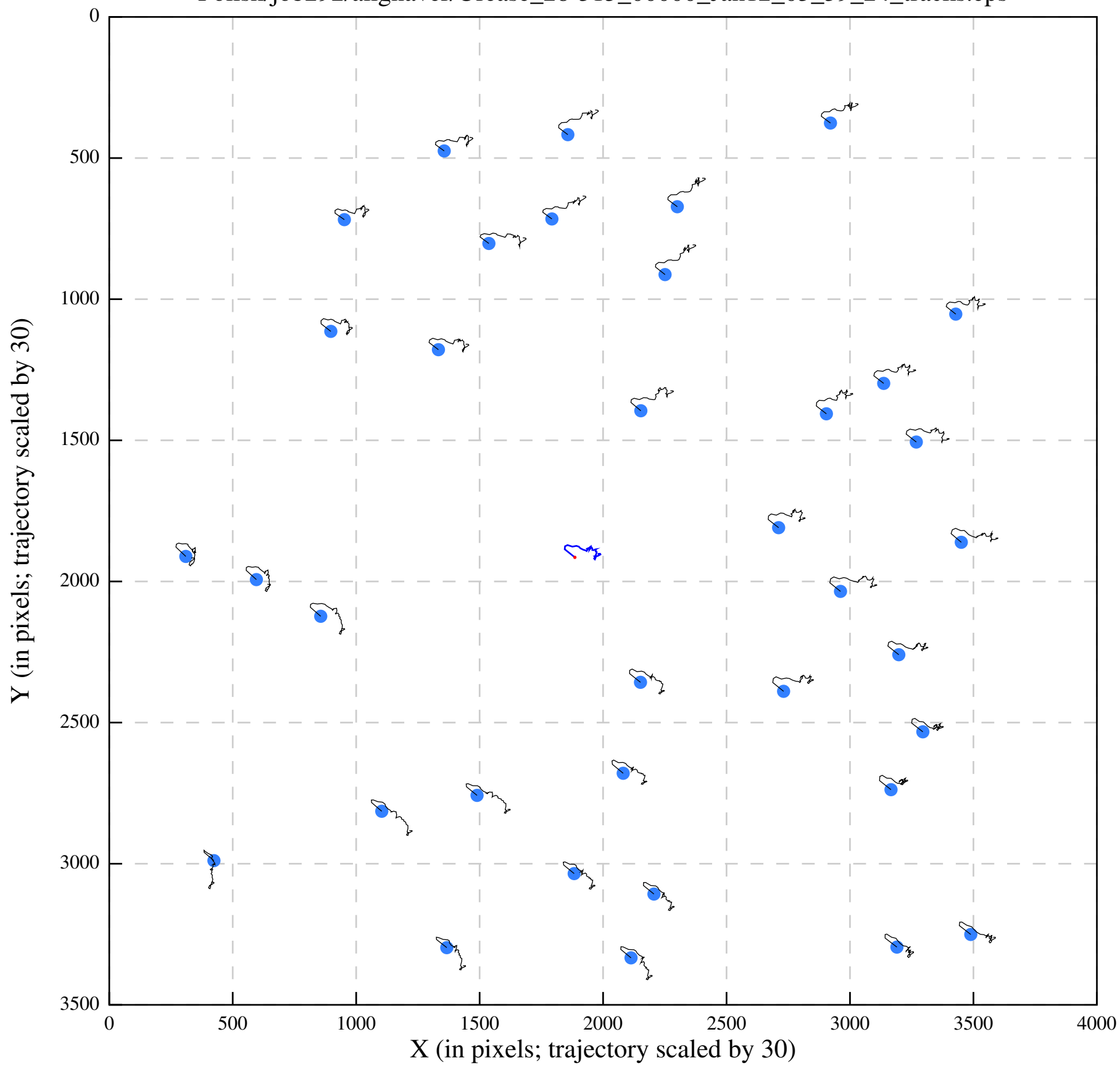
Polish/job292/alignaver/Urease_28-315_00000_Jan12_03_39_24_tracks.eps
