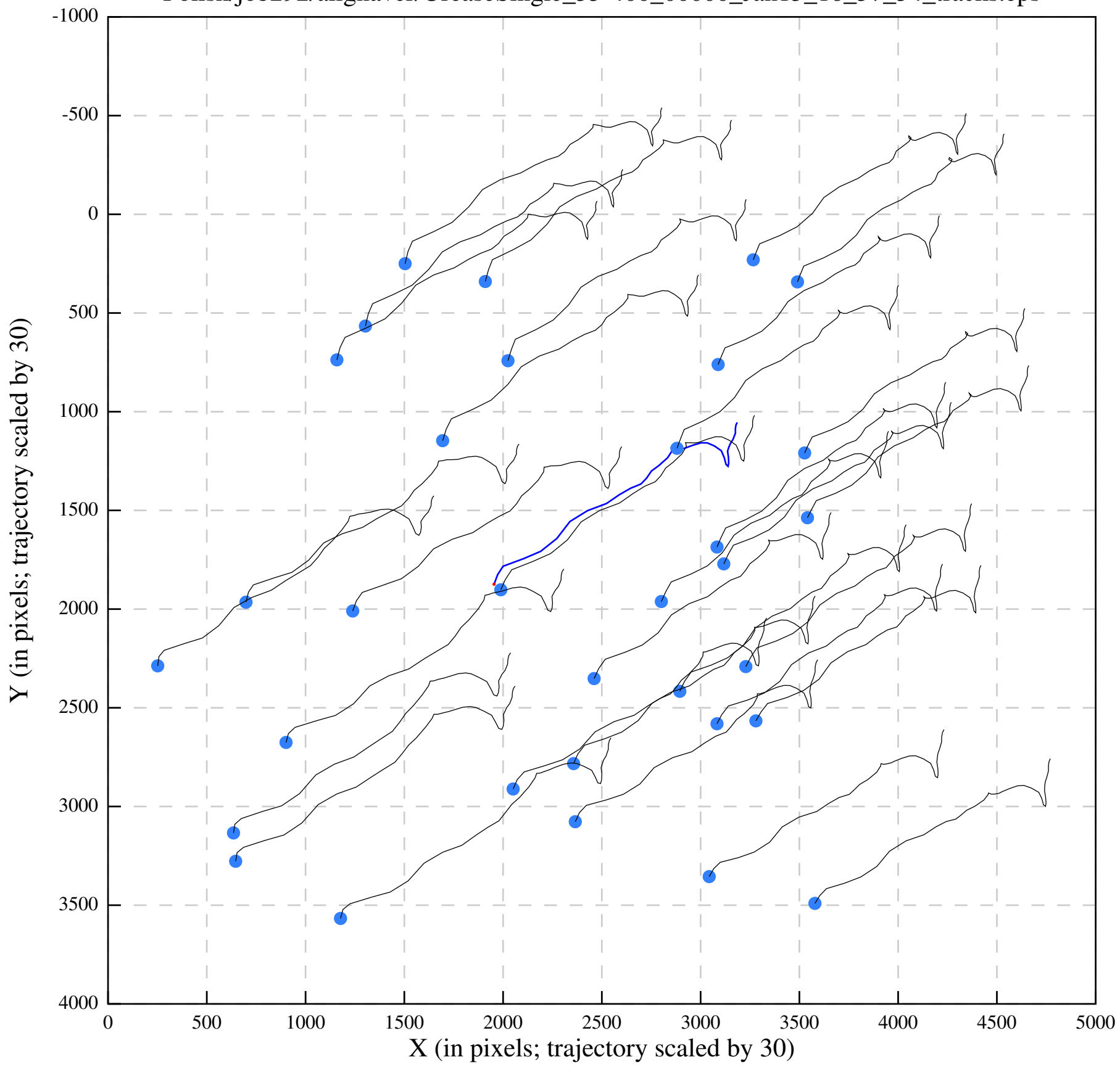
Polish/job292/alignaver/UreaseSingle_35-400_00000_Jan13_16_57_54_tracks.eps
