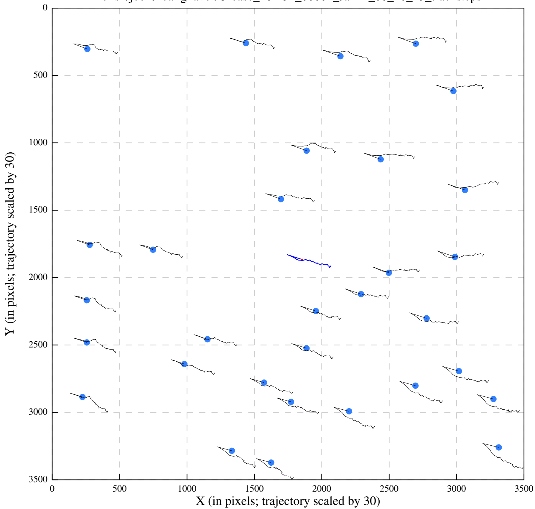
Polish/job292/alignaver/Urease_28-454_00001_Jan12_08_16_23_tracks.eps
