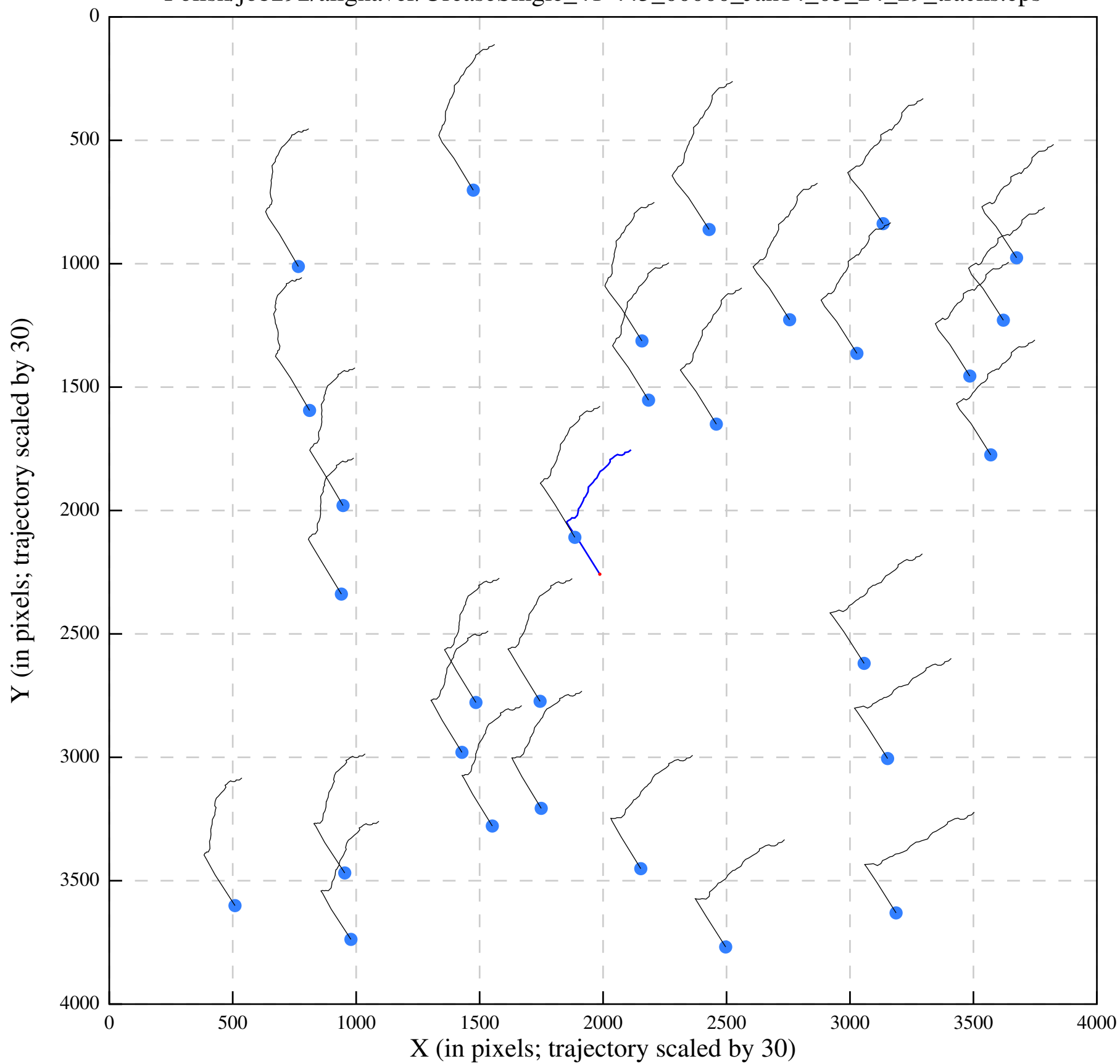
Polish/job292/alignaver/UreaseSingle_41-445_00000_Jan14_03_24_29_tracks.eps
