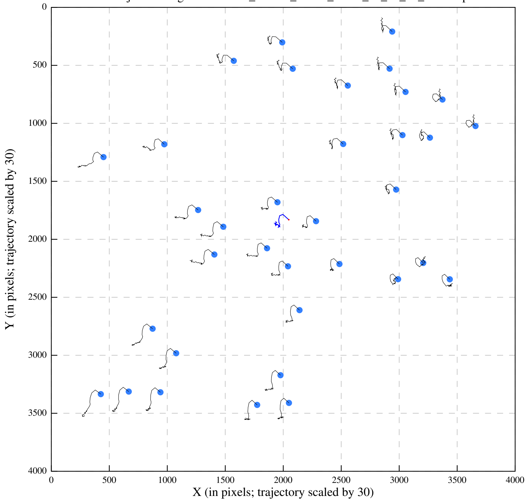
Polish/job292/alignaver/Urease_28-207_00002_Jan12_00_03_37_tracks.eps
