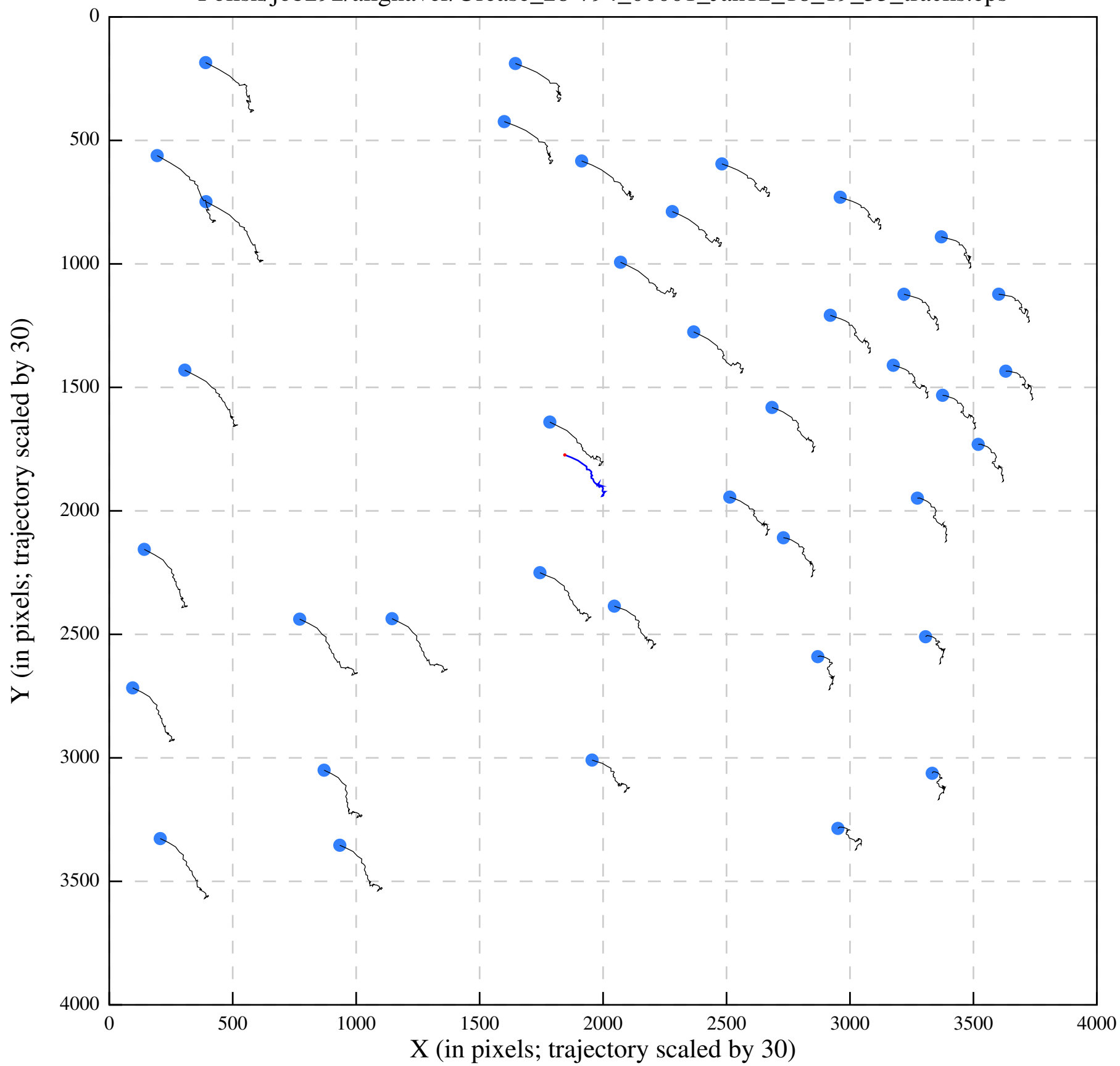
Polish/job292/alignaver/Urease_28-794_00001_Jan12_18_19_33_tracks.eps
