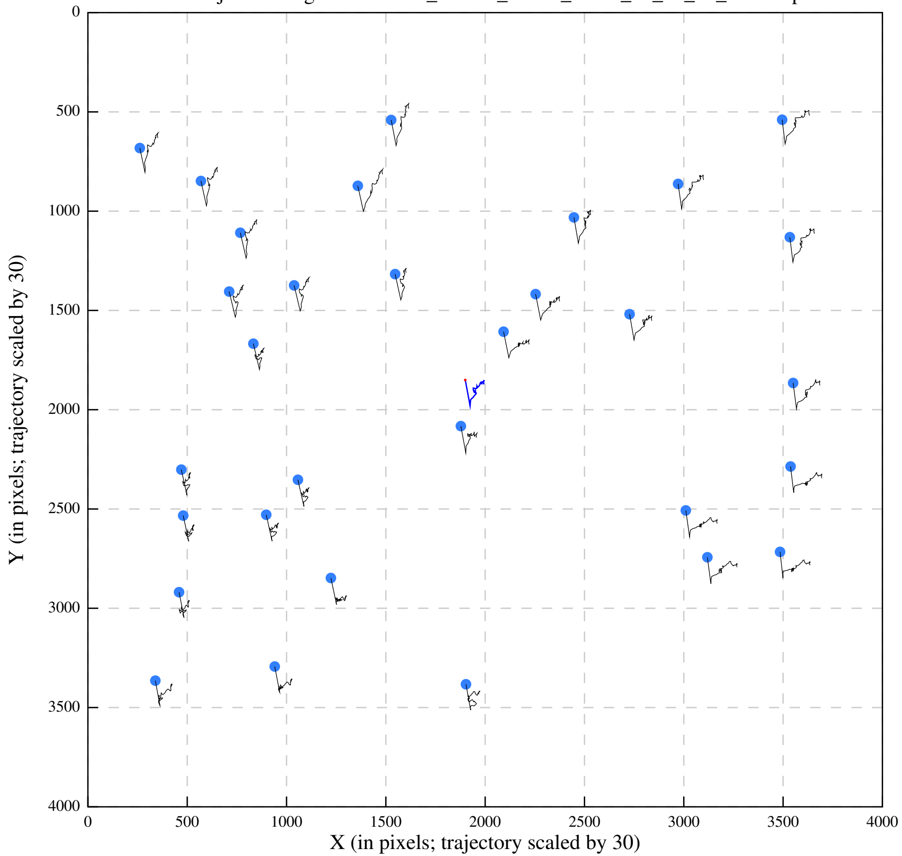
Polish/job292/alignaver/Urease_28-410_00000_Jan12_06_49_33_tracks.eps
