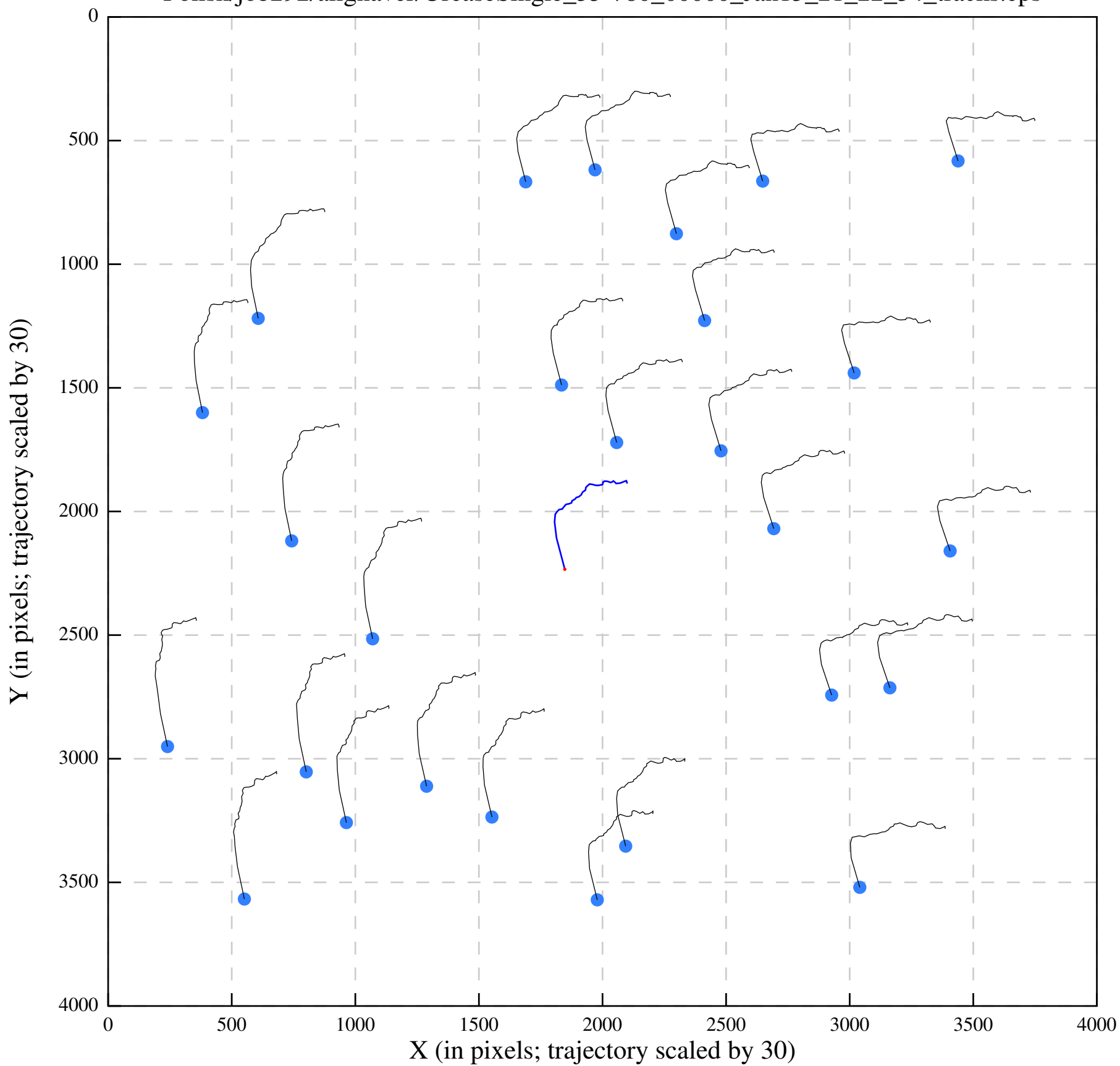
Polish/job292/alignaver/UreaseSingle_35-780_00000_Jan13_21_22_34_tracks.eps
