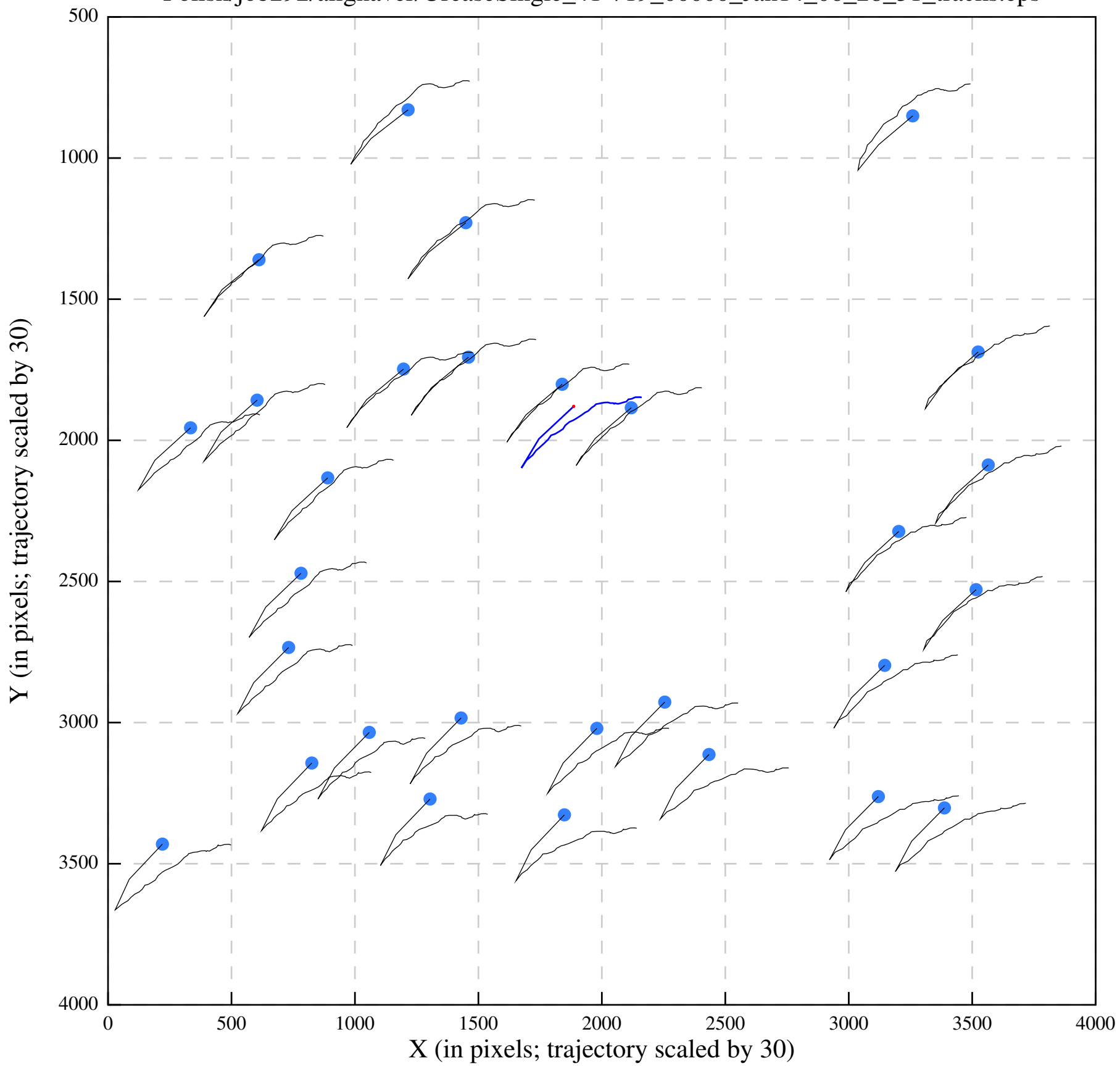
Polish/job292/alignaver/UreaseSingle_41-719_00000_Jan14_06_28_31_tracks.eps
