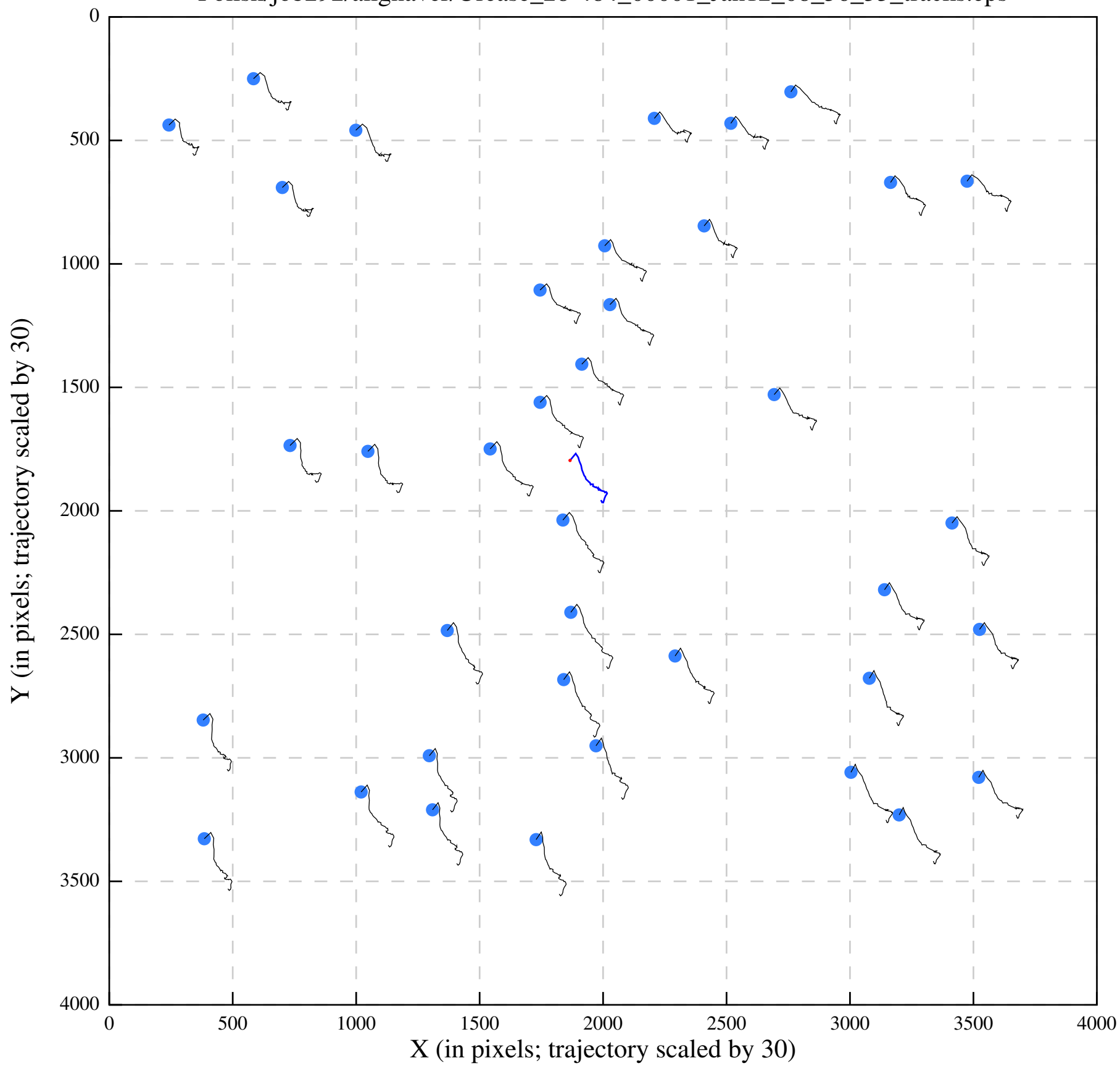
Polish/job292/alignaver/Urease_28-484_00001_Jan12_08_56_33_tracks.eps
