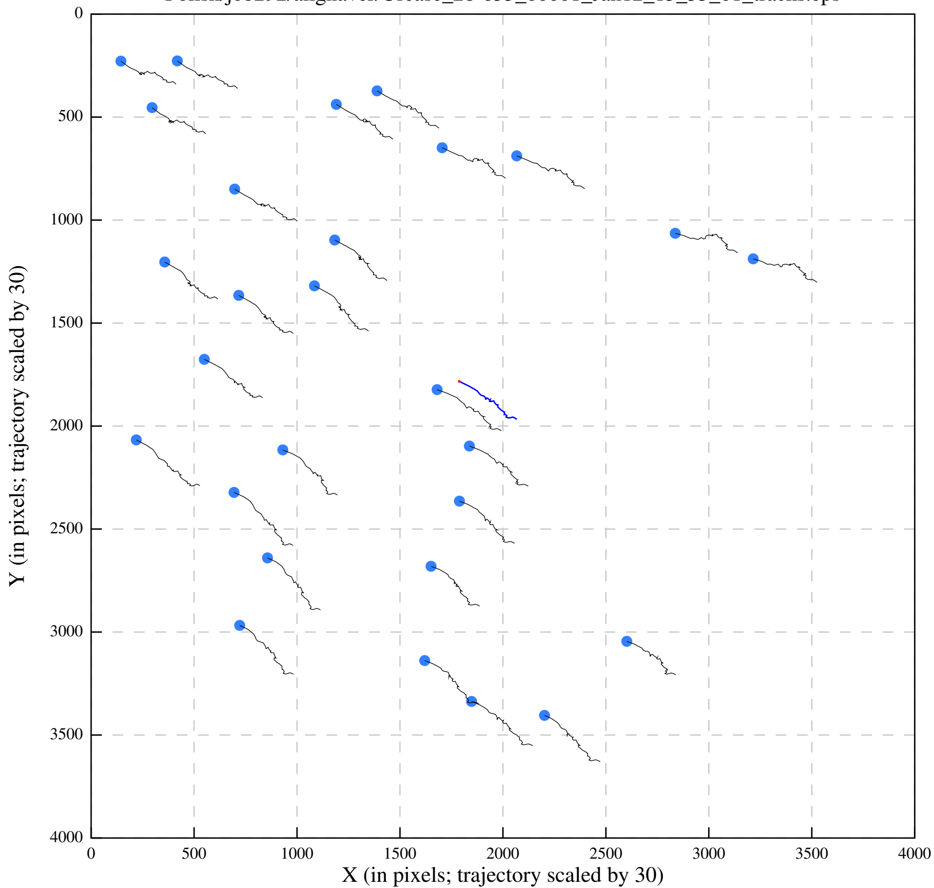
Polish/job292/alignaver/Urease_28-633_00001_Jan12_13_35_01_tracks.eps
