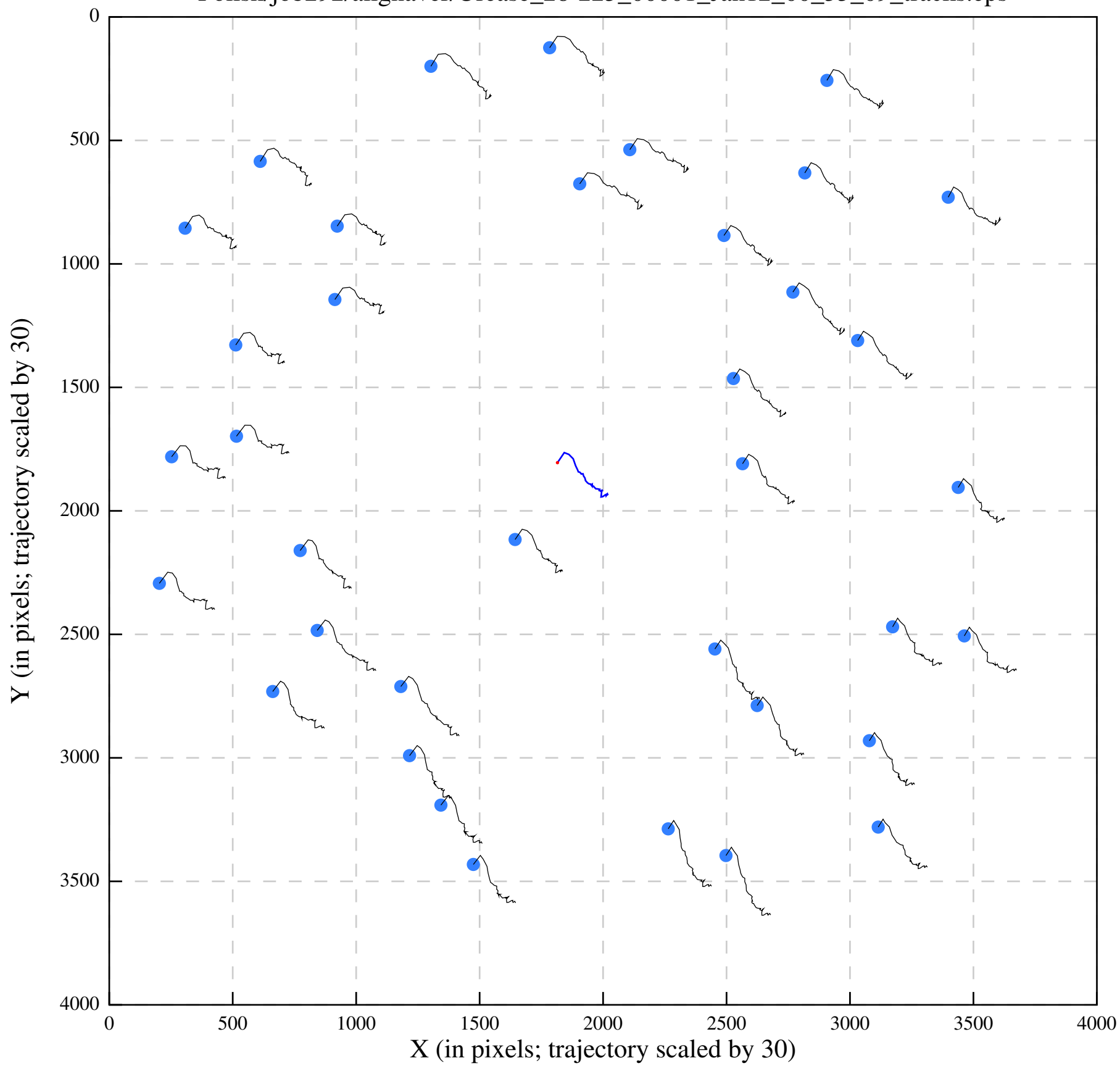
Polish/job292/alignaver/Urease_28-225_00001_Jan12_00_35_09_tracks.eps
