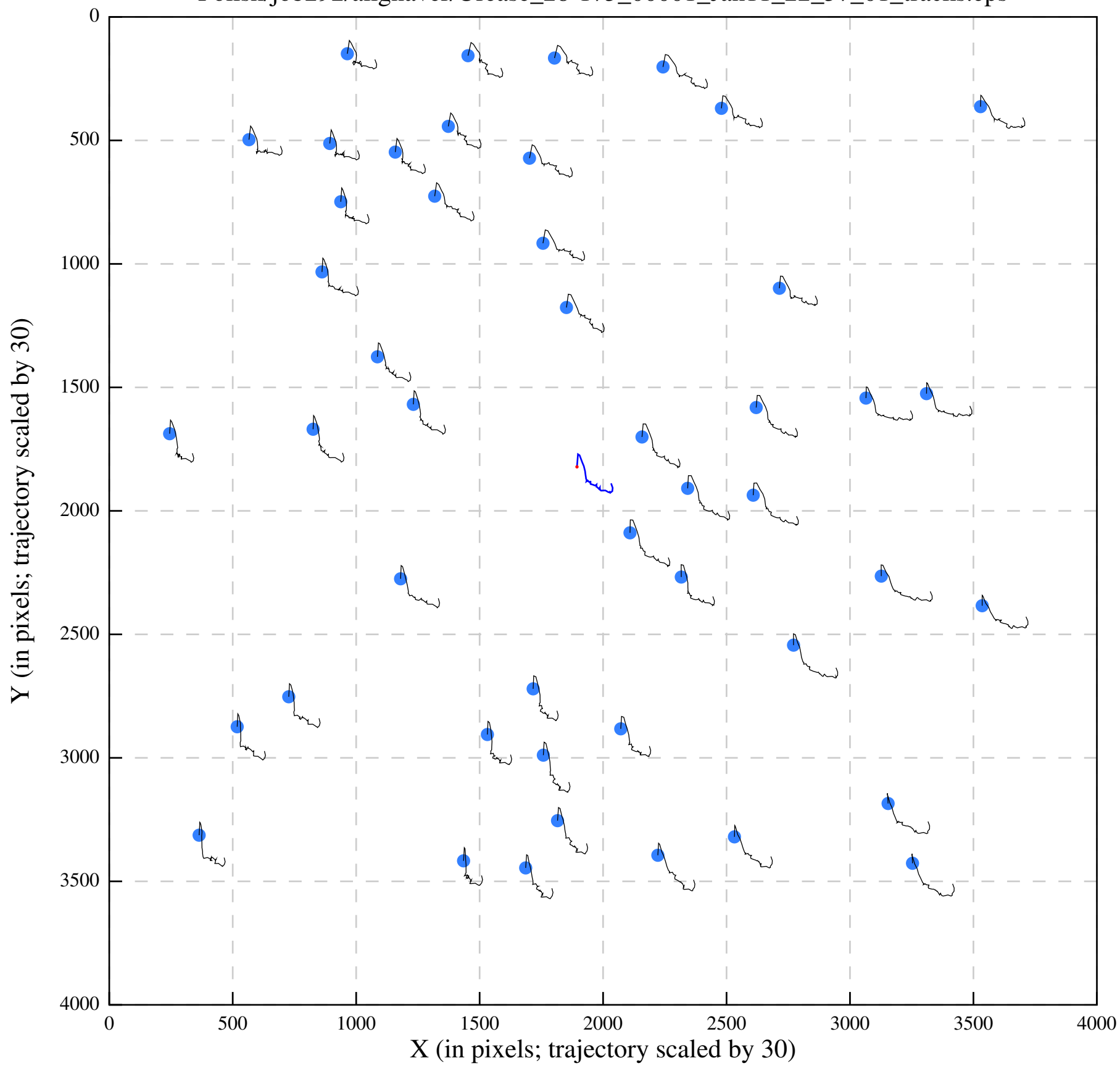
Polish/job292/alignaver/Urease_28-175_00001_Jan11_22_57_01_tracks.eps
