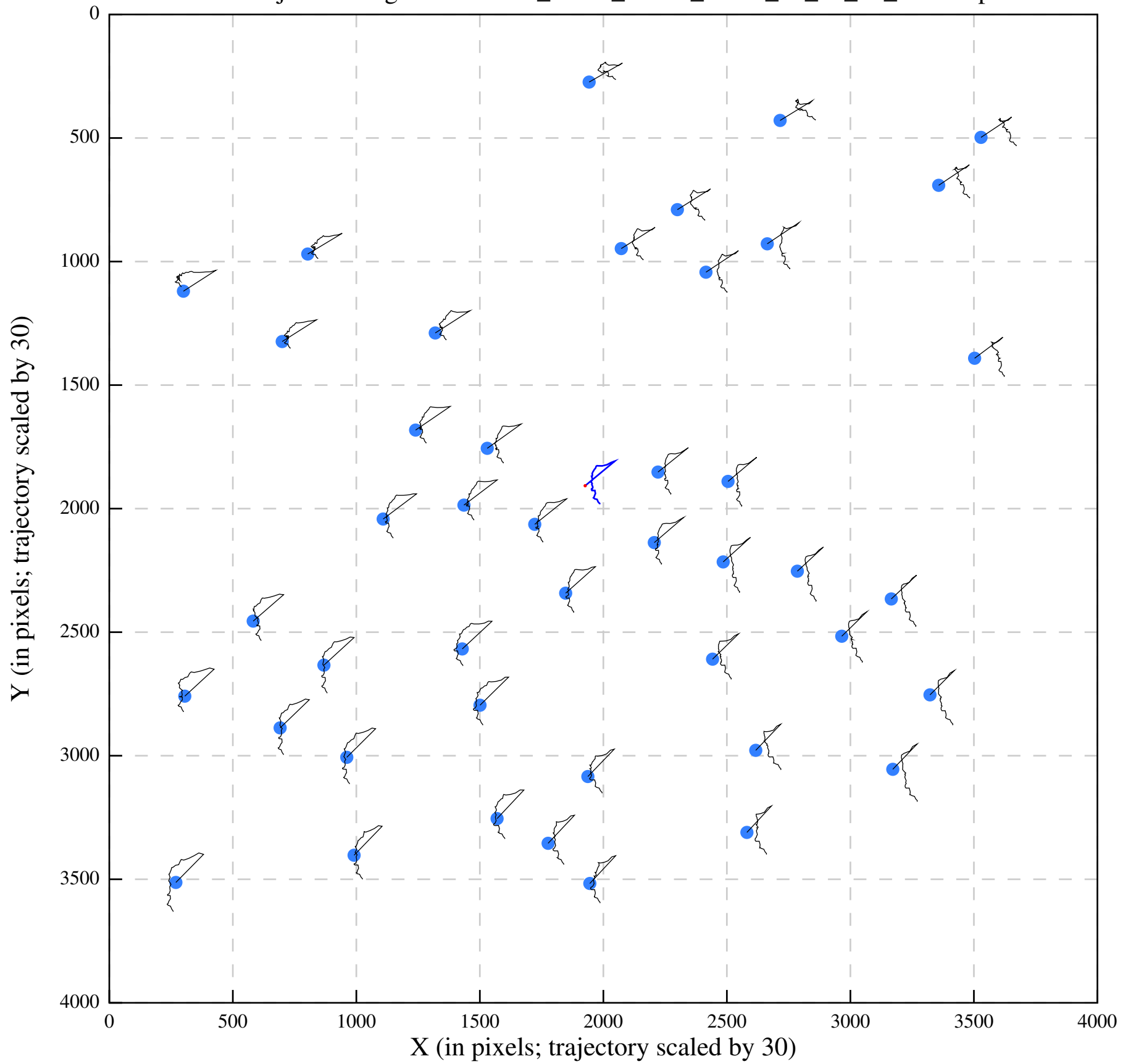
Polish/job292/alignaver/Urease_28-60_00002_Jan11_19_13_11_tracks.eps
