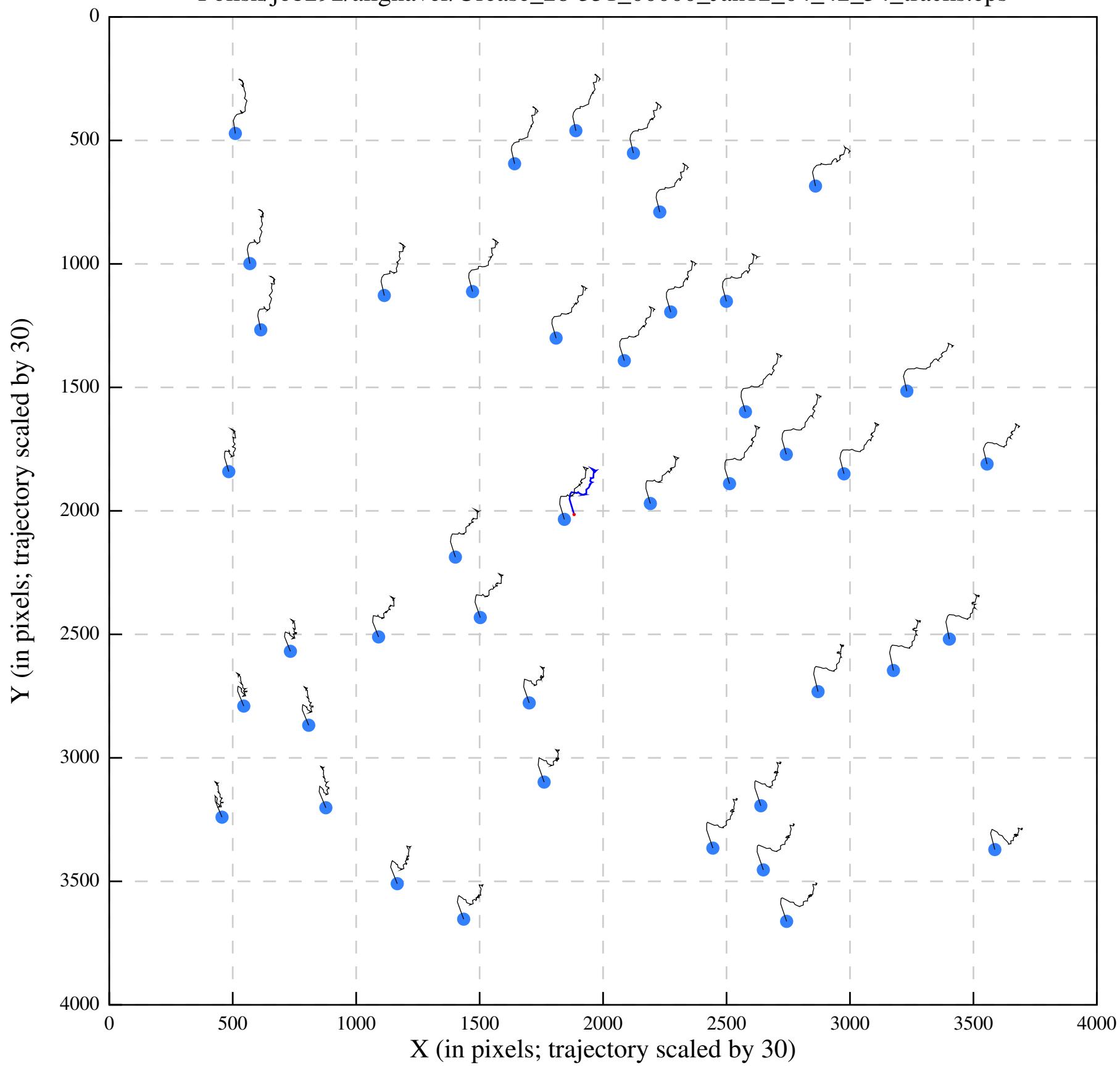
Polish/job292/alignaver/Urease_28-351_00000_Jan12_04_42_54_tracks.eps
