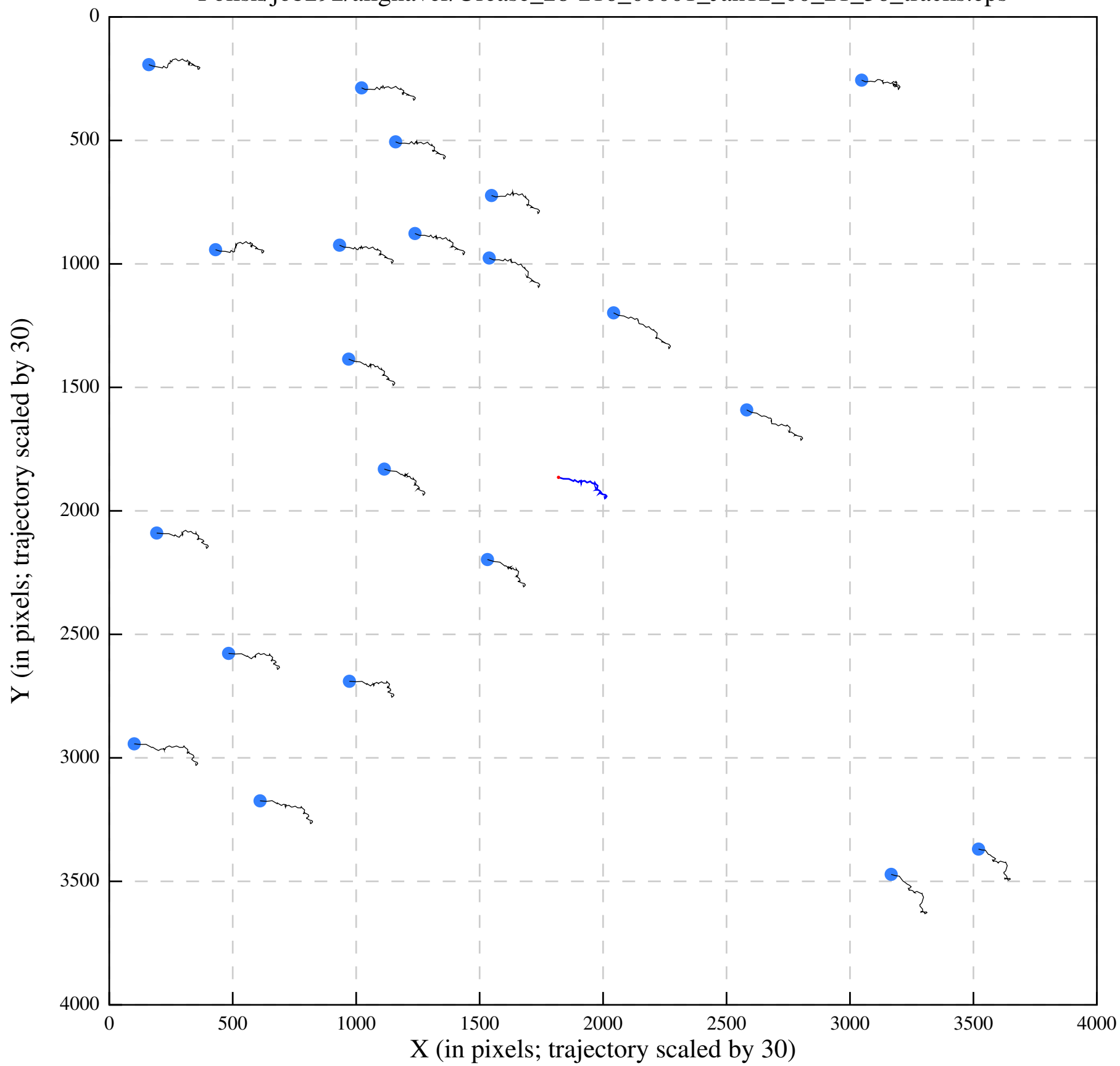
Polish/job292/alignaver/Urease_28-216_00001_Jan12_00_21_36_tracks.eps
