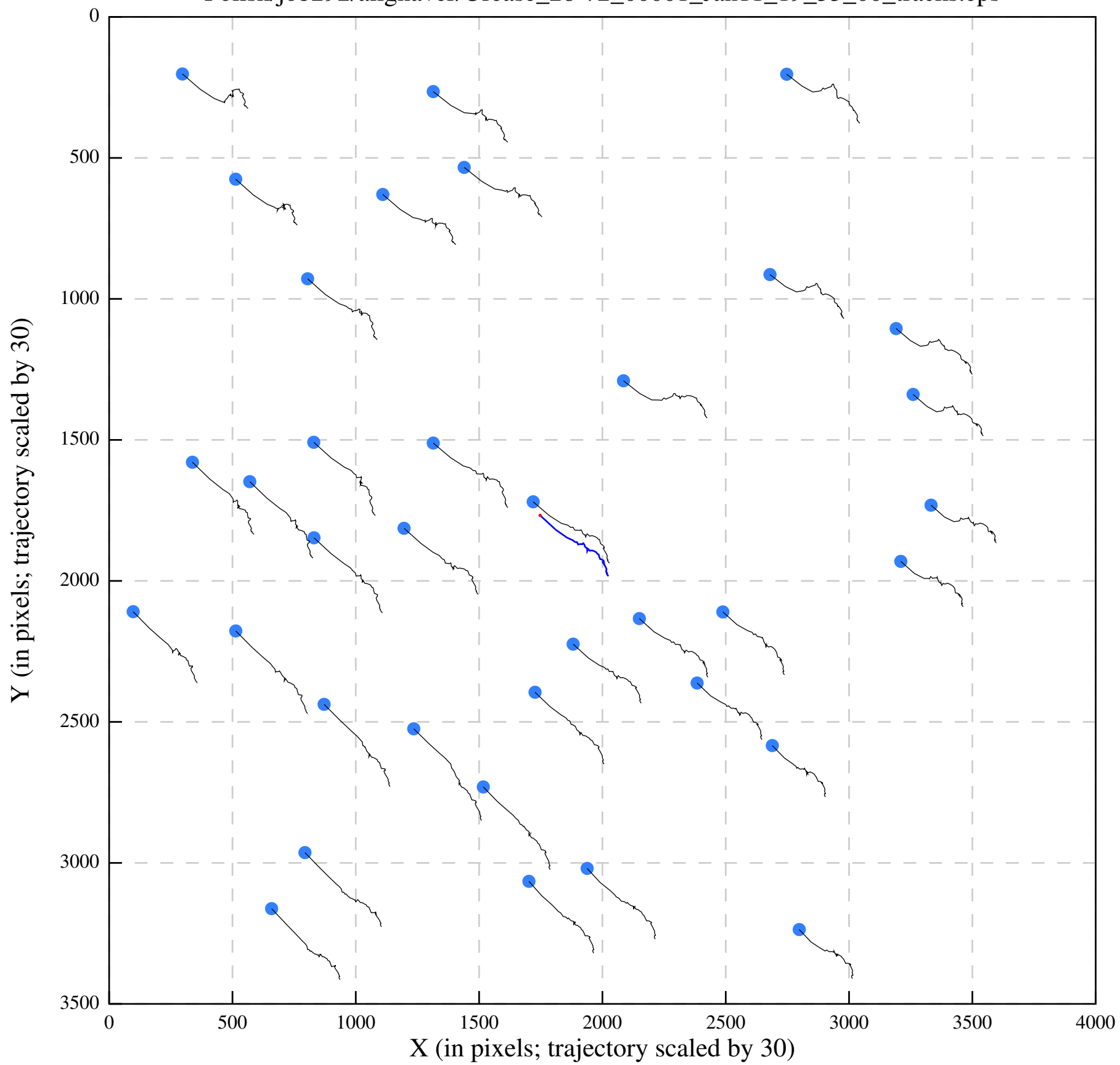
Polish/job292/alignaver/Urease_28-72_00001_Jan11_19_33_00_tracks.eps
