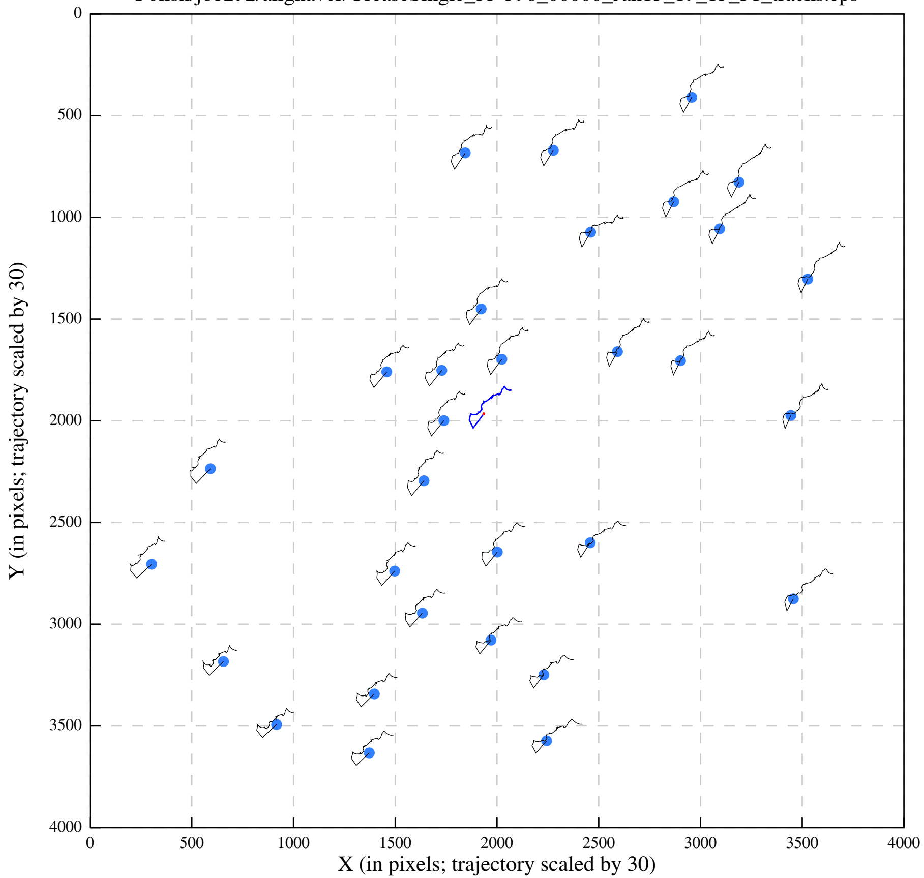
Polish/job292/alignaver/UreaseSingle_35-598_00000_Jan13_19_15_51_tracks.eps
