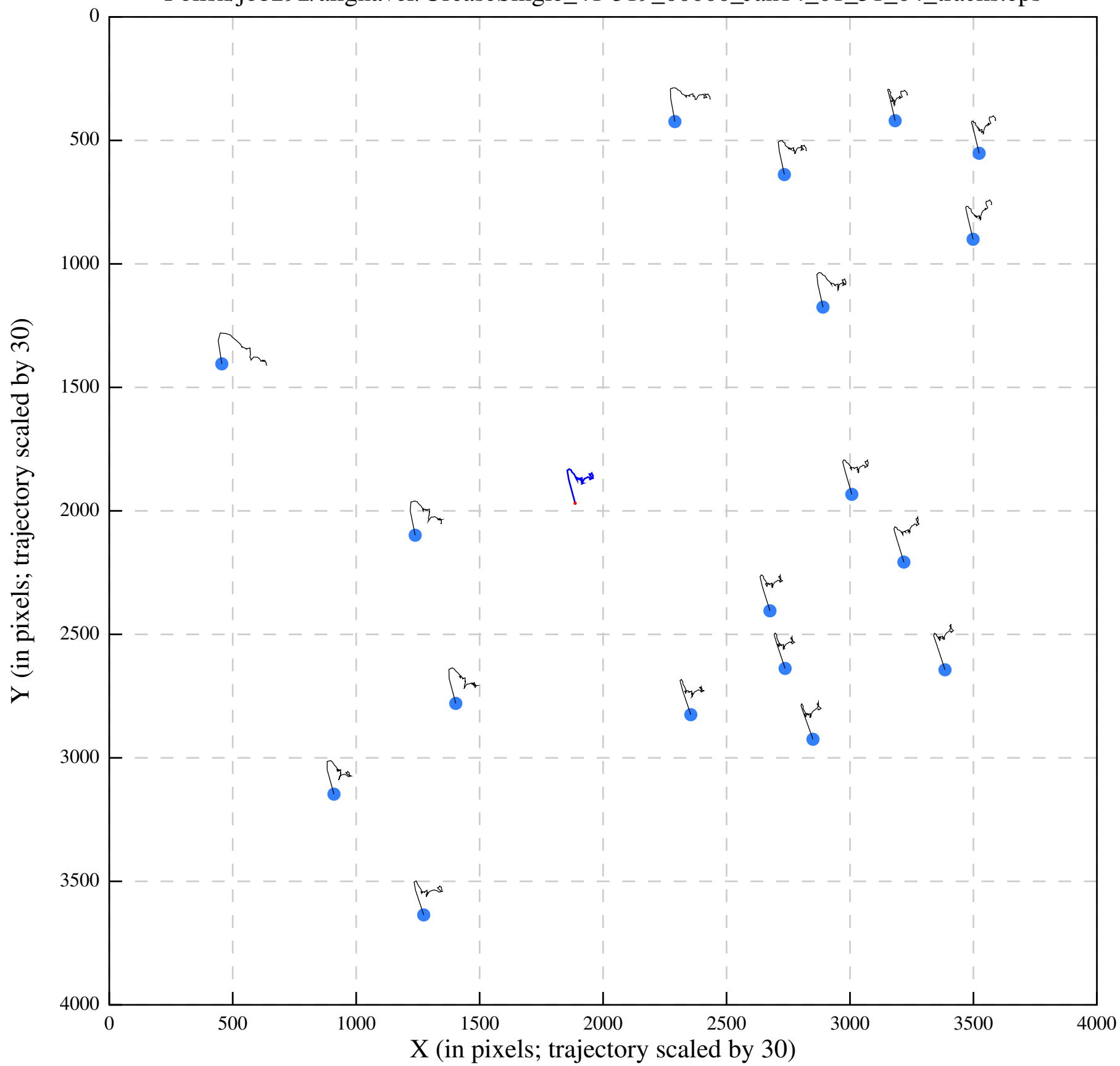
Polish/job292/alignaver/UreaseSingle_41-319_00000_Jan14_01_51_04_tracks.eps
