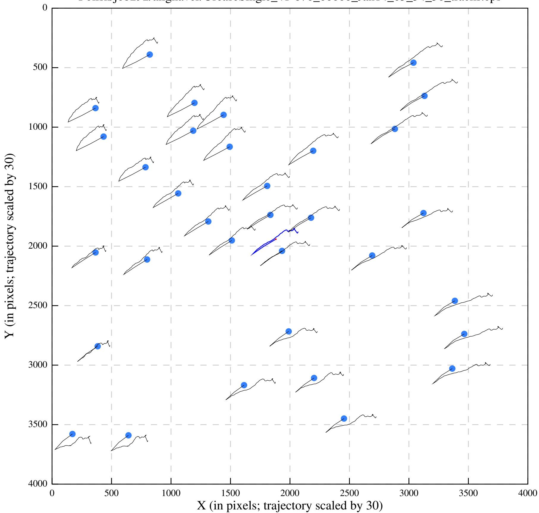
Polish/job292/alignaver/UreaseSingle_41-670_00000_Jan14_05_54_50_tracks.eps
