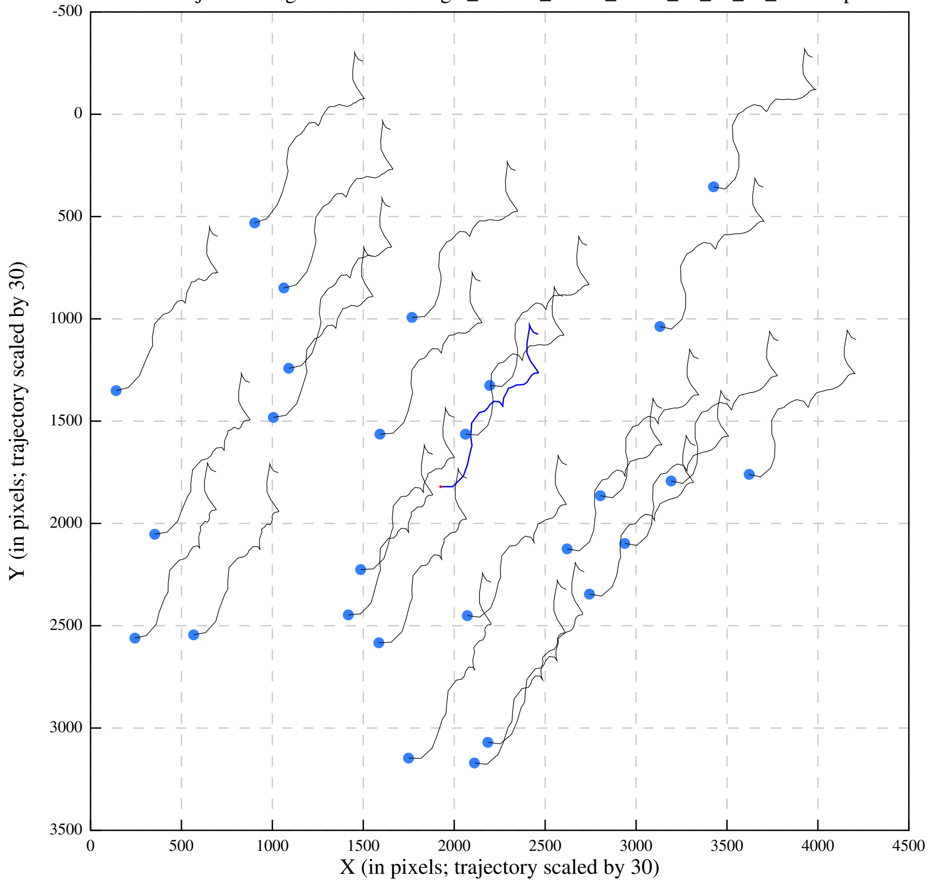
Polish/job292/alignaver/UreaseSingle_35-693_00000_Jan13_20_16_28_tracks.eps
