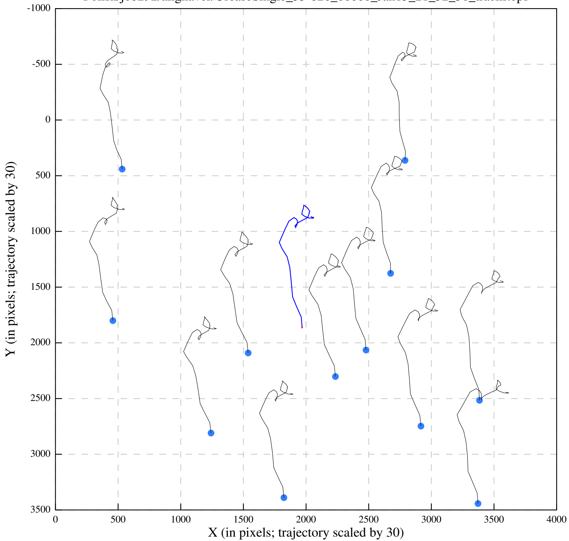
Polish/job292/alignaver/UreaseSingle_35-826_00000_Jan13_21_52_30_tracks.eps
