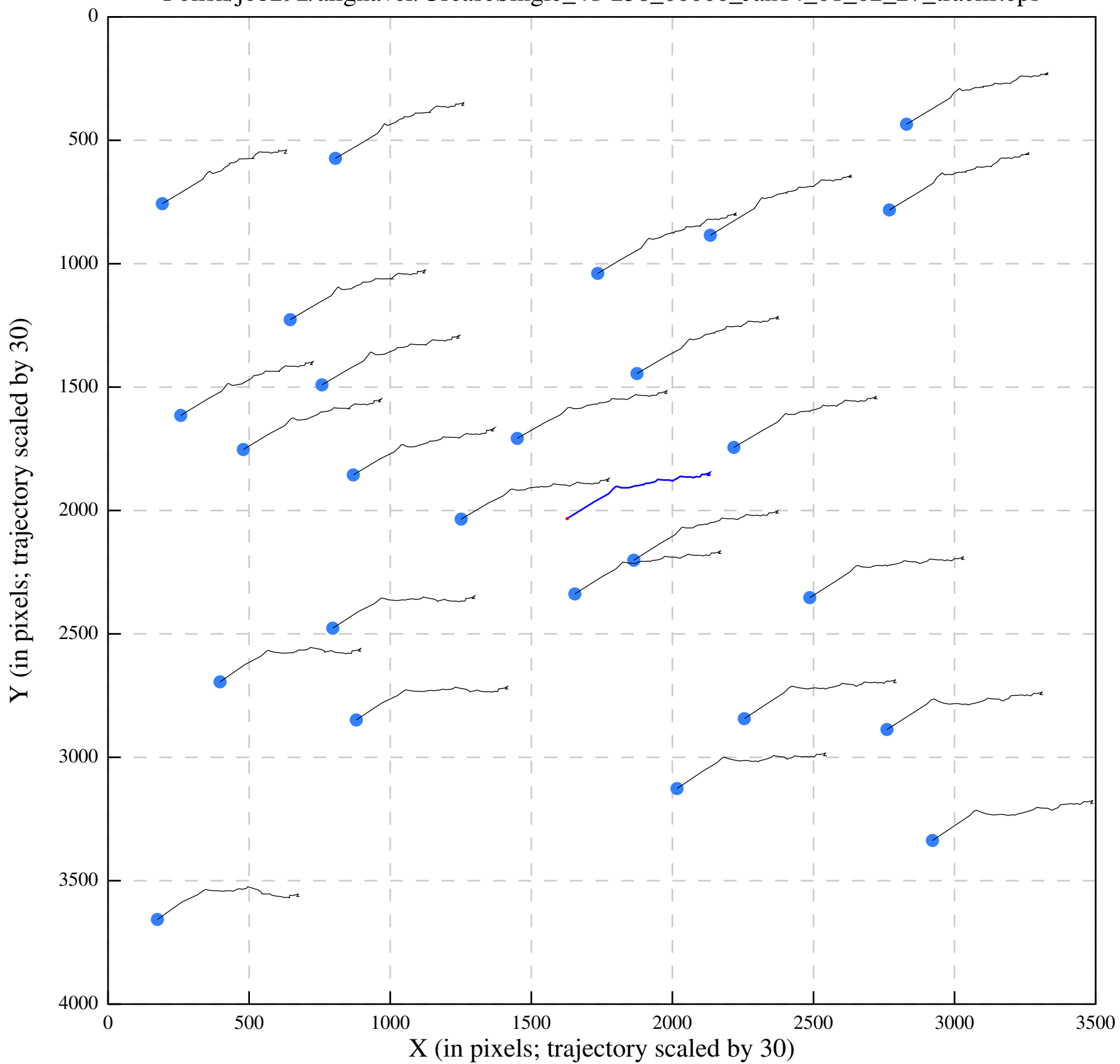
Polish/job292/alignaver/UreaseSingle_41-238_00000_Jan14_01_02_27_tracks.eps
