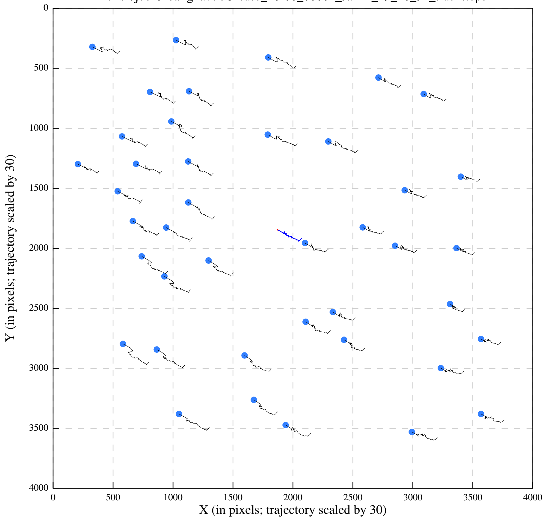
Polish/job292/alignaver/Urease_28-66_00001_Jan11_19_16_51_tracks.eps
