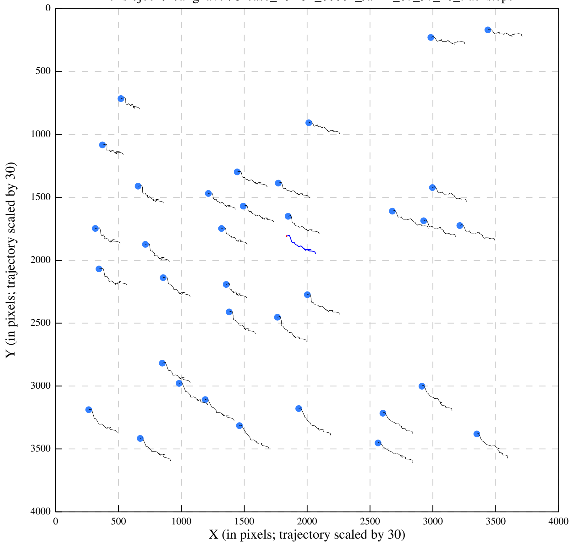
Polish/job292/alignaver/Urease_28-434_00001_Jan12_07_37_40_tracks.eps
