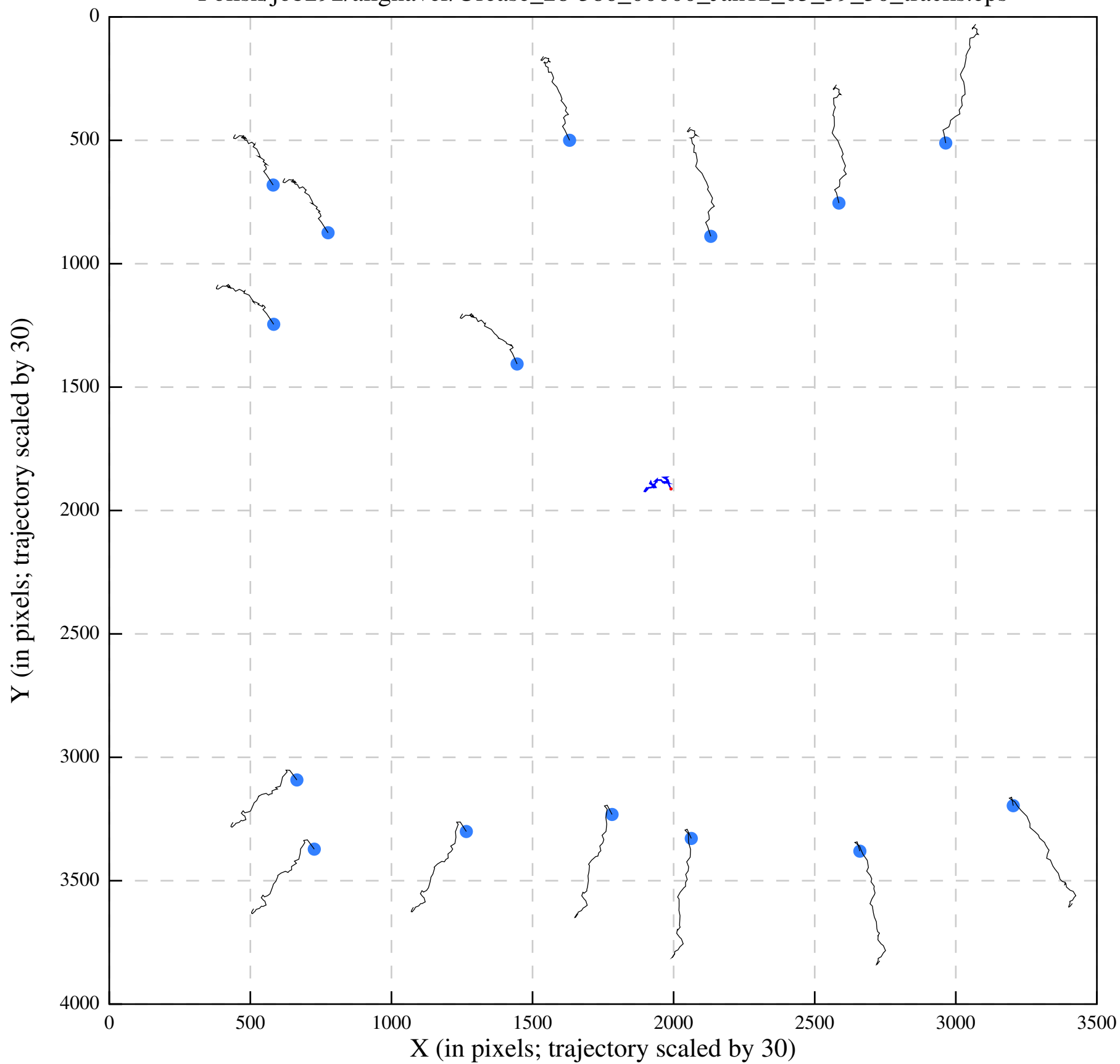
Polish/job292/alignaver/Urease_28-386_00000_Jan12_05_59_30_tracks.eps
