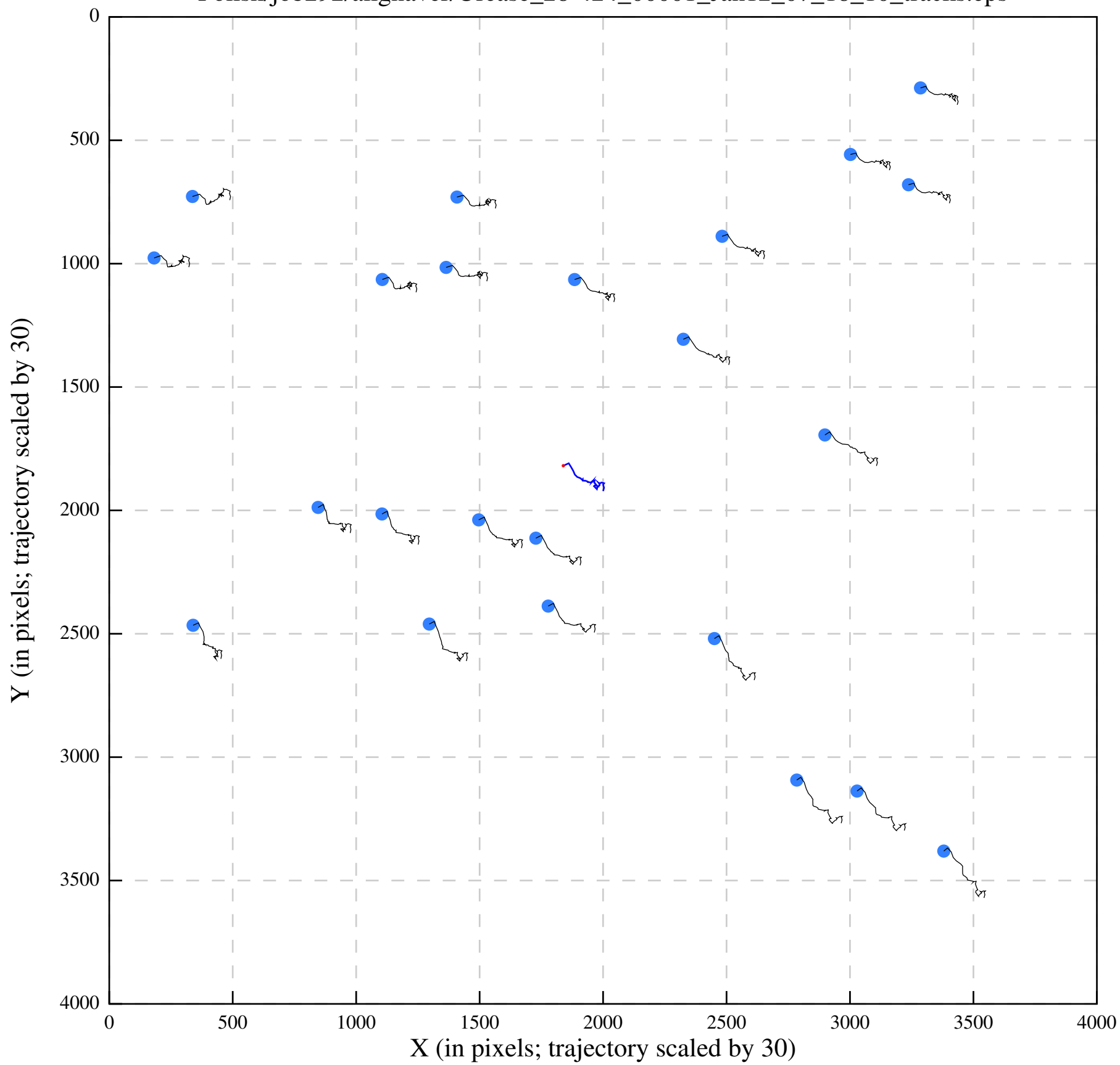
Polish/job292/alignaver/Urease_28-424_00001_Jan12_07_18_10_tracks.eps
