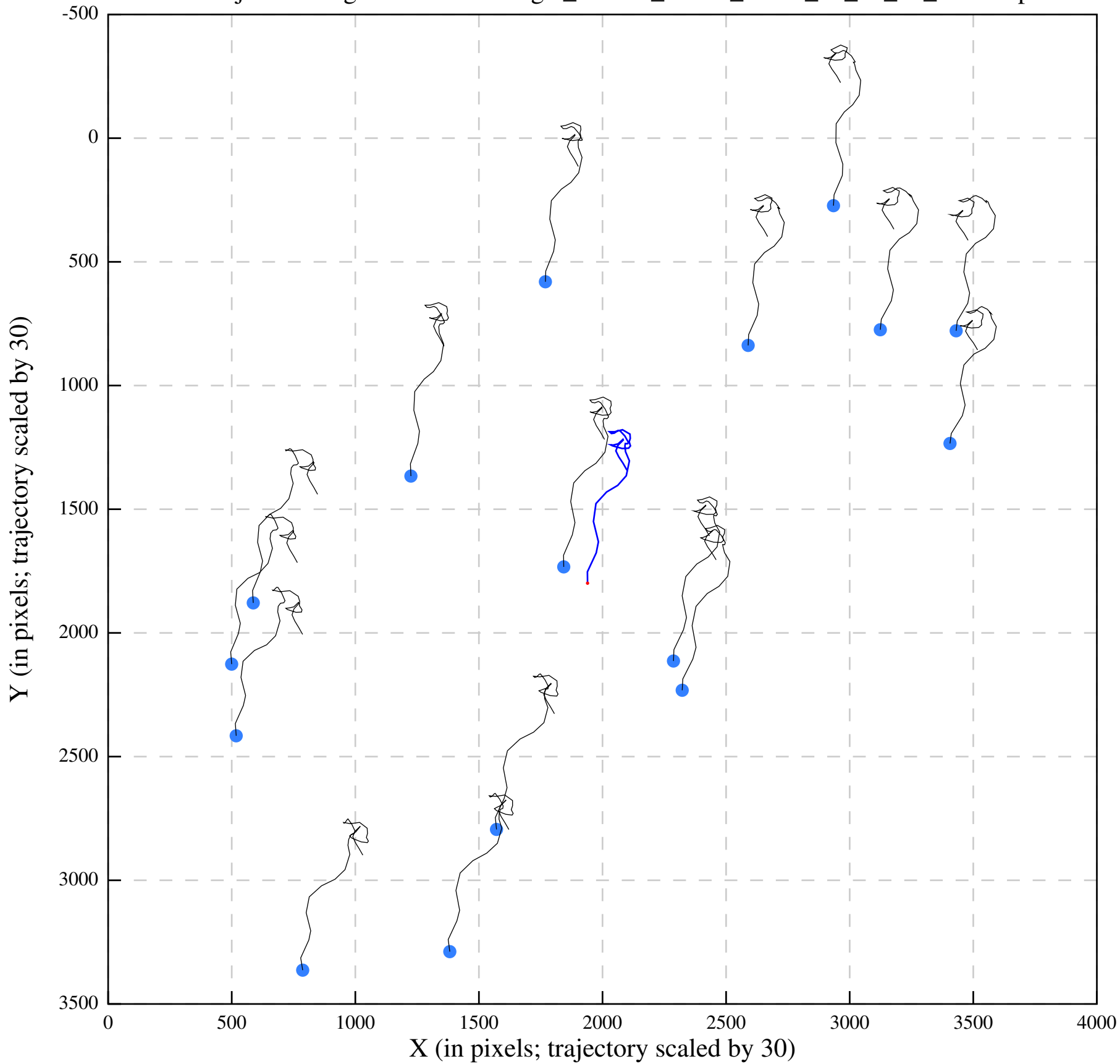
Polish/job292/alignaver/UreaseSingle_47-739_00000_Jan14_16_23_18_tracks.eps
