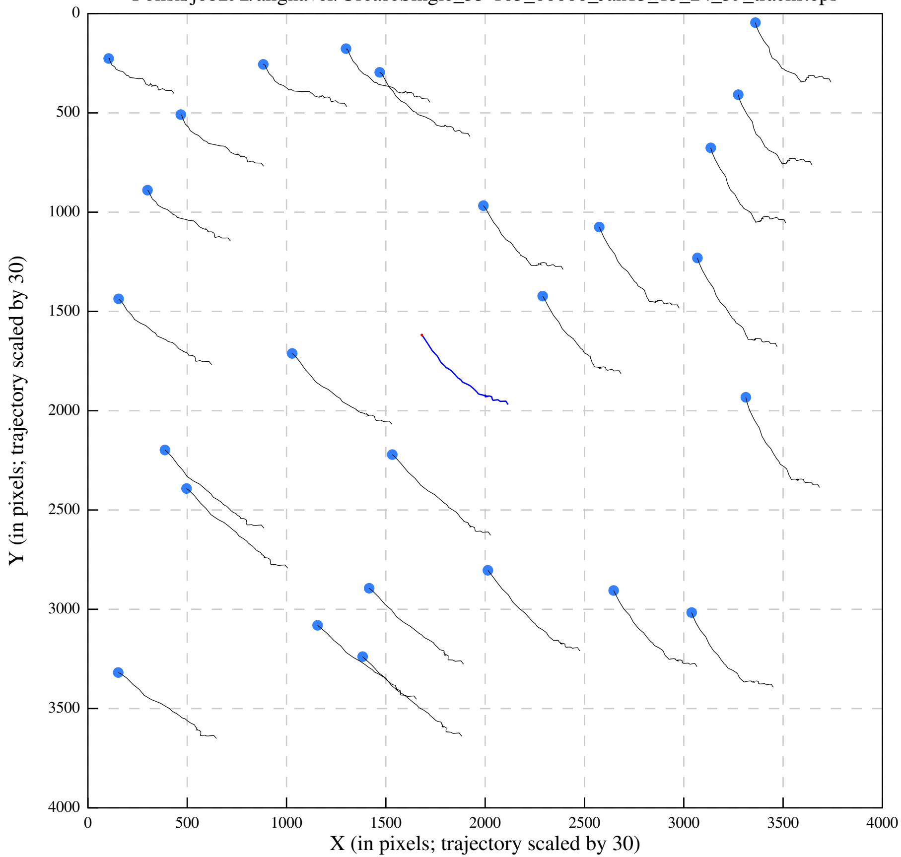
Polish/job292/alignaver/UreaseSingle_35-103_00000_Jan13_13_24_39_tracks.eps
