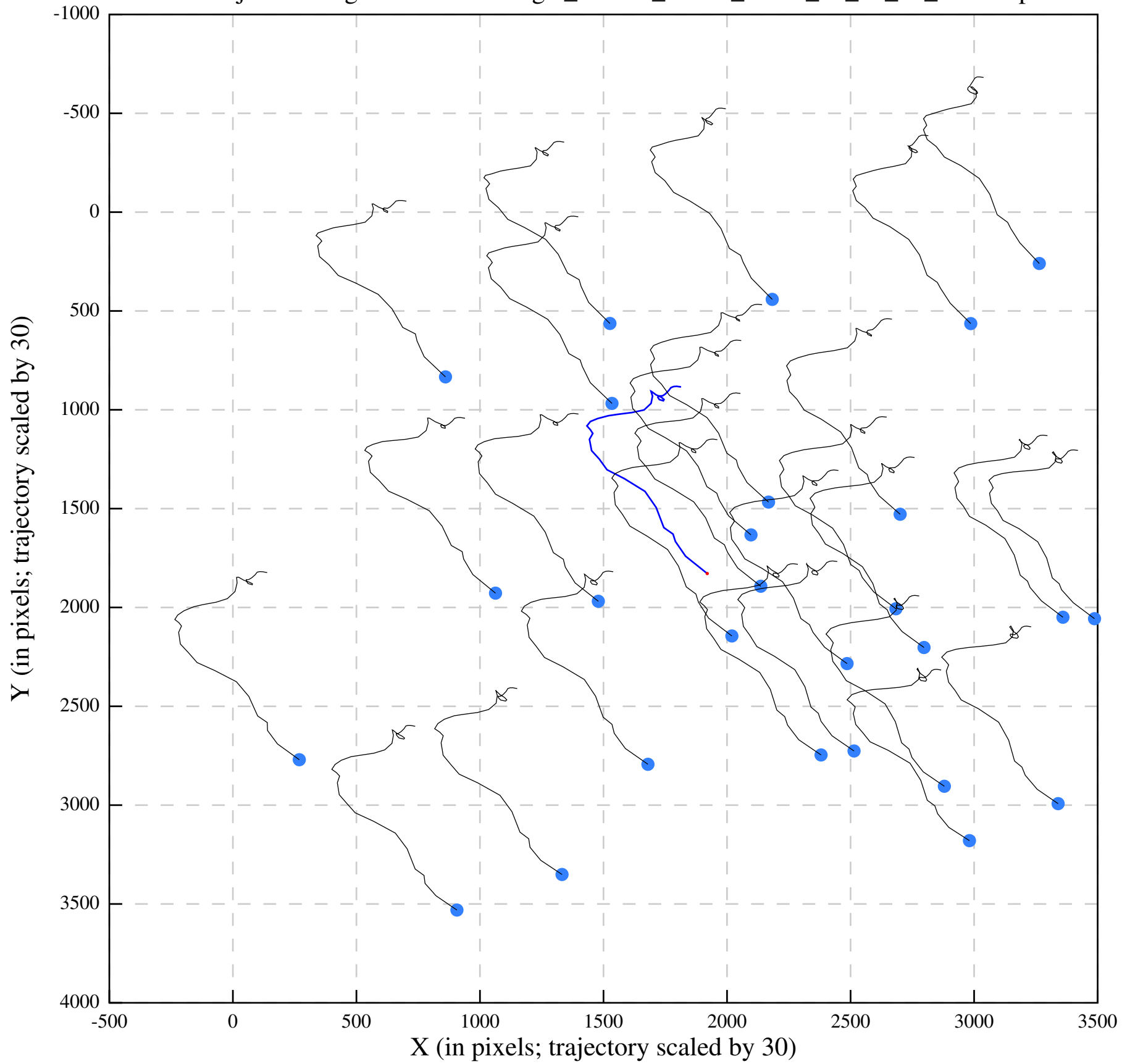
Polish/job292/alignaver/UreaseSingle_47-634_00000_Jan14_15_17_09_tracks.eps
