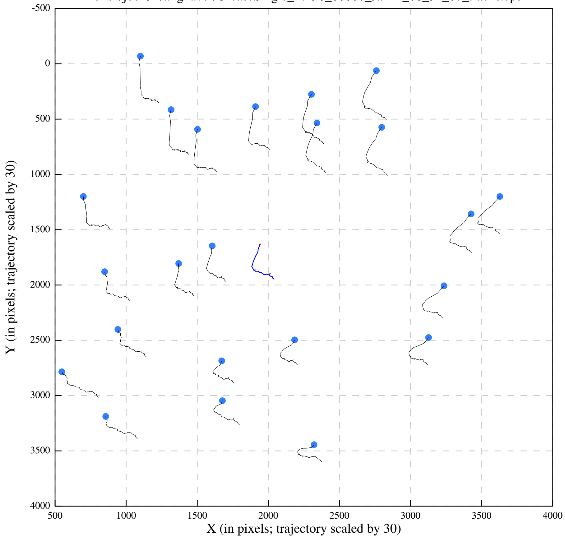
Polish/job292/alignaver/UreaseSingle_47-98_00000_Jan14_08_51_07_tracks.eps
