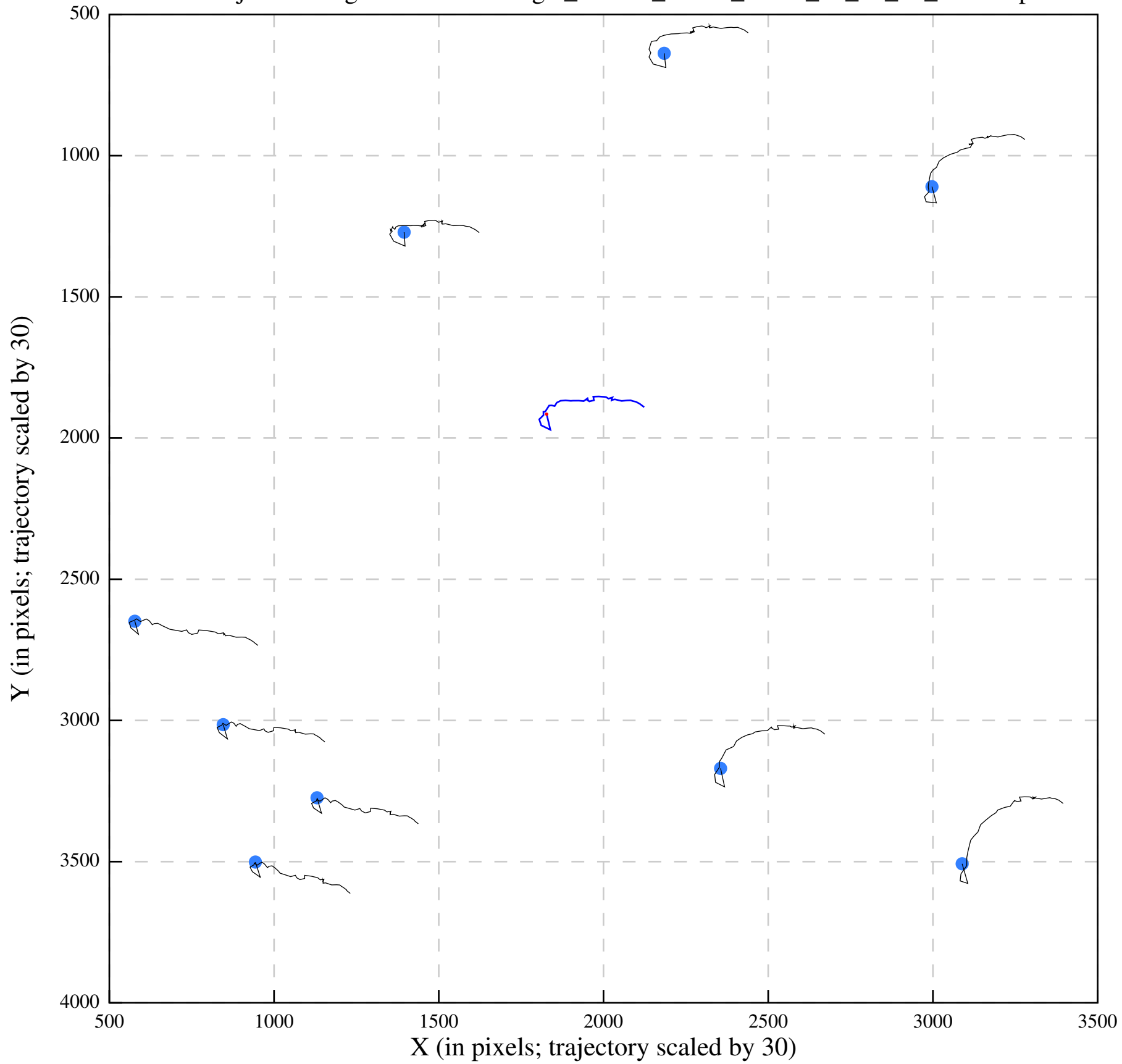
Polish/job292/alignaver/UreaseSingle_47-729_00000_Jan14_16_19_10_tracks.eps
