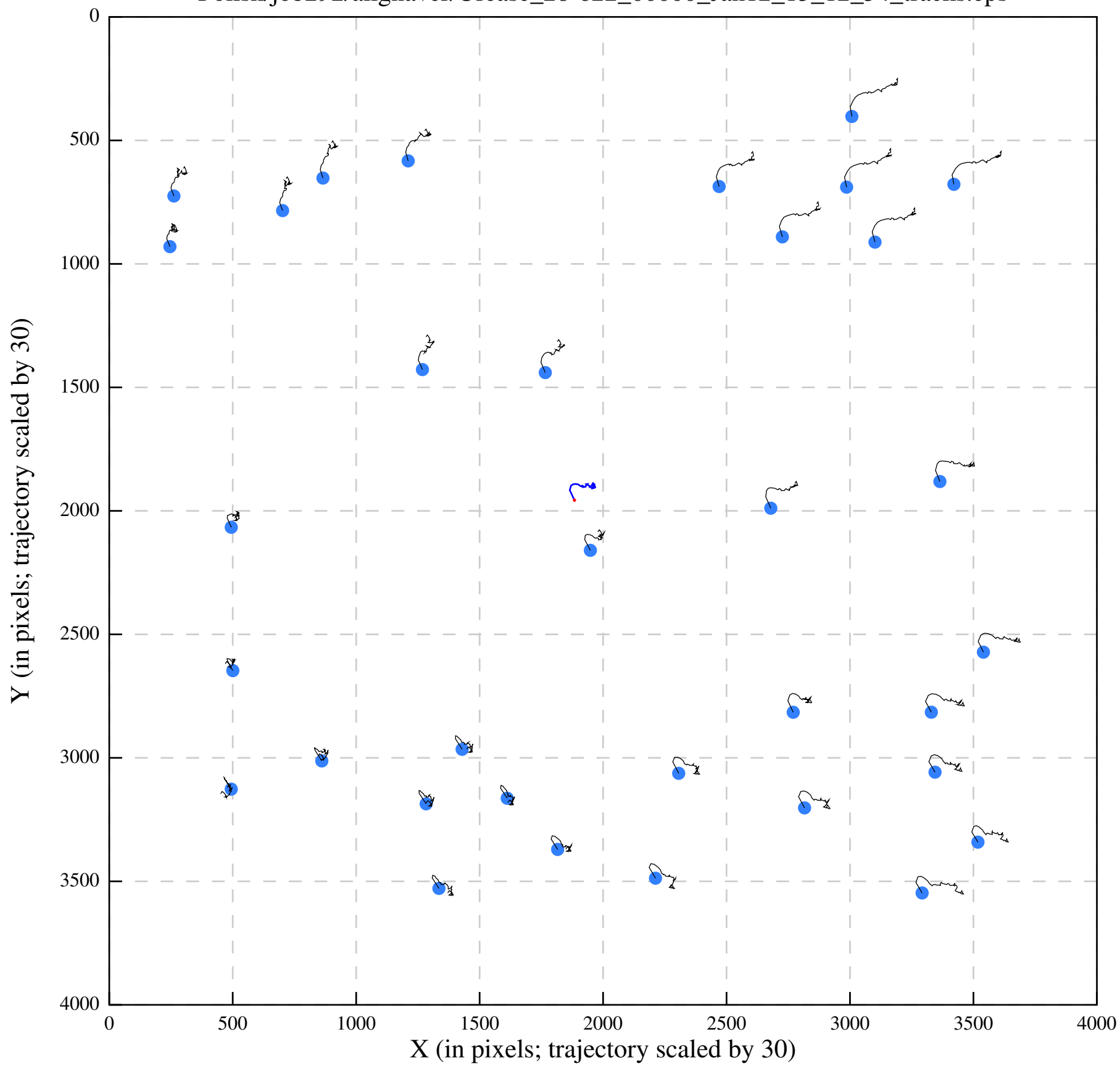
Polish/job292/alignaver/Urease_28-622_00000_Jan12_13_12_54_tracks.eps
