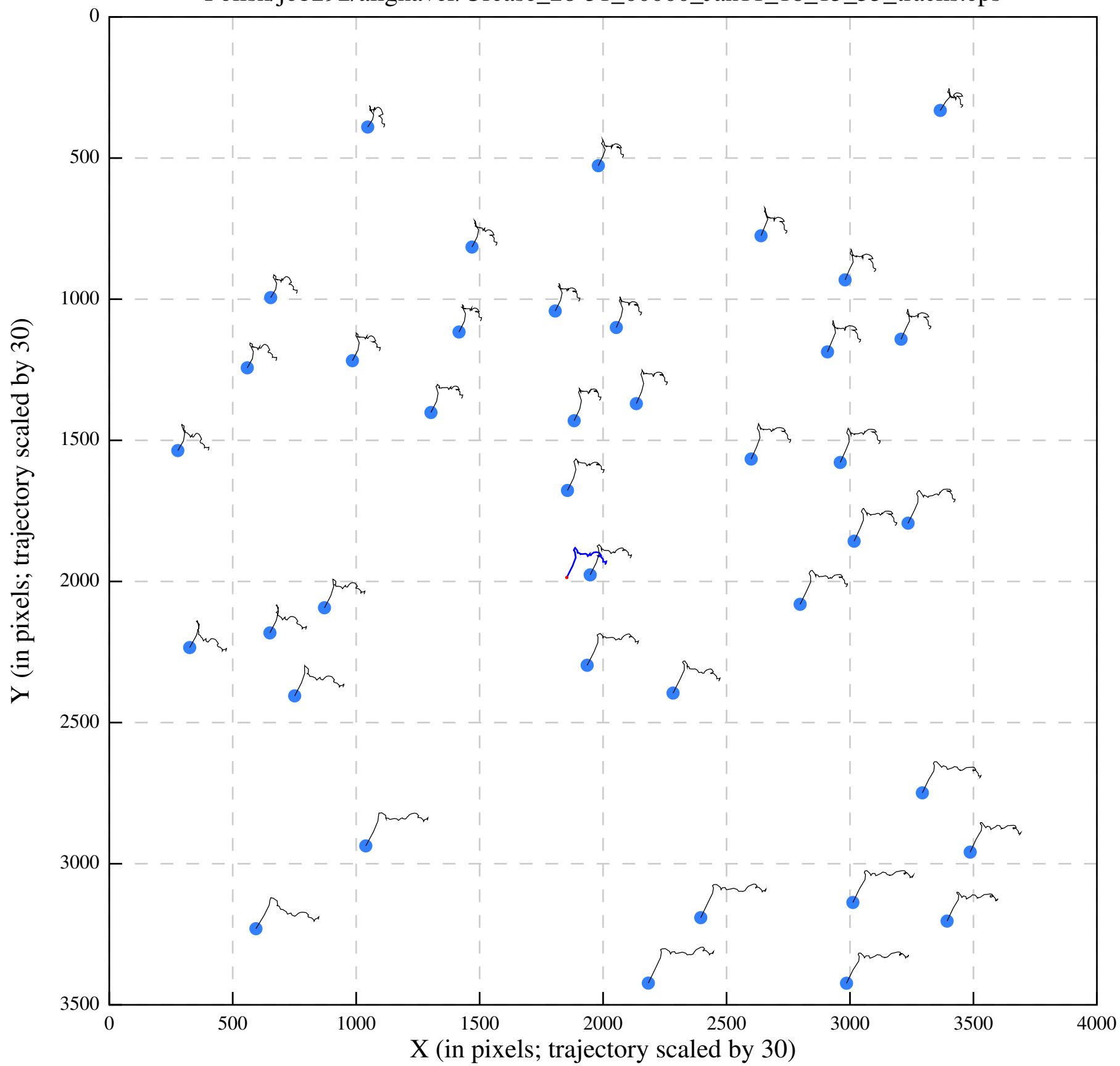
Polish/job292/alignaver/Urease_28-31_00000_Jan11_18_15_55_tracks.eps
