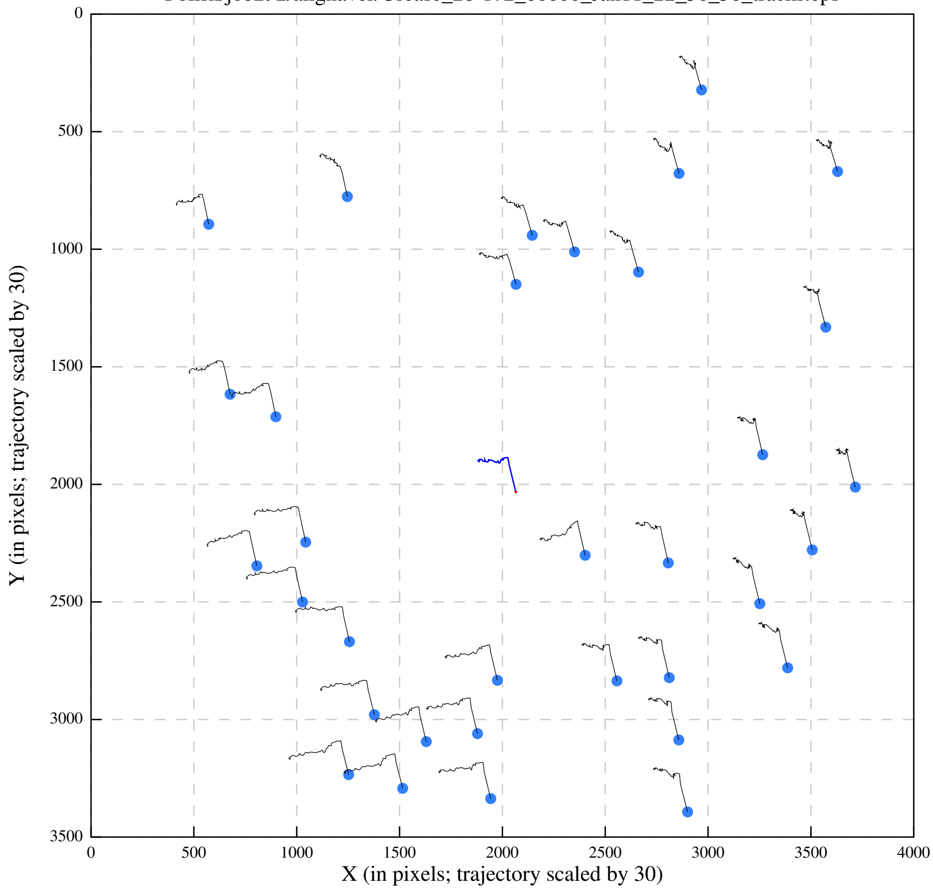
Polish/job292/alignaver/Urease_28-172_00000_Jan11_22_50_50_tracks.eps
