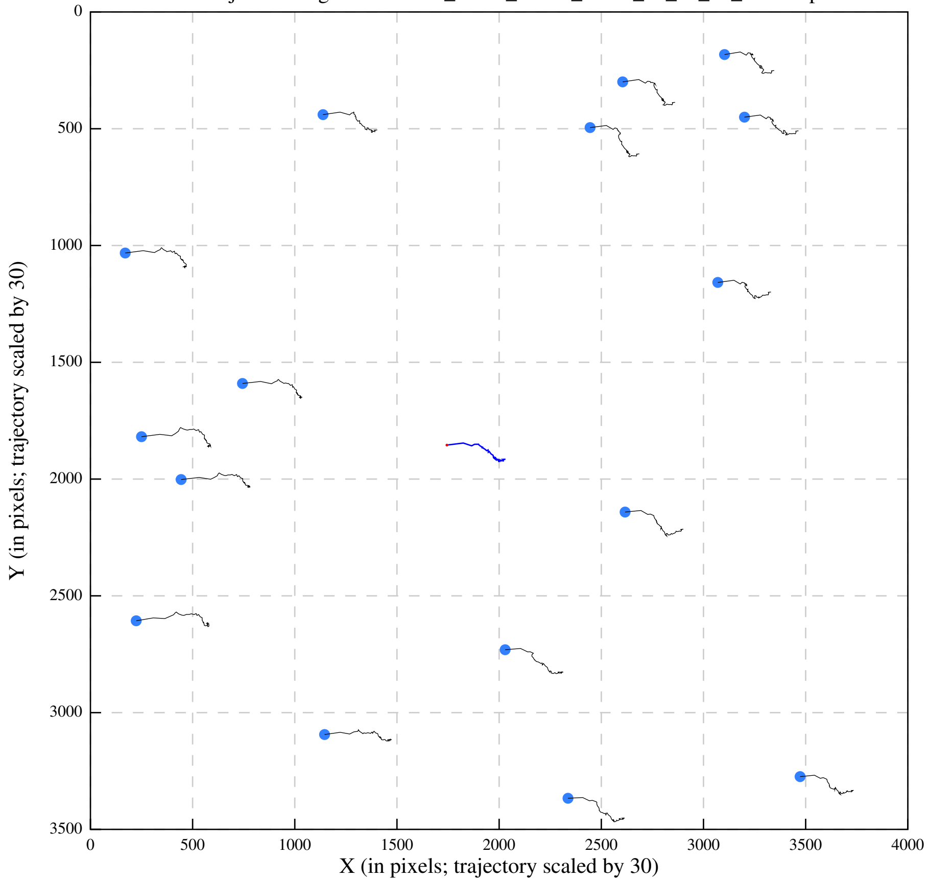
Polish/job292/alignaver/Urease_28-13_00001_Jan11_17_56_39_tracks.eps
