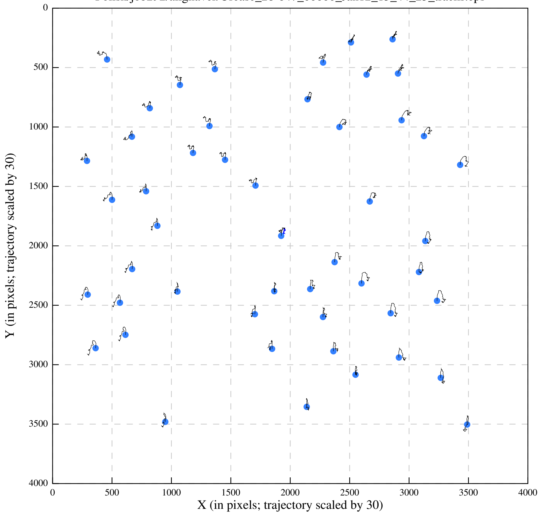
Polish/job292/alignaver/Urease_28-647_00000_Jan12_13_44_25_tracks.eps
