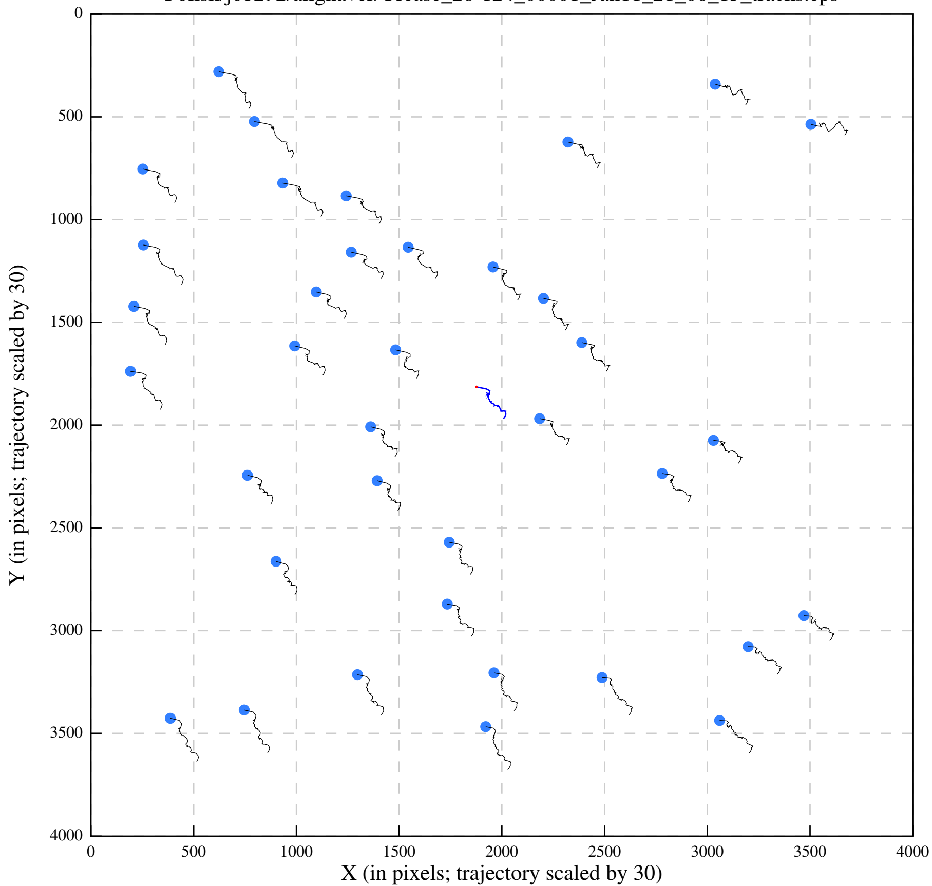
Polish/job292/alignaver/Urease_28-124_00001_Jan11_21_06_15_tracks.eps
