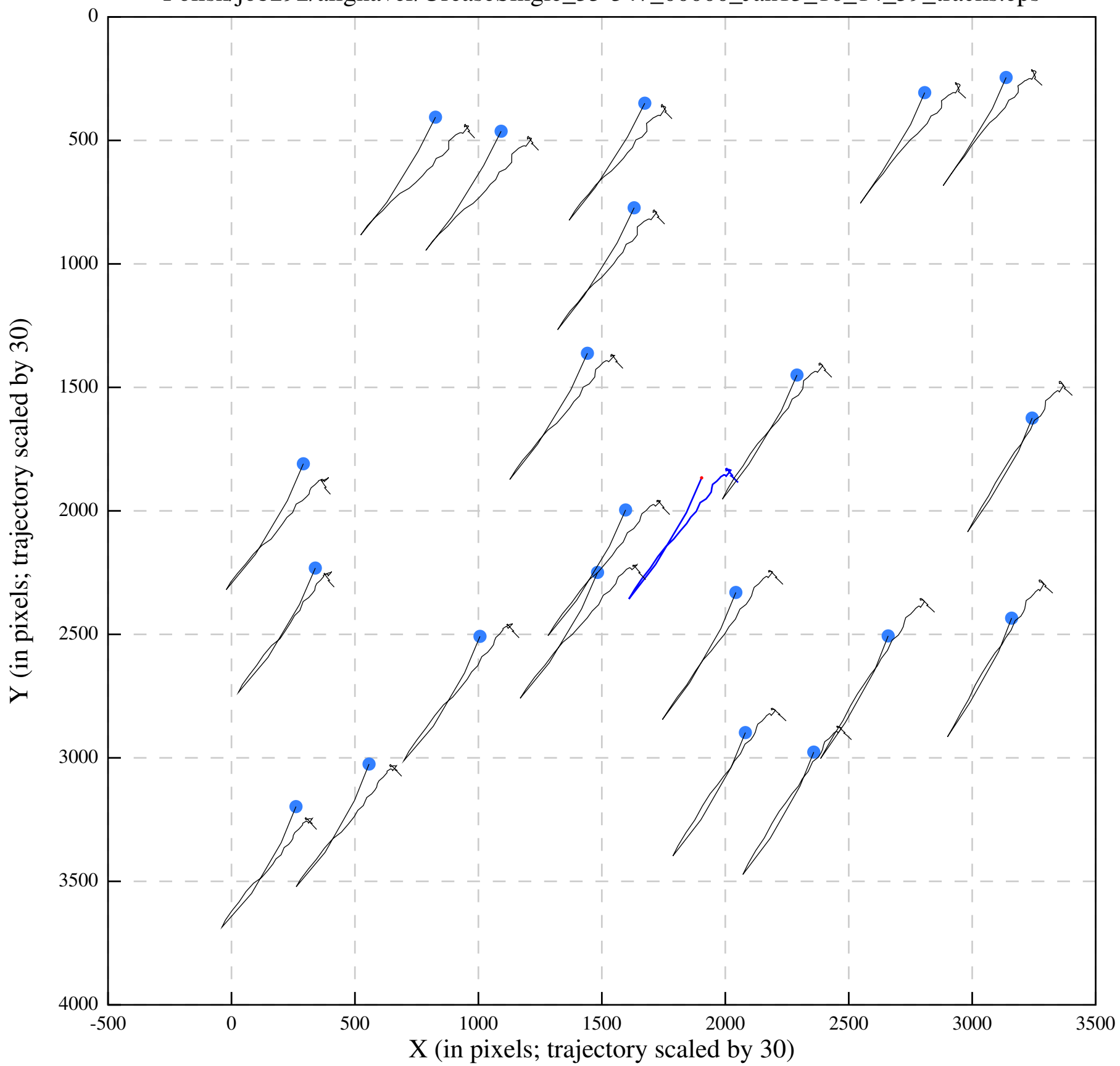
Polish/job292/alignaver/UreaseSingle_35-347_00000_Jan13_16_14_59_tracks.eps
