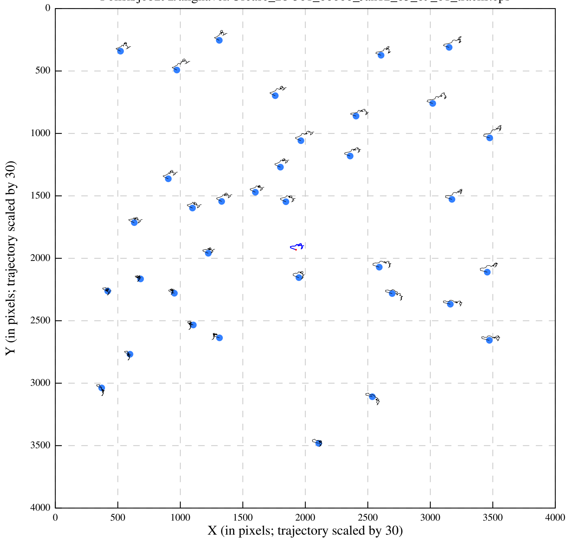
Polish/job292/alignaver/Urease_28-301_00000_Jan12_03_09_01_tracks.eps
