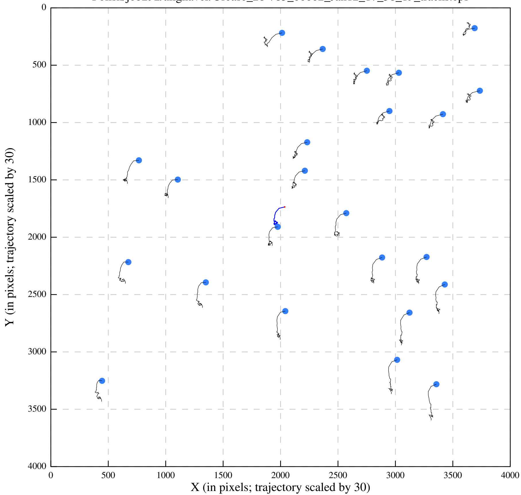
Polish/job292/alignaver/Urease_28-783_00002_Jan12_17_58_19_tracks.eps
