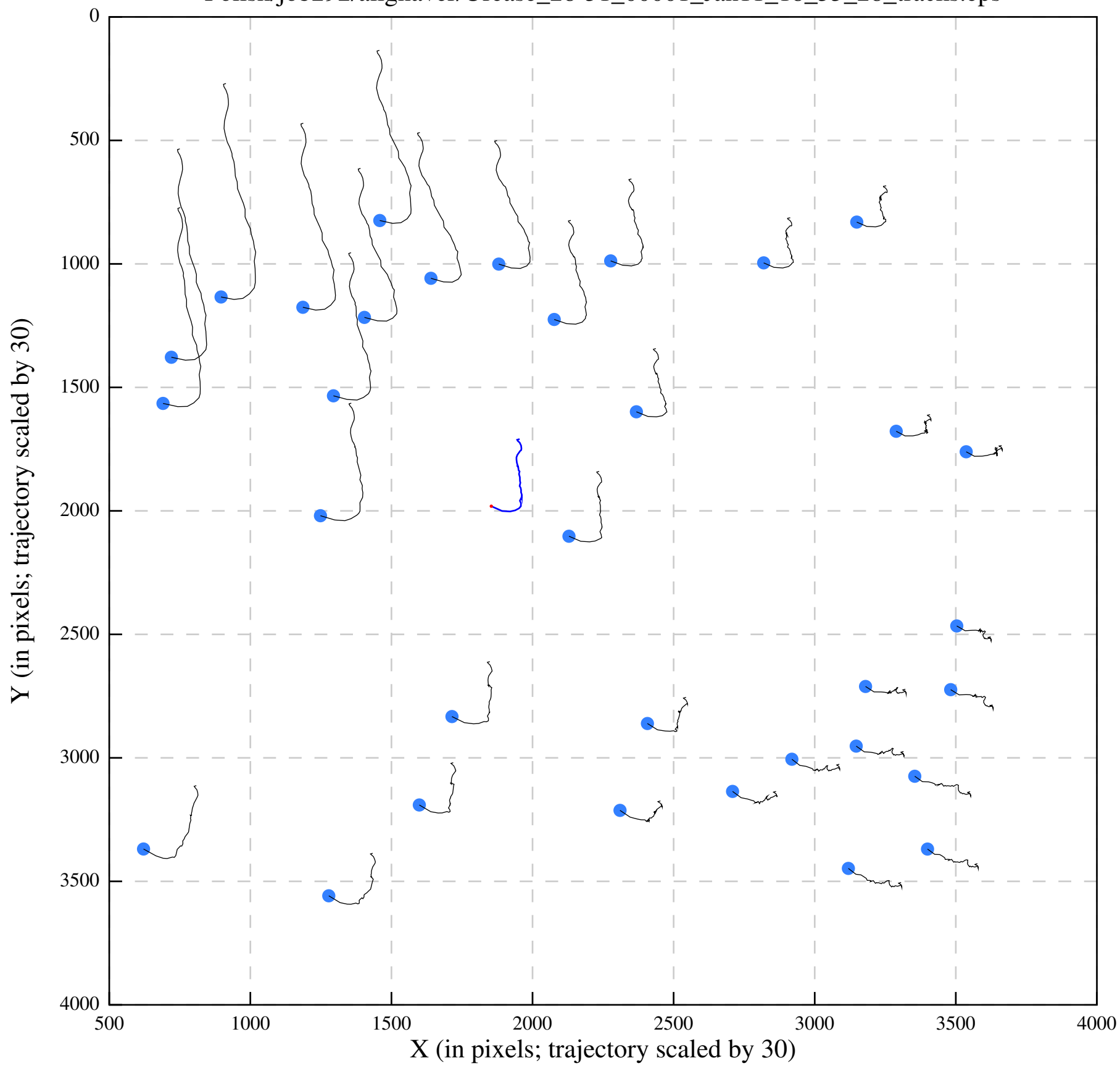
Polish/job292/alignaver/Urease_28-51_00001_Jan11_18_55_28_tracks.eps
