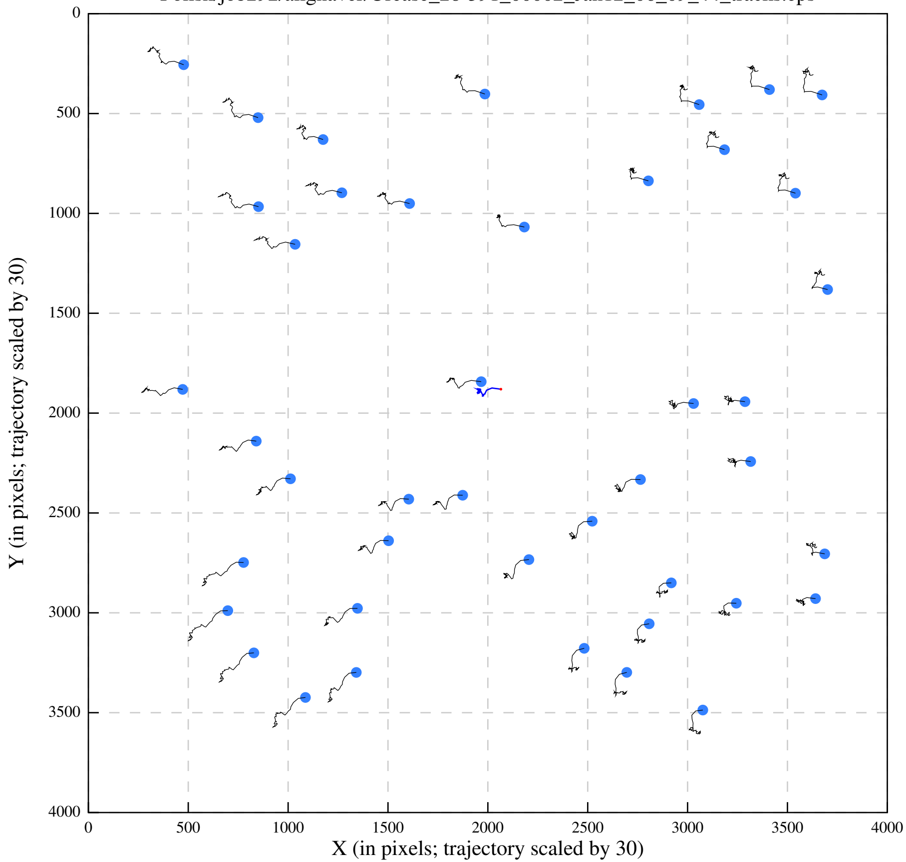
Polish/job292/alignaver/Urease_28-391_00002_Jan12_06_09_44_tracks.eps
