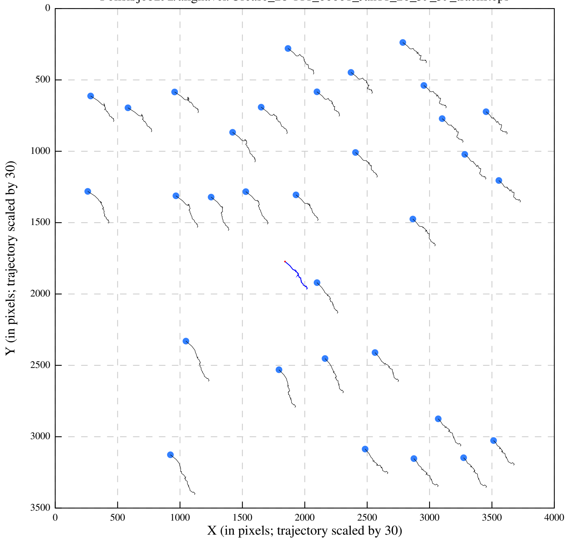
Polish/job292/alignaver/Urease_28-111_00001_Jan11_20_39_59_tracks.eps
