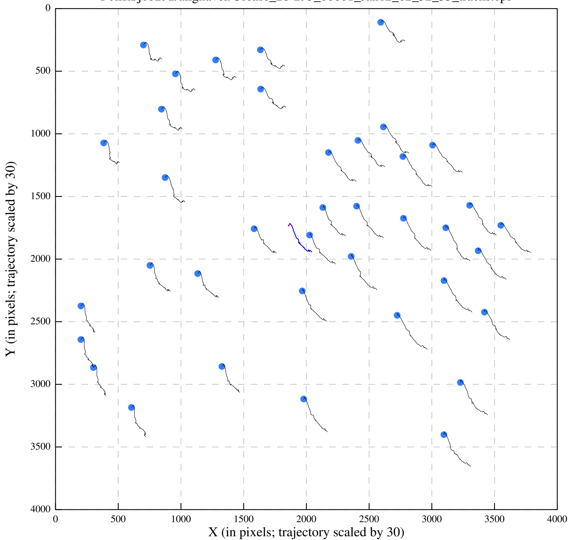
Polish/job292/alignaver/Urease_28-293_00001_Jan12_02_52_55_tracks.eps
