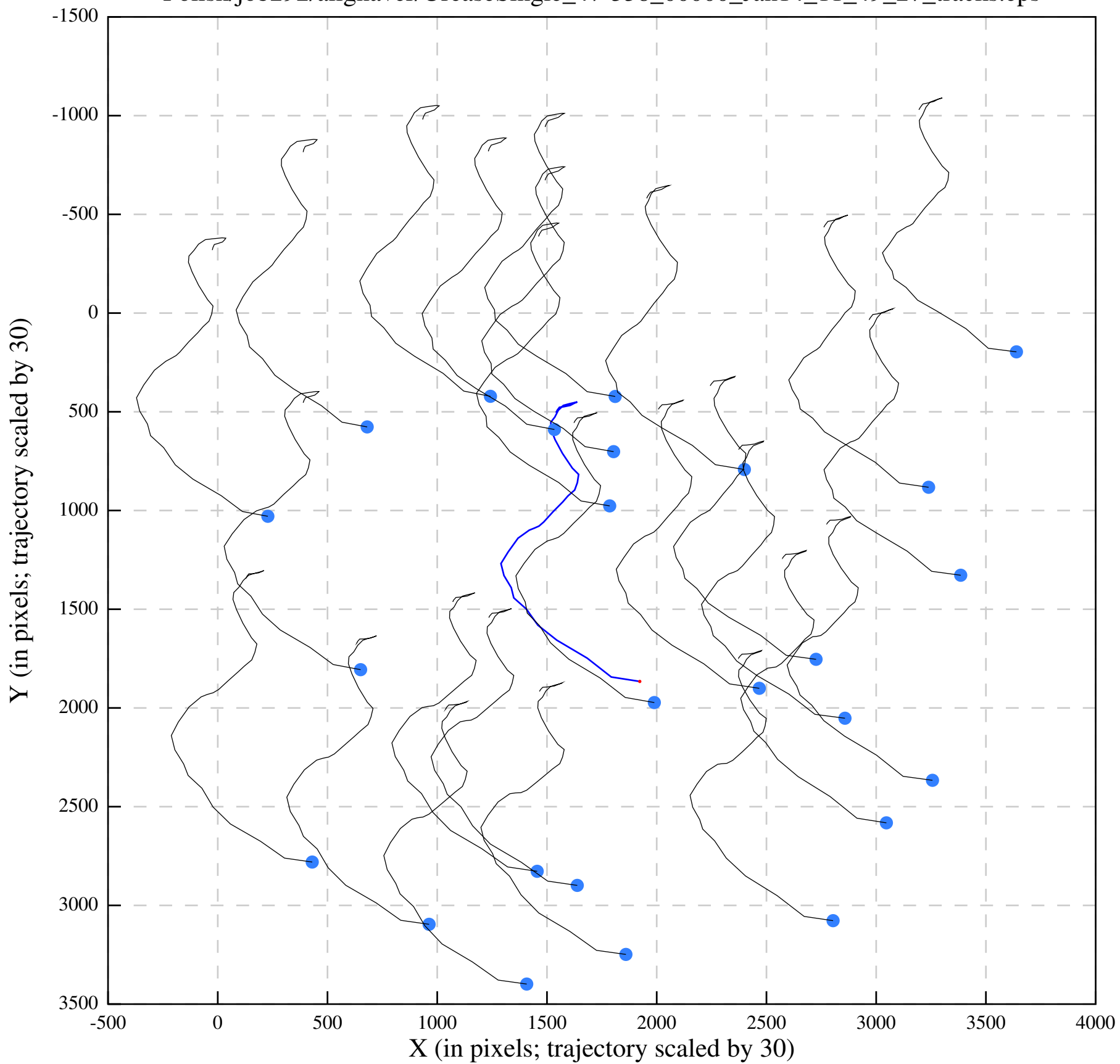
Polish/job292/alignaver/UreaseSingle_47-338_00000_Jan14_11_49_27_tracks.eps
