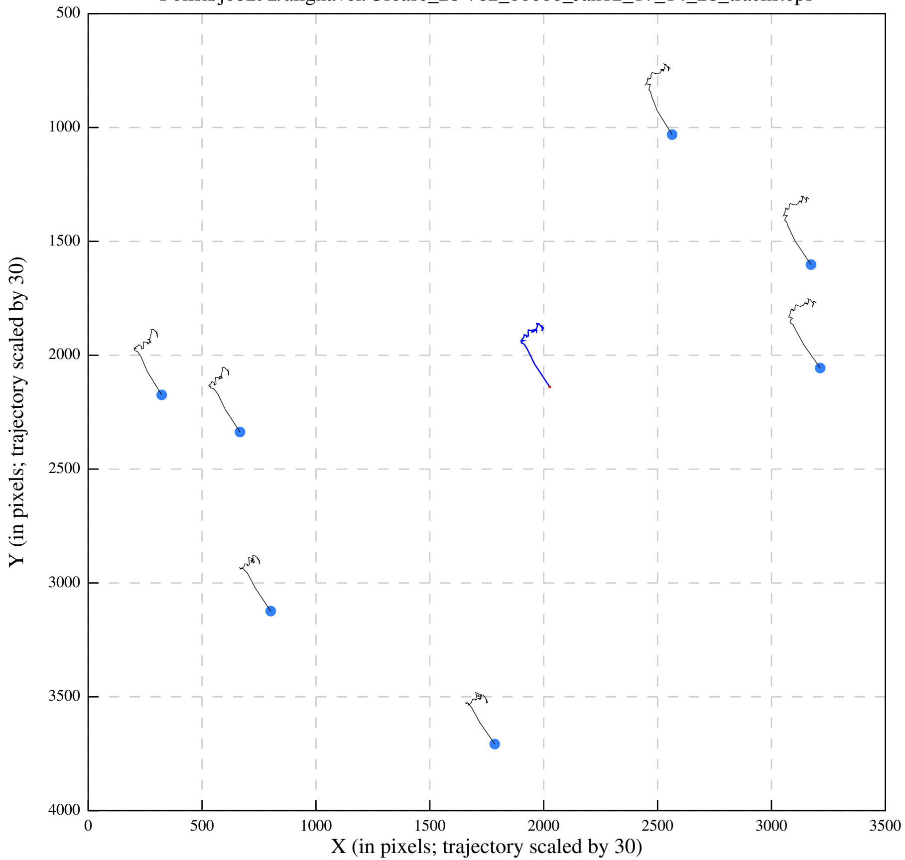
Polish/job292/alignaver/Urease_28-762_00000_Jan12_17_14_28_tracks.eps
