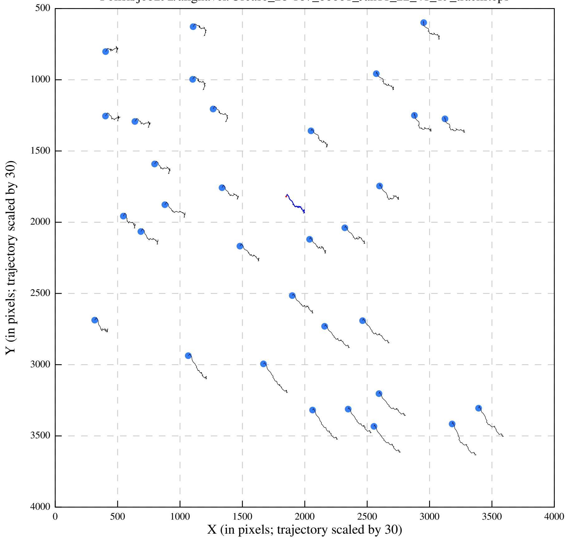
Polish/job292/alignaver/Urease_28-167_00001_Jan11_22_41_19_tracks.eps
