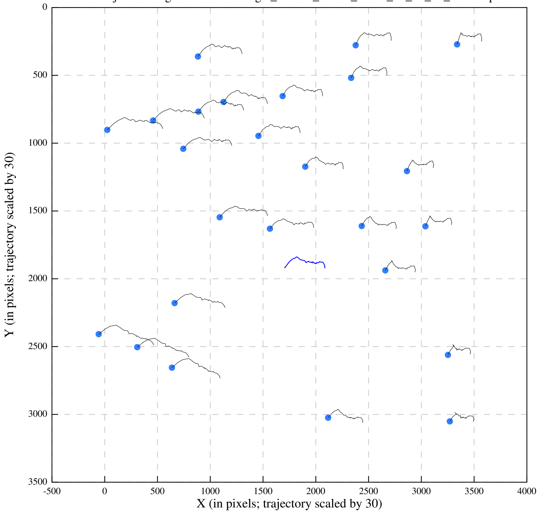
Polish/job292/alignaver/UreaseSingle_47-466_00000_Jan14_13_20_24_tracks.eps
