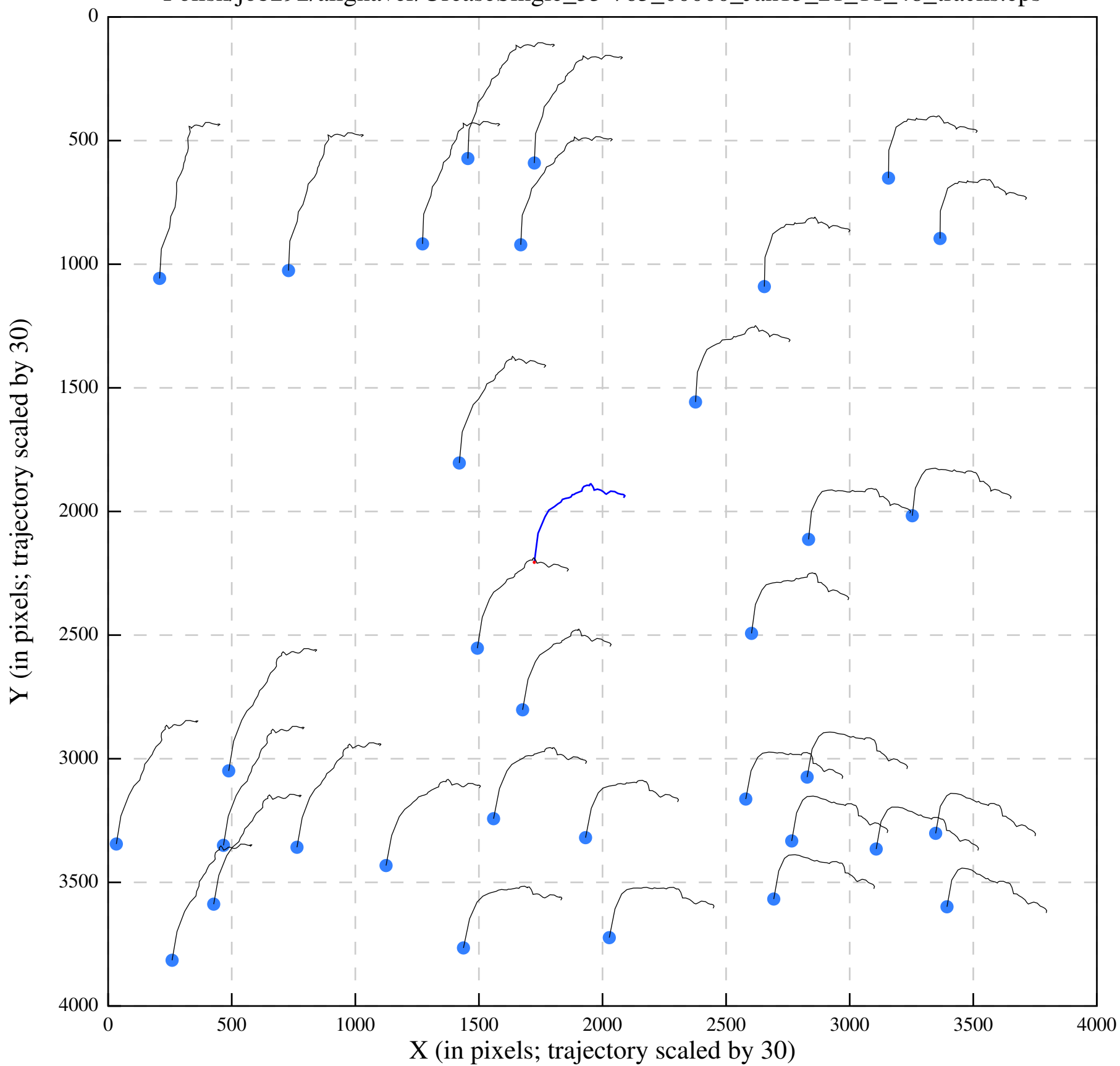
Polish/job292/alignaver/UreaseSingle_35-765_00000_Jan13_21_11_48_tracks.eps
