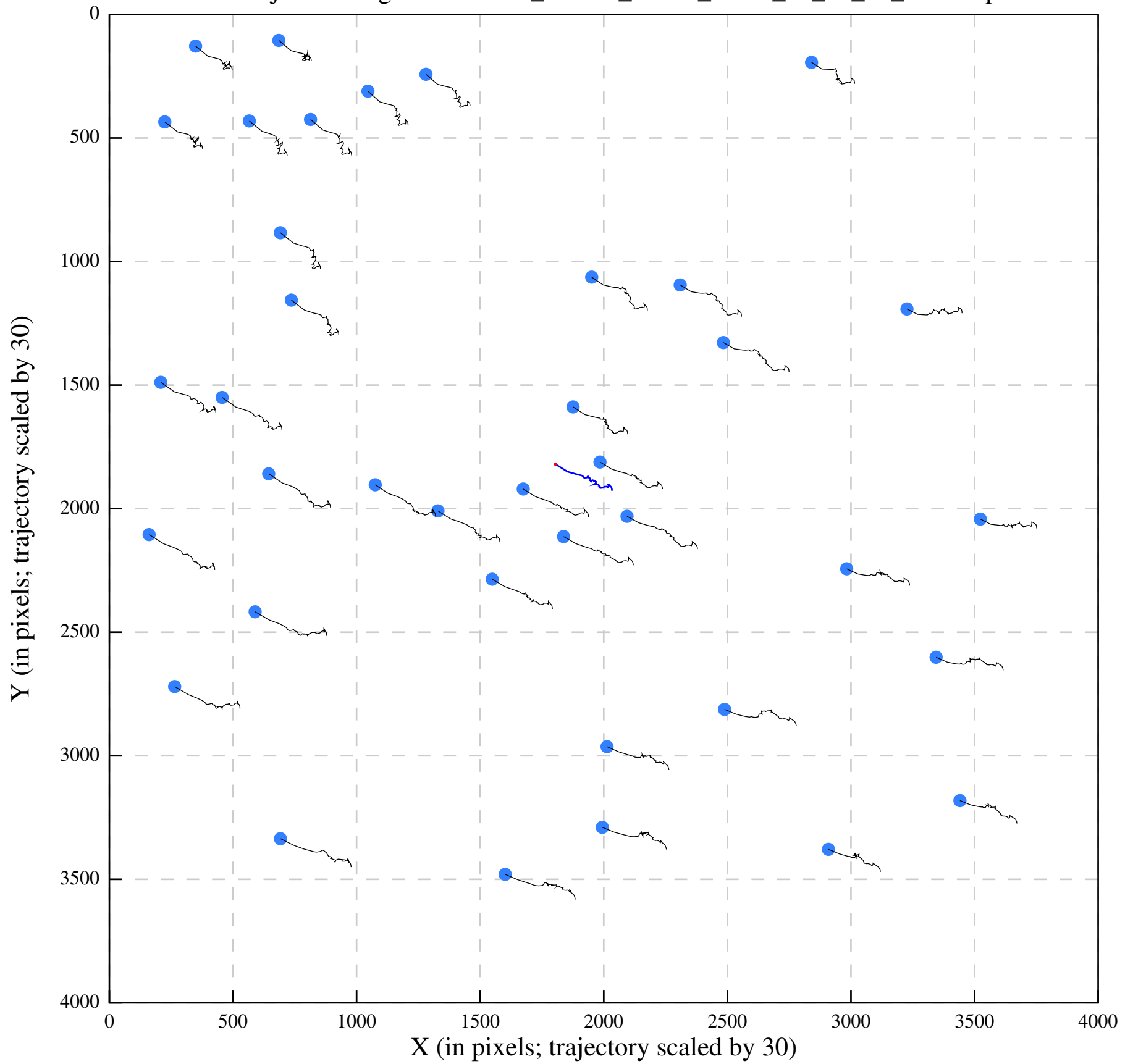
Polish/job292/alignaver/Urease_28-100_00001_Jan11_20_20_40_tracks.eps
