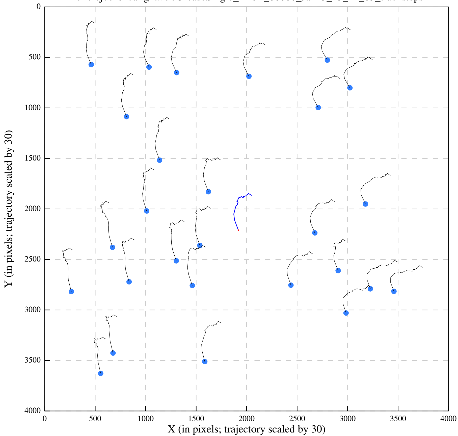
Polish/job292/alignaver/UreaseSingle_41-92_00000_Jan13_23_22_05_tracks.eps
