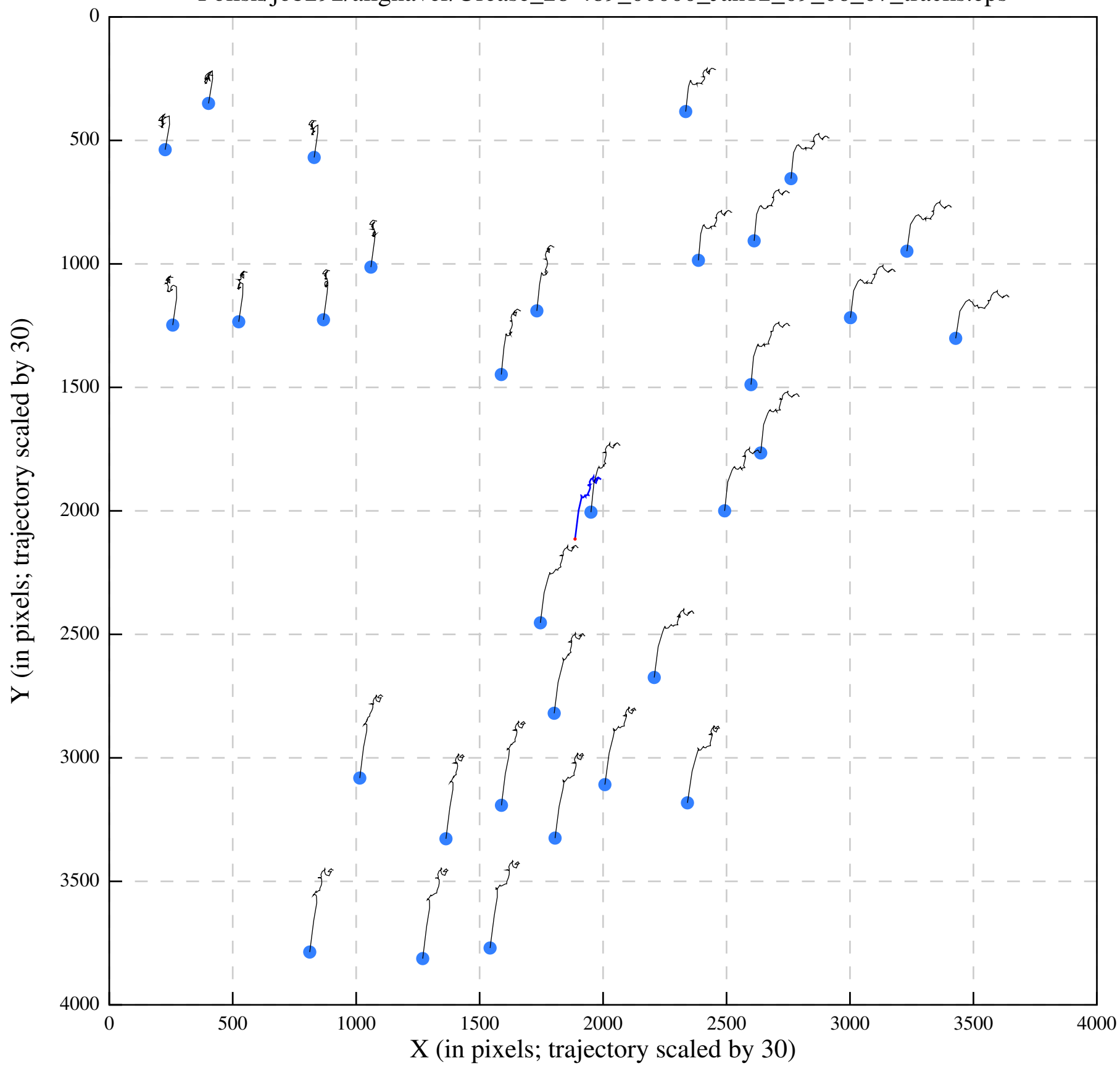
Polish/job292/alignaver/Urease_28-489_00000_Jan12_09_06_07_tracks.eps
