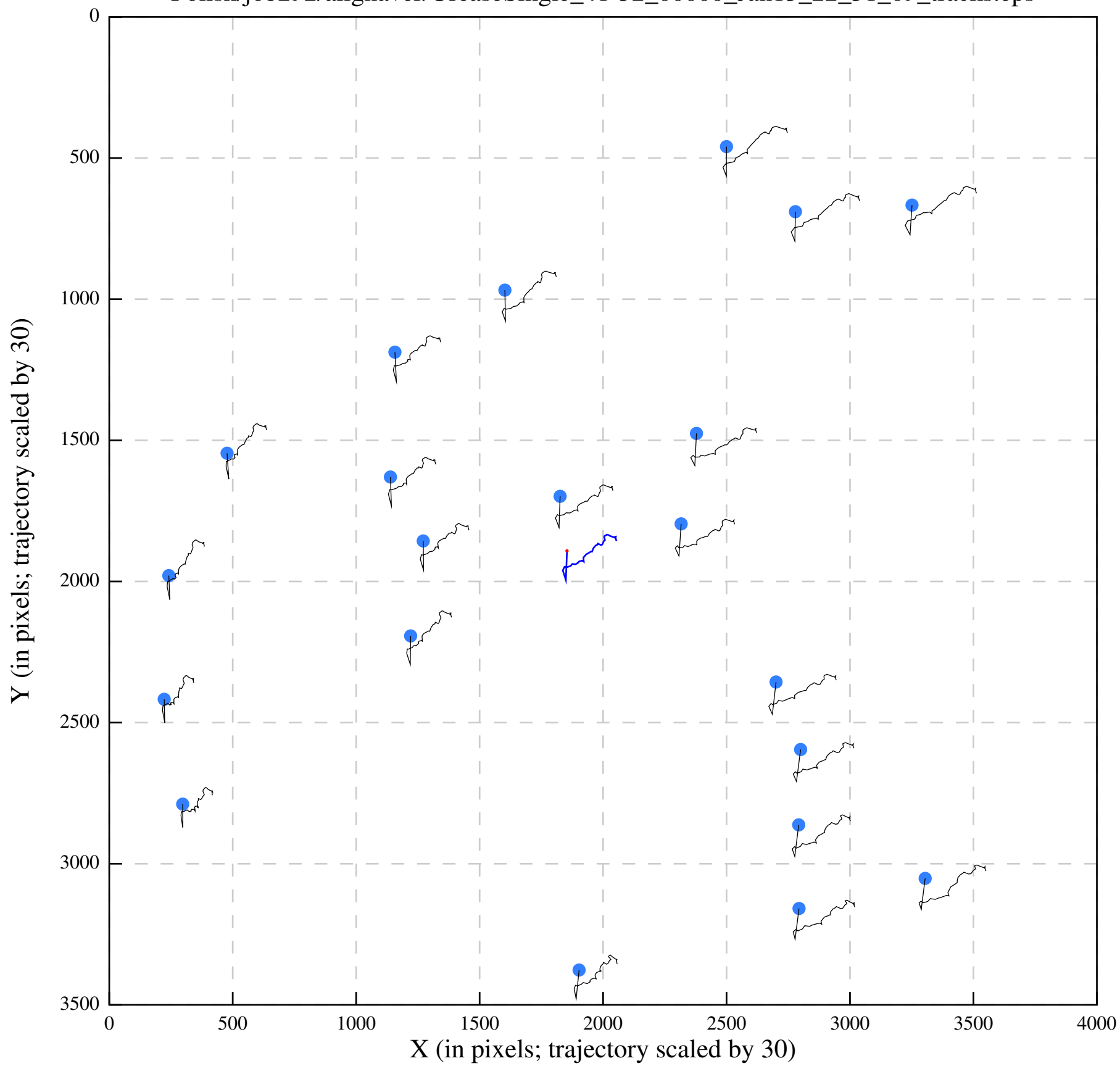
Polish/job292/alignaver/UreaseSingle_41-52_00000_Jan13_22_51_09_tracks.eps
