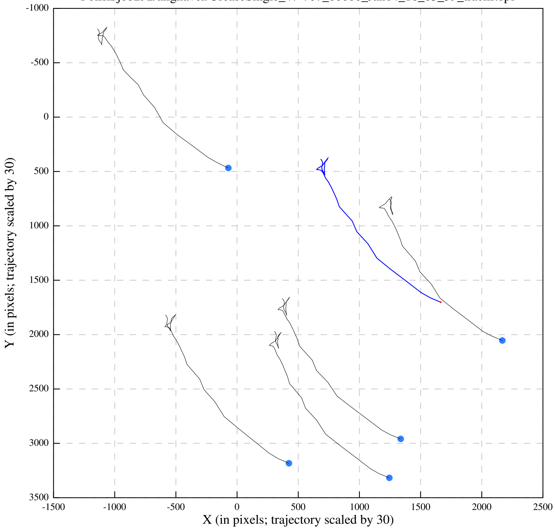
Polish/job292/alignaver/UreaseSingle_47-707_00000_Jan14_16_03_39_tracks.eps
