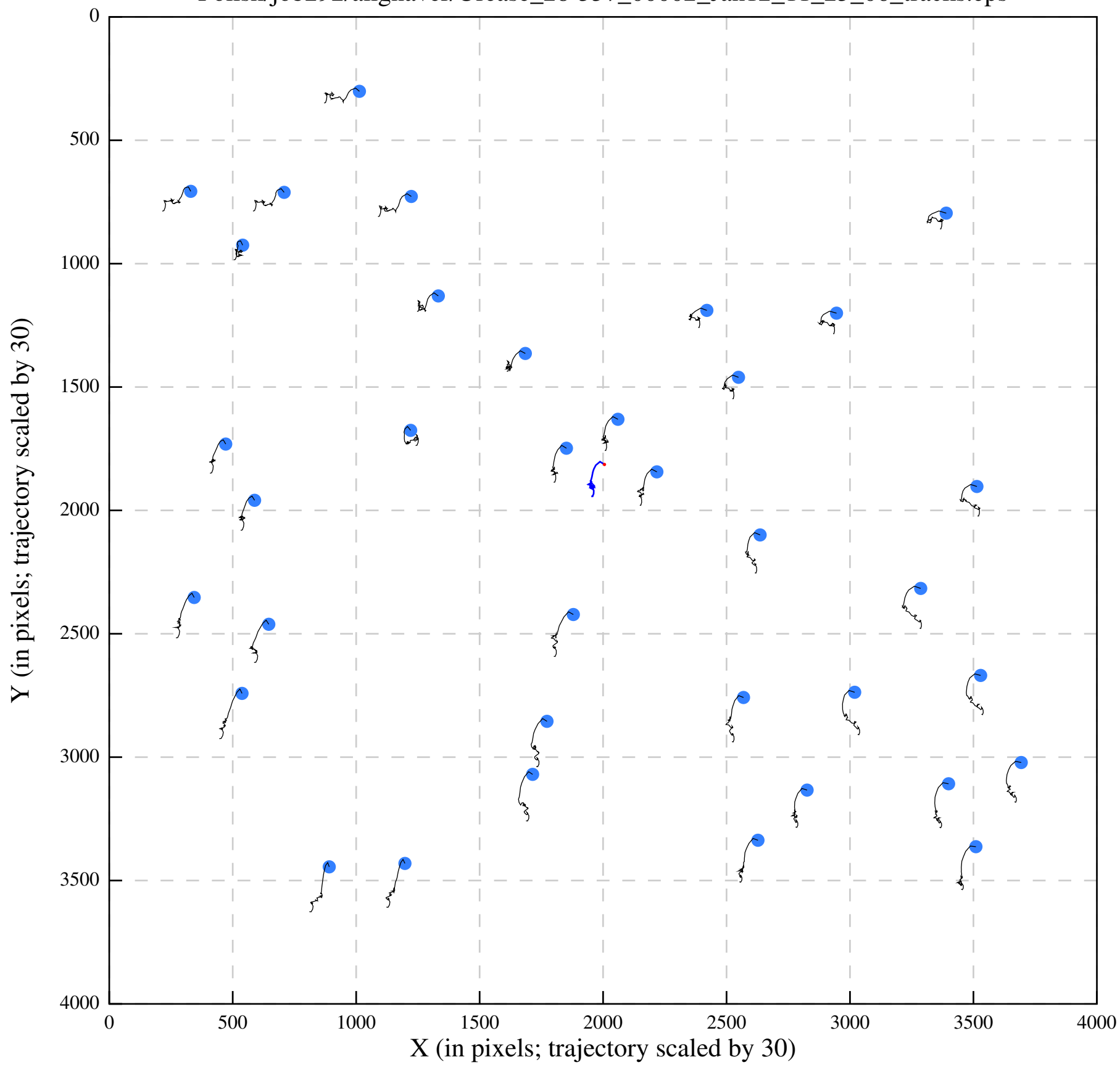
Polish/job292/alignaver/Urease_28-557_00002_Jan12_11_25_06_tracks.eps
