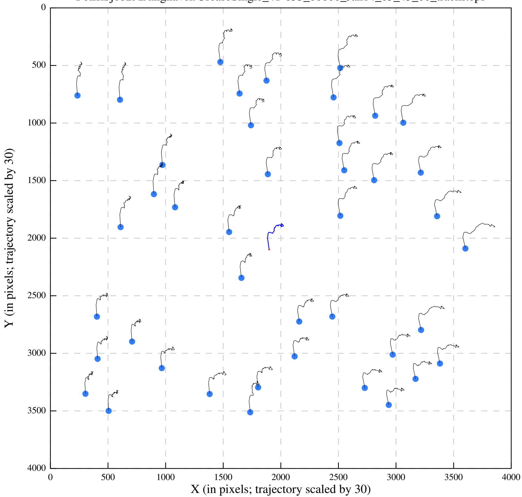
Polish/job292/alignaver/UreaseSingle_41-653_00000_Jan14_05_45_00_tracks.eps
