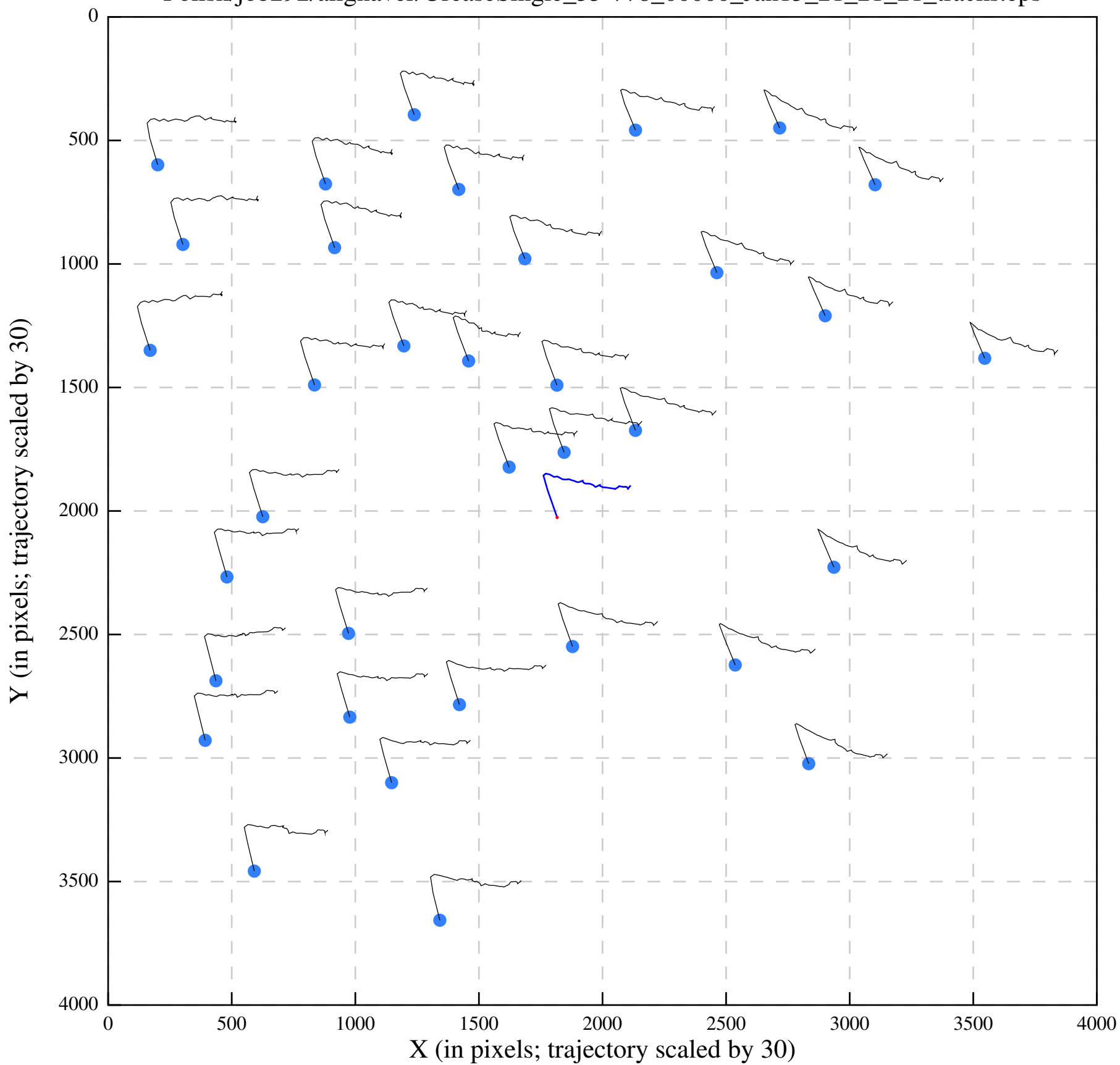
Polish/job292/alignaver/UreaseSingle_35-778_00000_Jan13_21_21_21_tracks.eps
