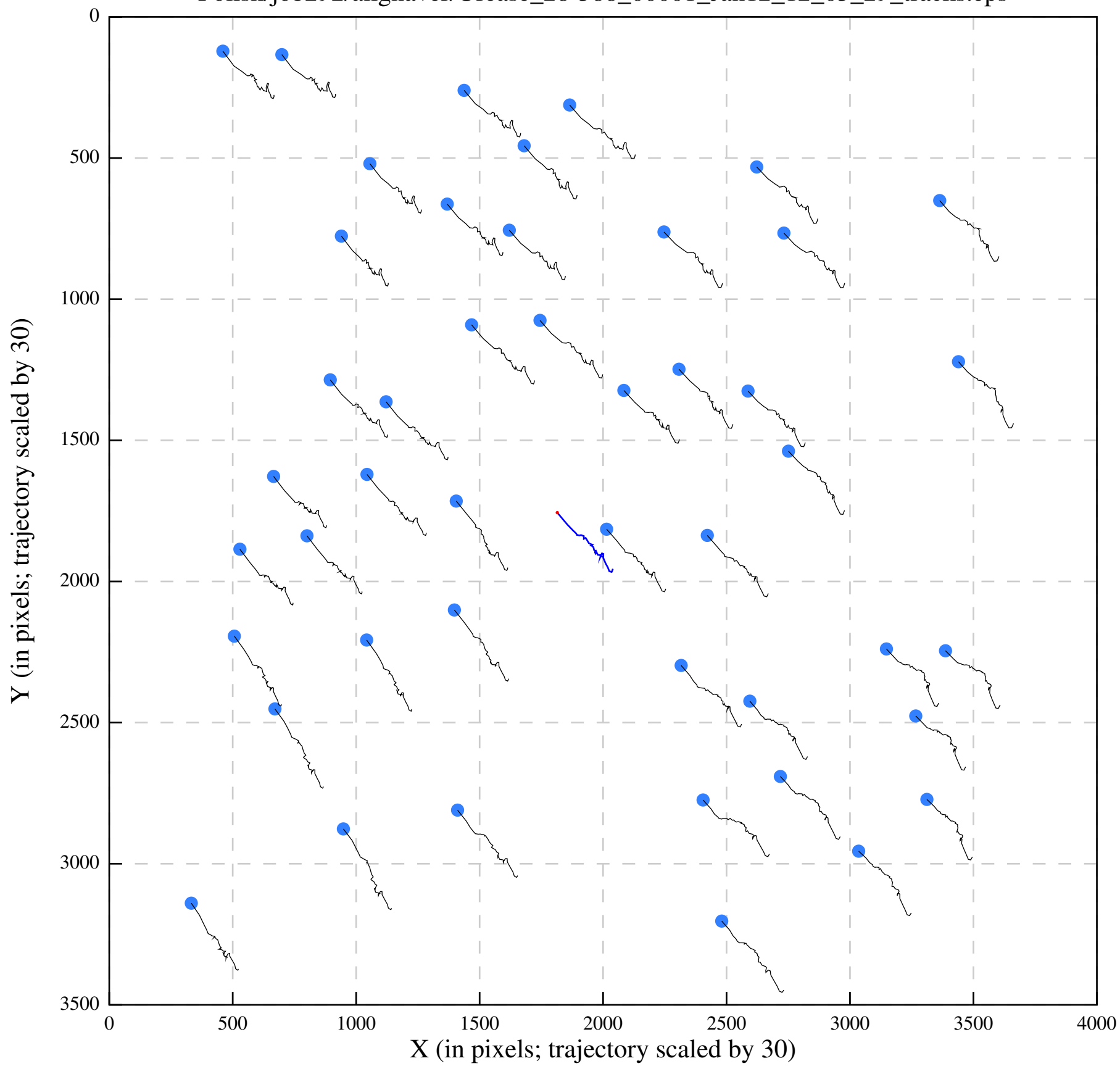
Polish/job292/alignaver/Urease_28-588_00001_Jan12_12_05_29_tracks.eps
