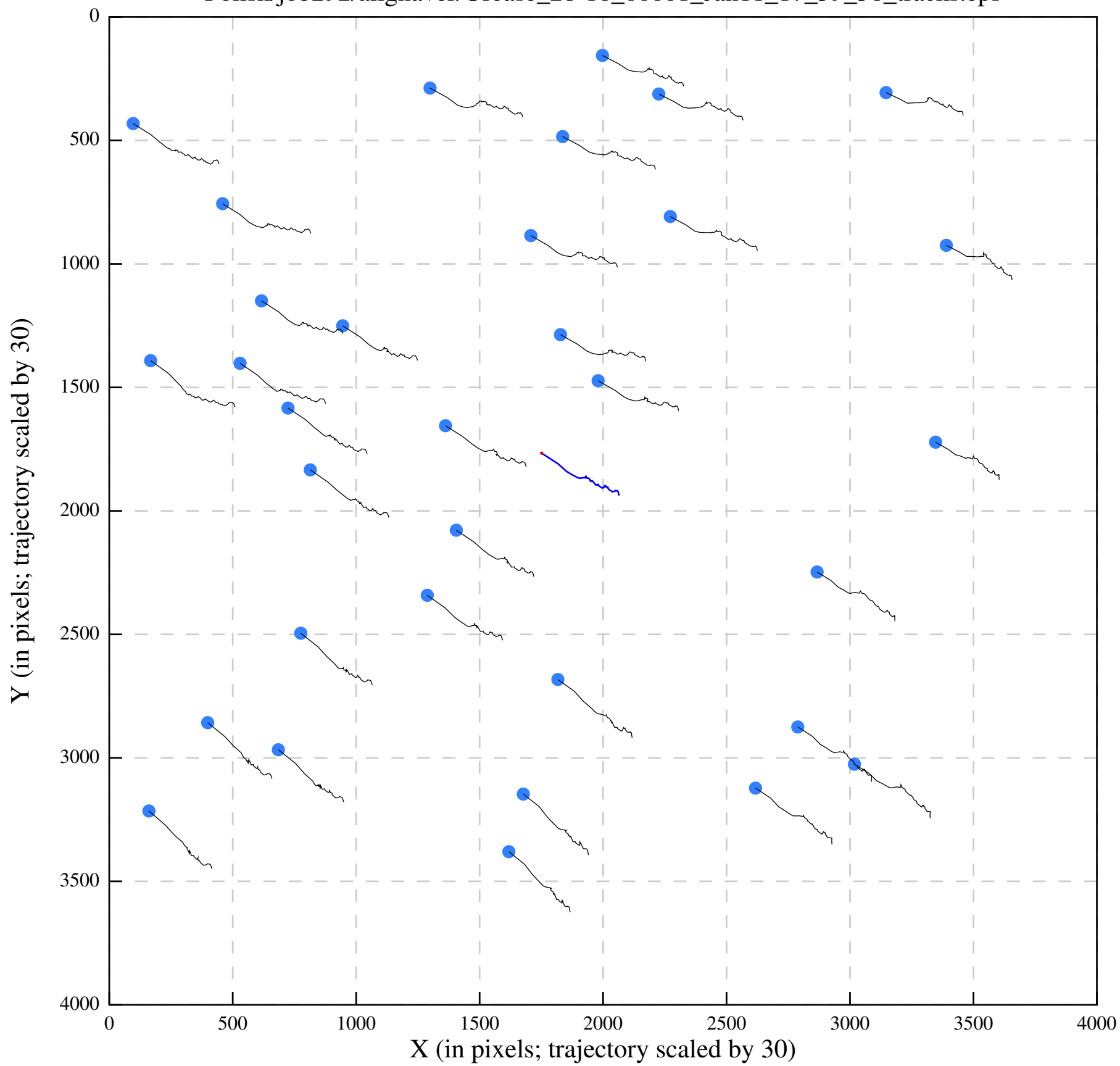
Polish/job292/alignaver/Urease_28-16_00001_Jan11_17_59_56_tracks.eps
