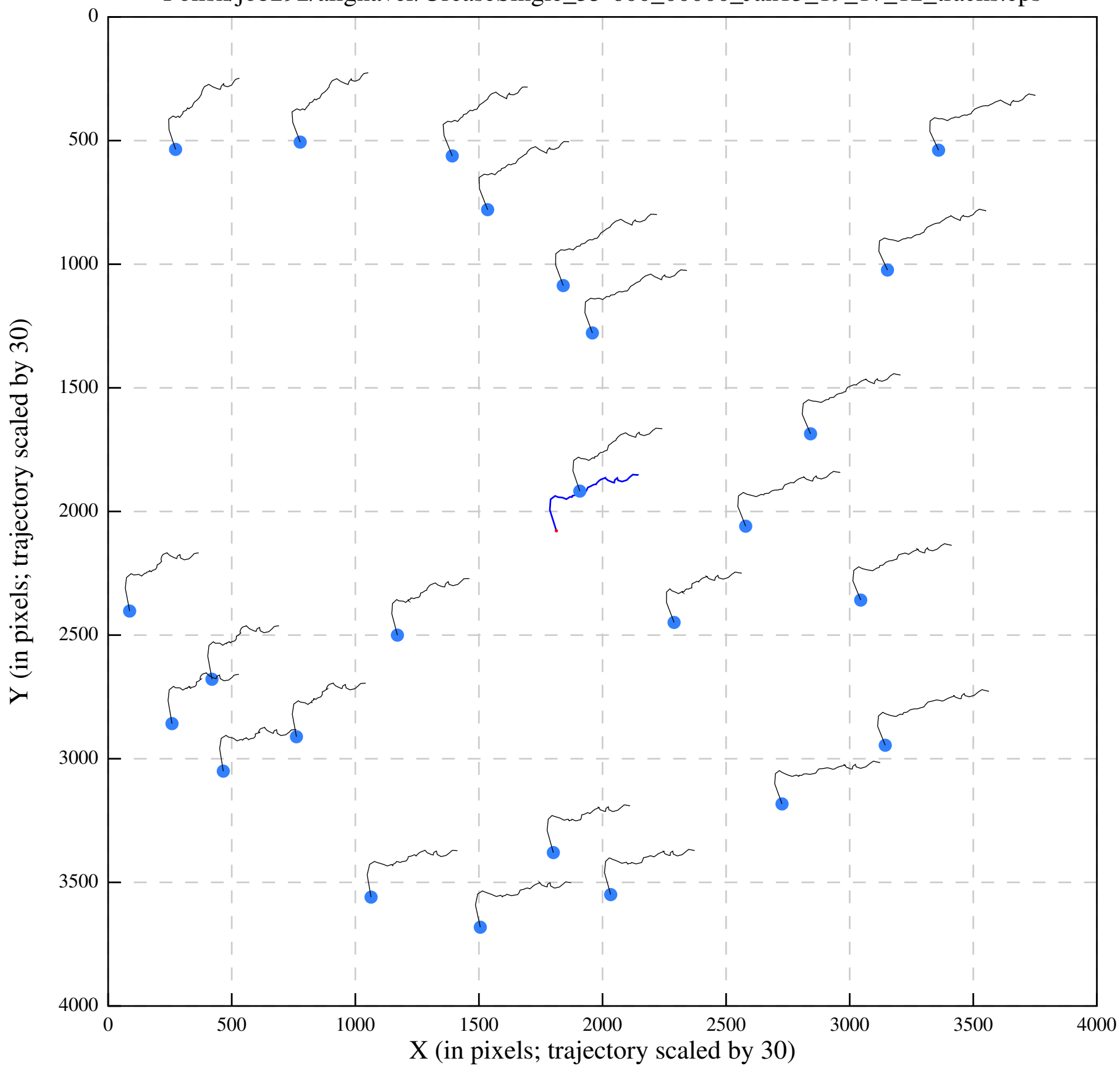
Polish/job292/alignaver/UreaseSingle_35-600_00000_Jan13_19_17_12_tracks.eps
