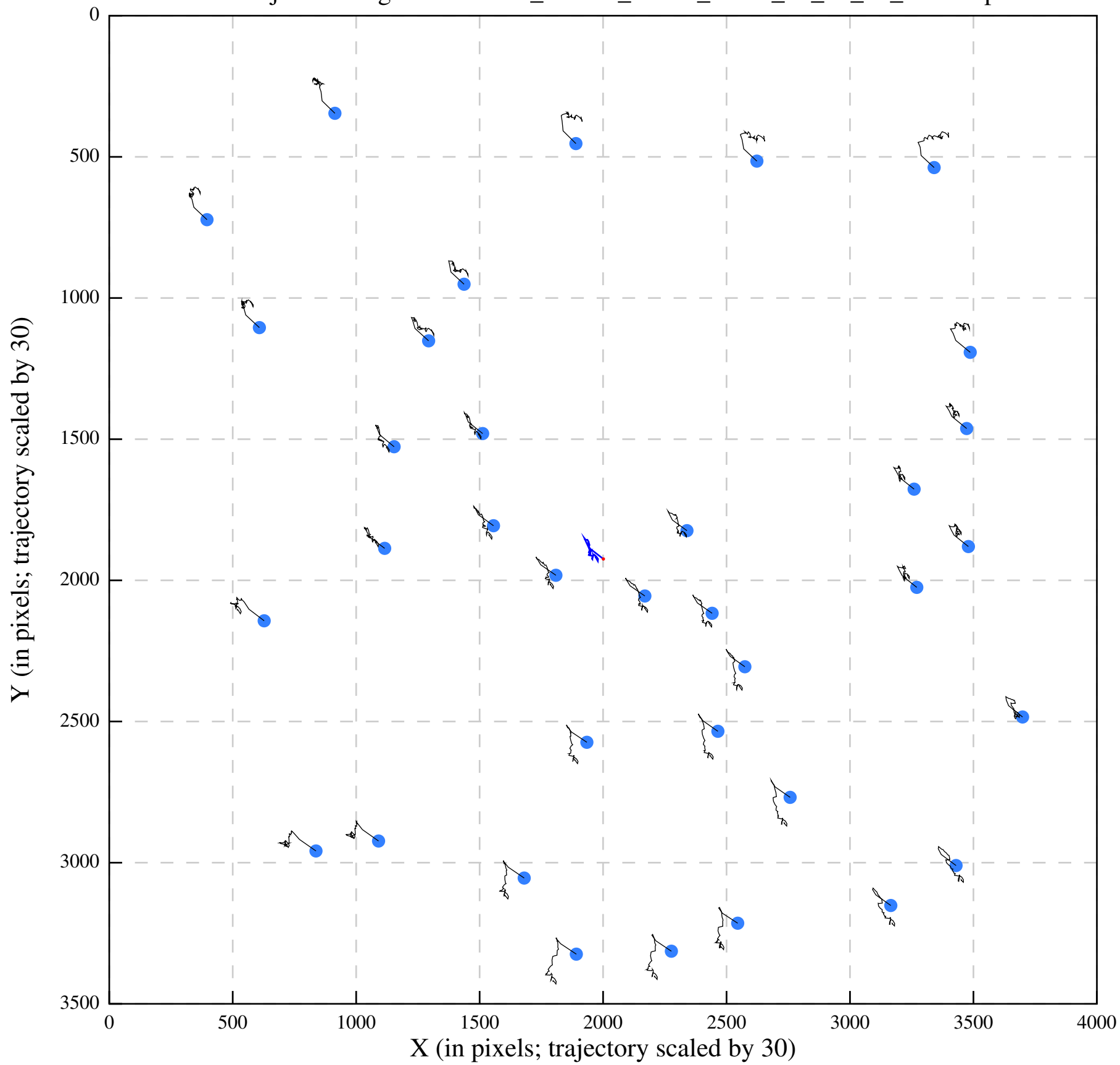
Polish/job292/alignaver/Urease_28-654_00000_Jan12_14_01_20_tracks.eps
