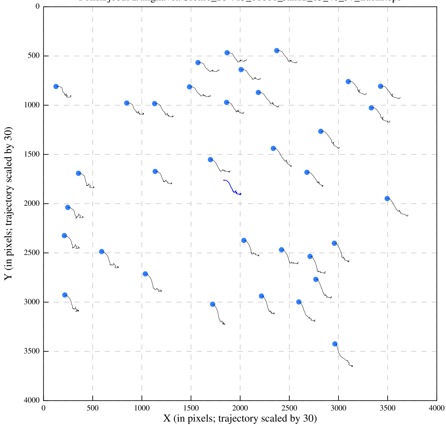
Polish/job292/alignaver/Urease_28-715_00001_Jan12_15_46_37_tracks.eps
