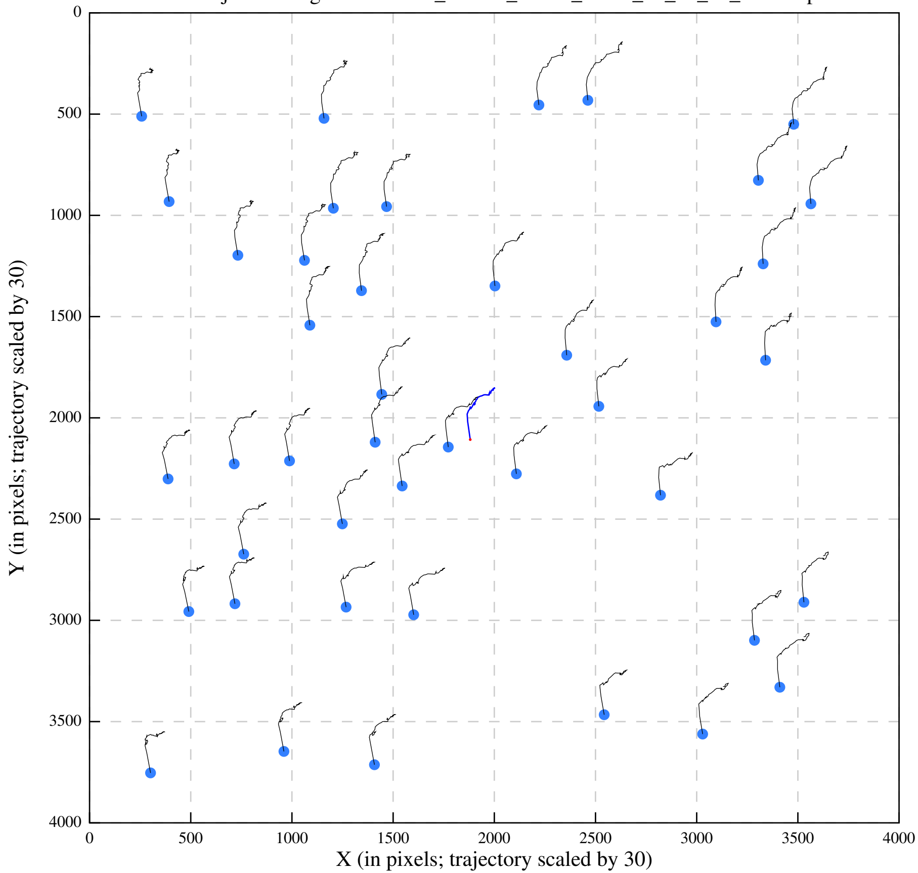
Polish/job292/alignaver/Urease_28-744_00000_Jan12_16_55_02_tracks.eps
