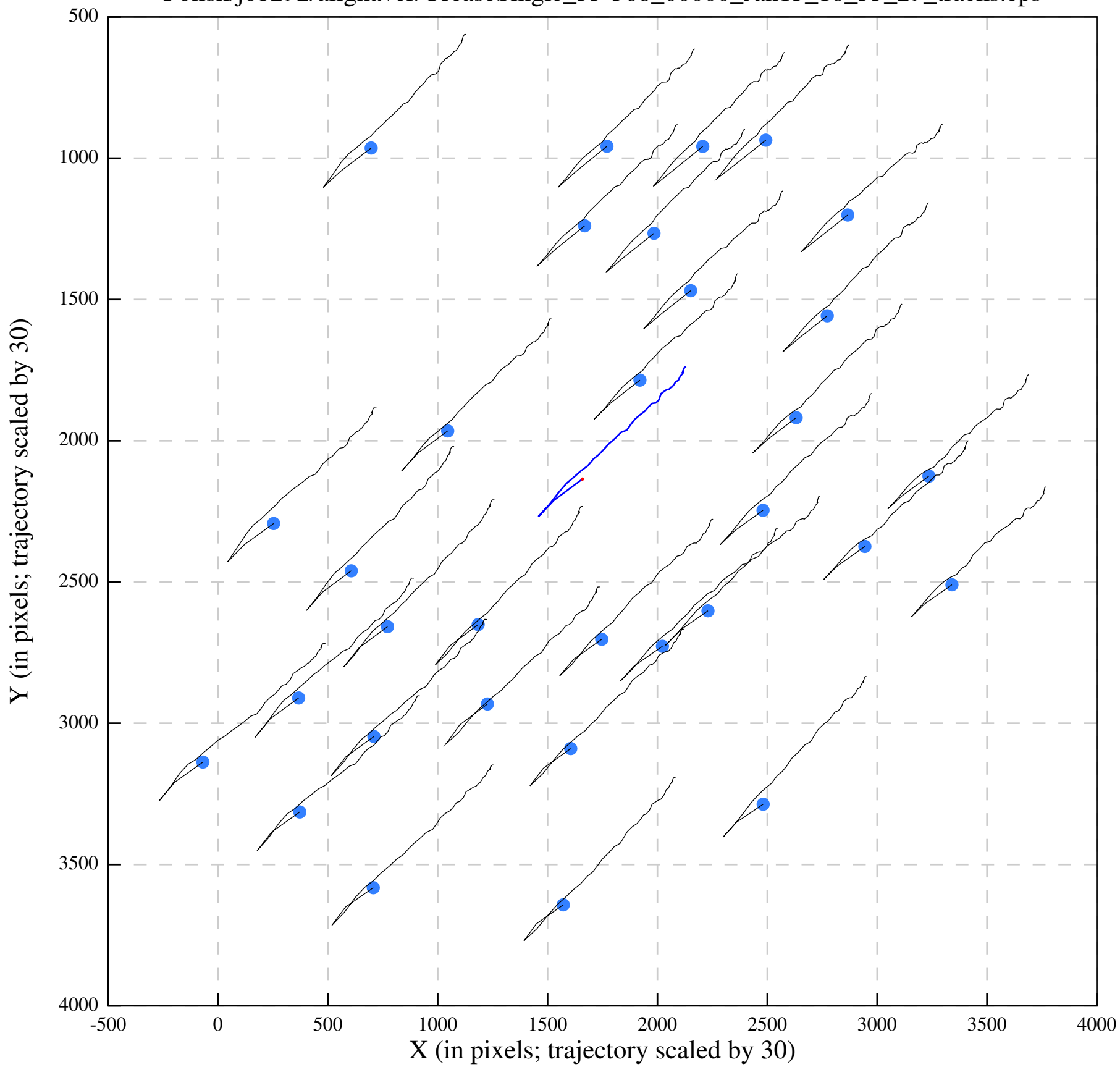
Polish/job292/alignaver/UreaseSingle_35-568_00000_Jan13_18_55_29_tracks.eps
