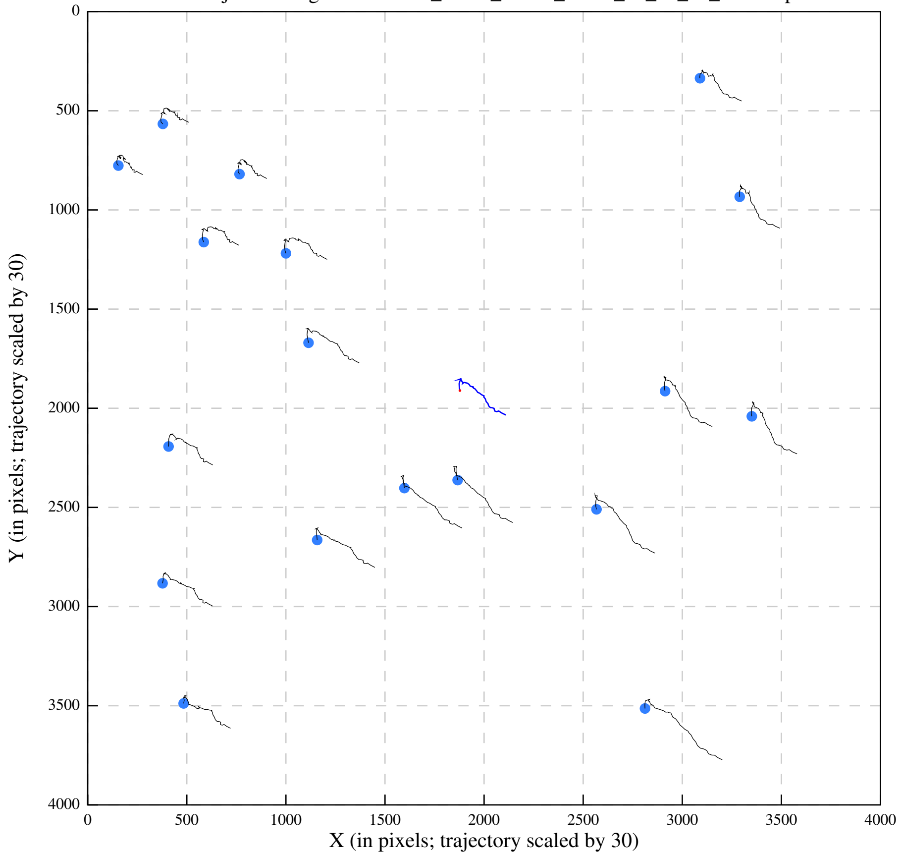
Polish/job292/alignaver/Urease_28-34_00000_Jan11_18_21_39_tracks.eps
