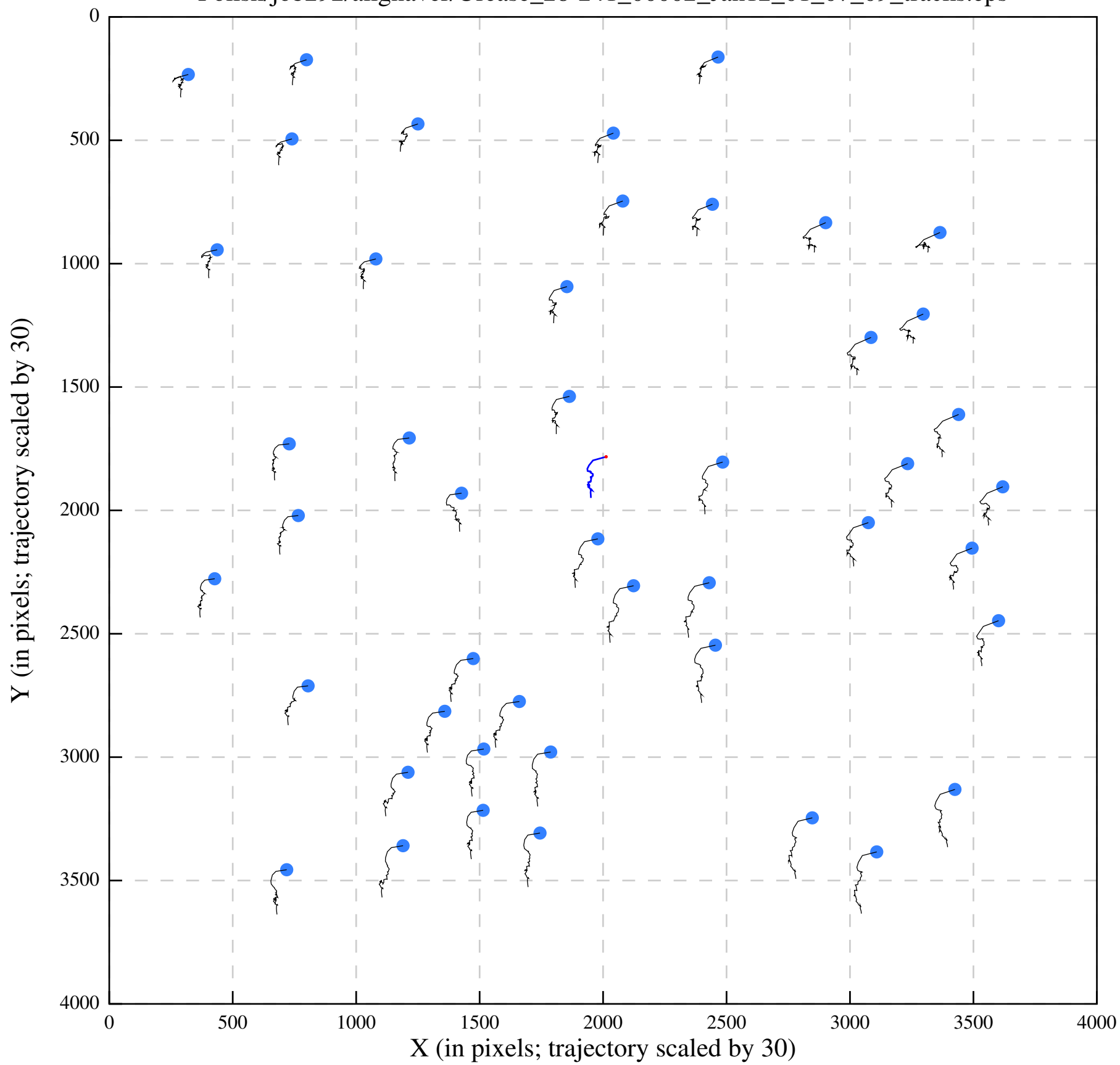
Polish/job292/alignaver/Urease_28-241_00002_Jan12_01_07_09_tracks.eps
