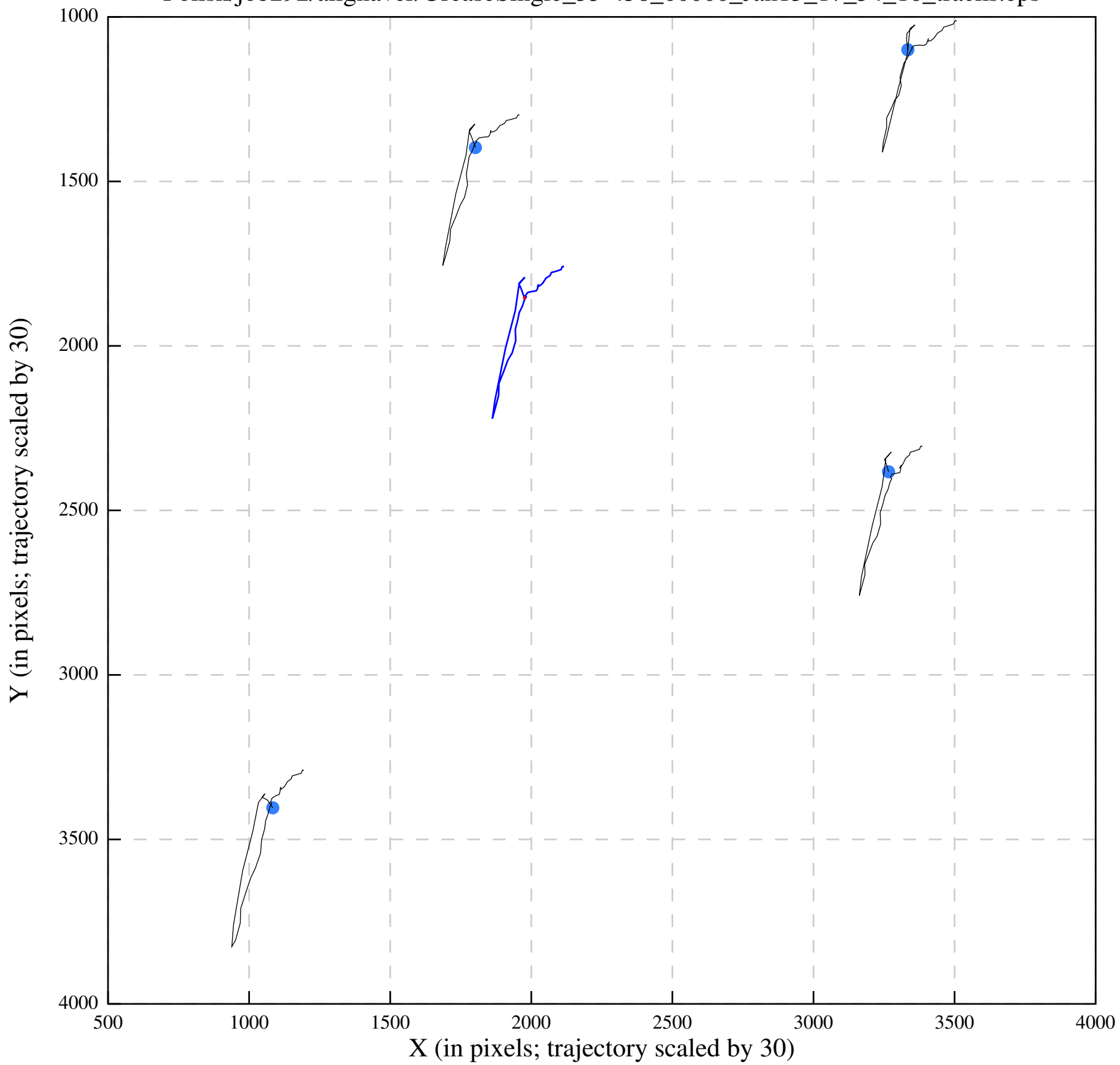
Polish/job292/alignaver/UreaseSingle_35-458_00000_Jan13_17_34_16_tracks.eps
