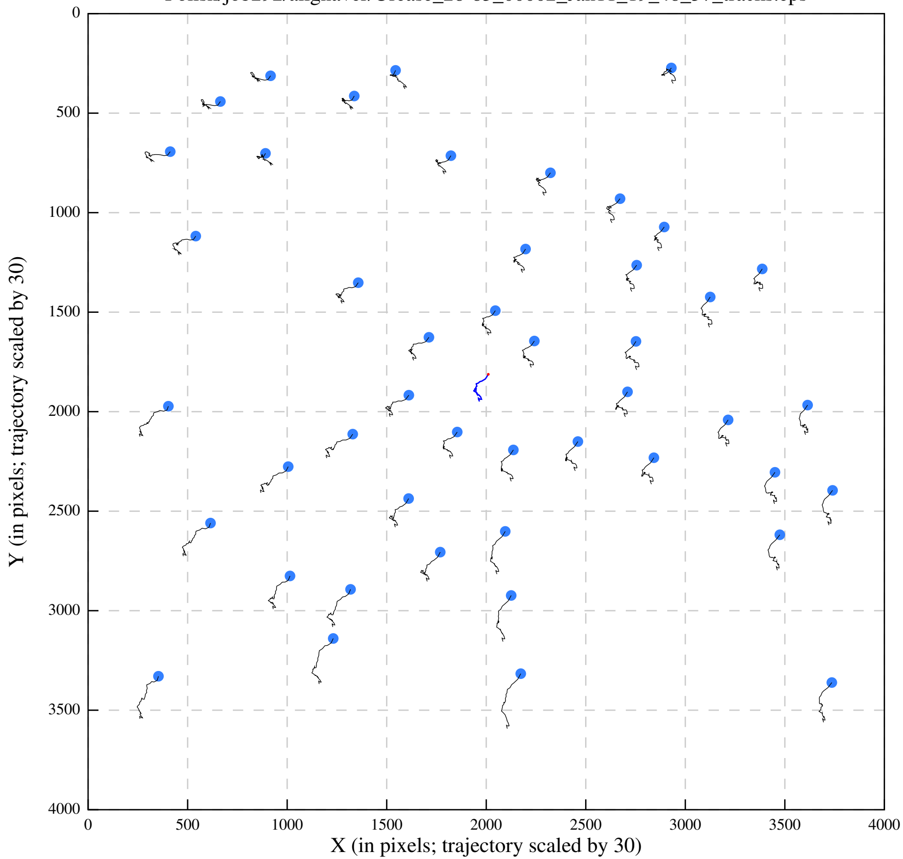
Polish/job292/alignaver/Urease_28-83_00002_Jan11_19_48_57_tracks.eps
