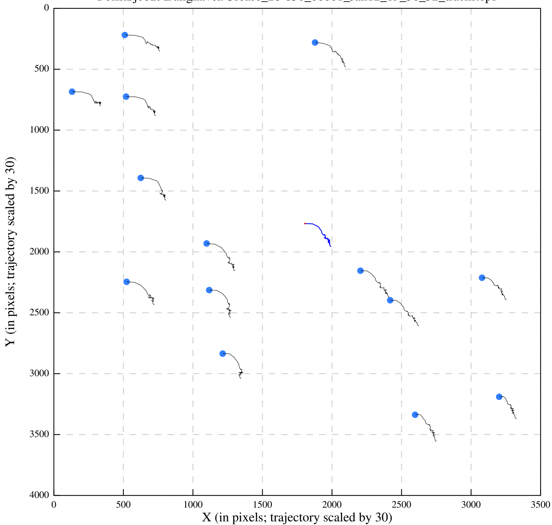
Polish/job292/alignaver/Urease_28-850_00001_Jan12_19_30_52_tracks.eps
