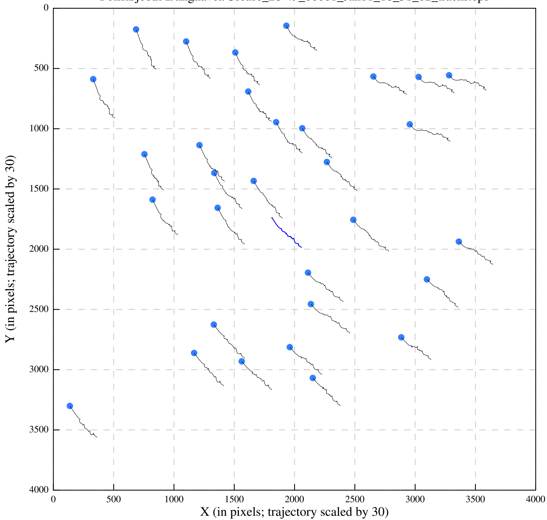
Polish/job292/alignaver/Urease_28-49_00001_Jan11_18_51_02_tracks.eps
