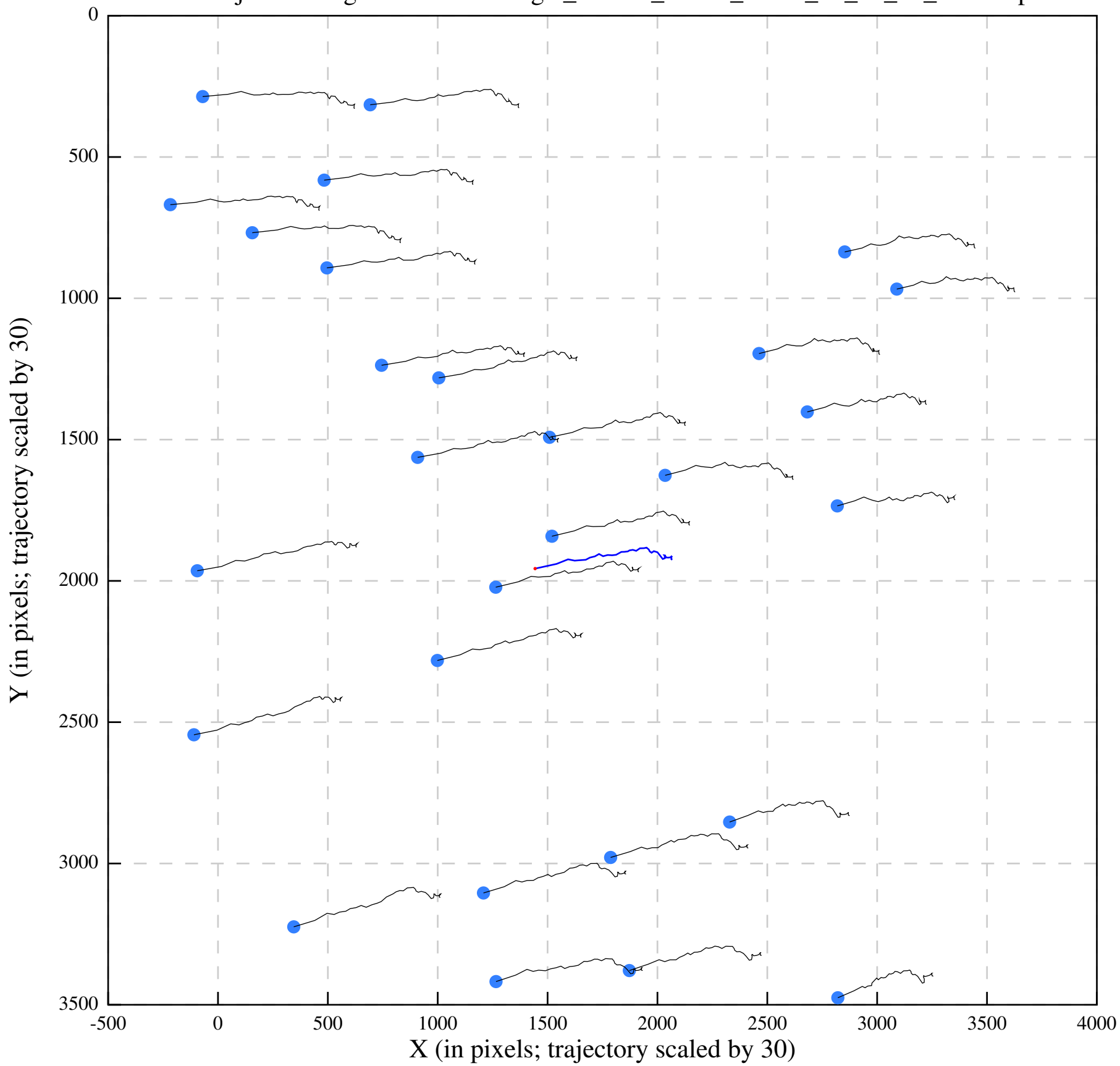
Polish/job292/alignaver/UreaseSingle_35-281_00000_Jan13_15_29_21_tracks.eps
