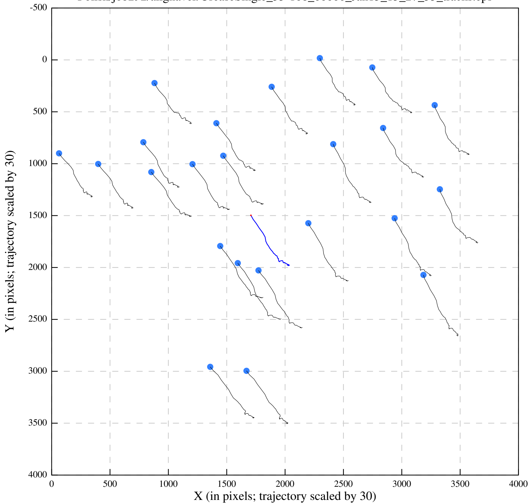
Polish/job292/alignaver/UreaseSingle_35-108_00000_Jan13_13_27_55_tracks.eps
