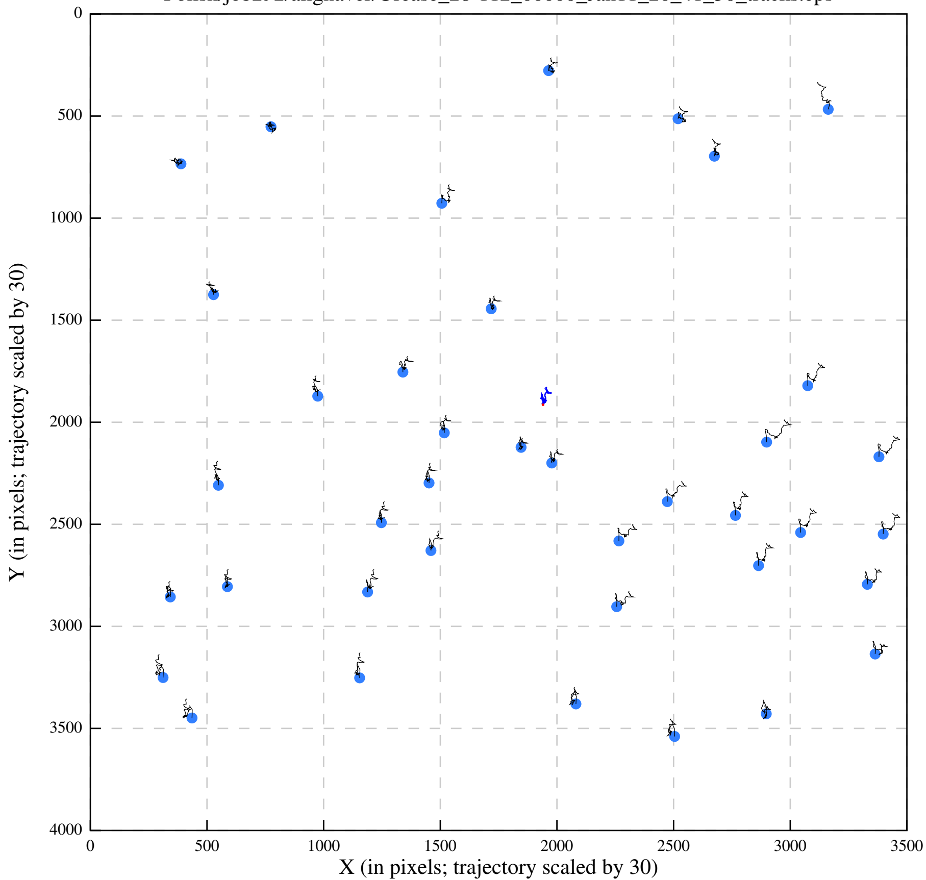
Polish/job292/alignaver/Urease_28-112_00000_Jan11_20_41_50_tracks.eps
