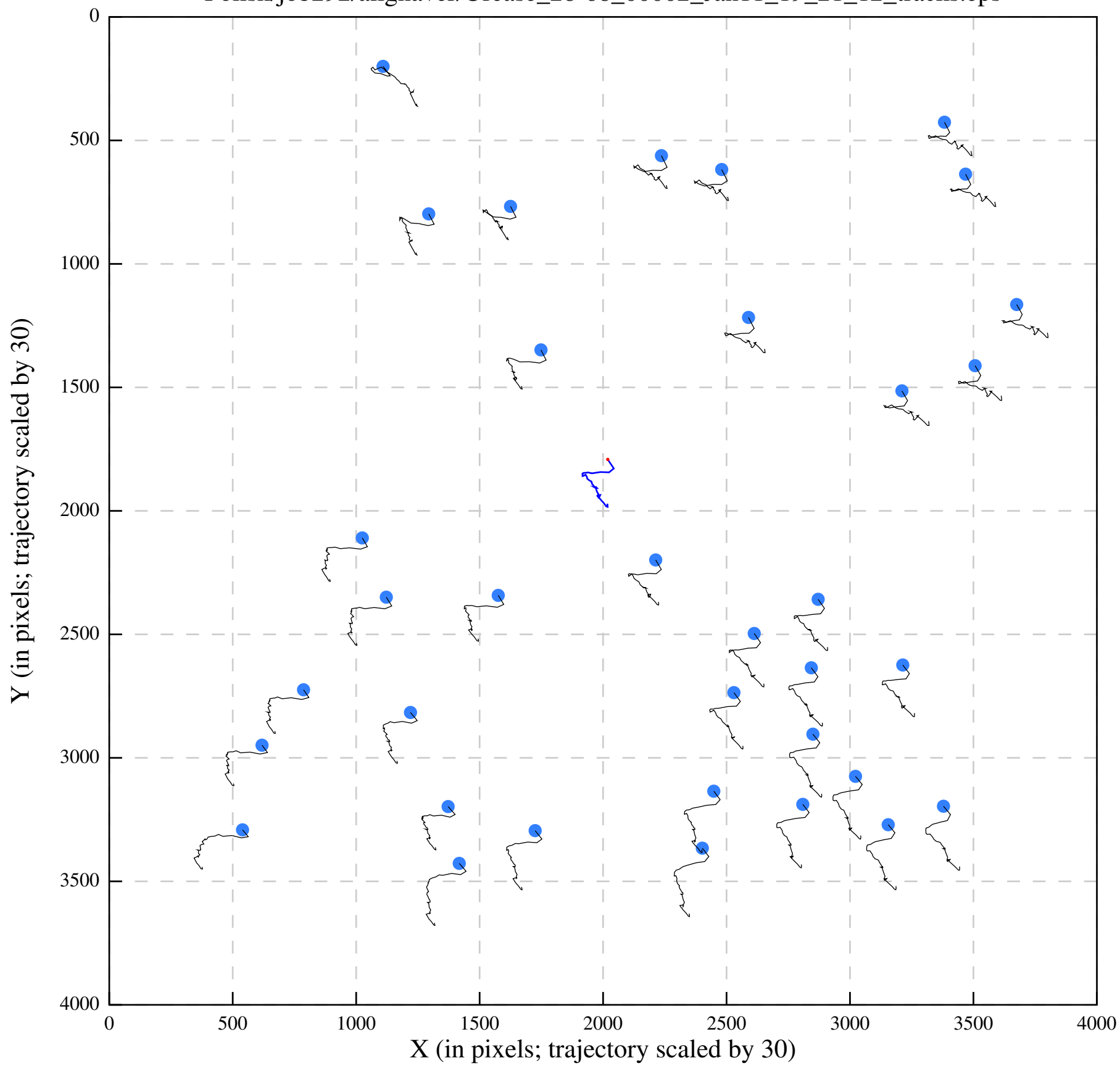
Polish/job292/alignaver/Urease_28-68_00002_Jan11_19_21_12_tracks.eps
