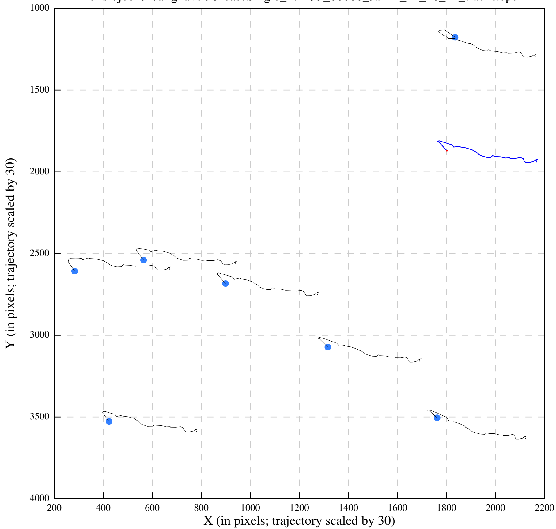
Polish/job292/alignaver/UreaseSingle_47-299_00000_Jan14_11_16_42_tracks.eps
