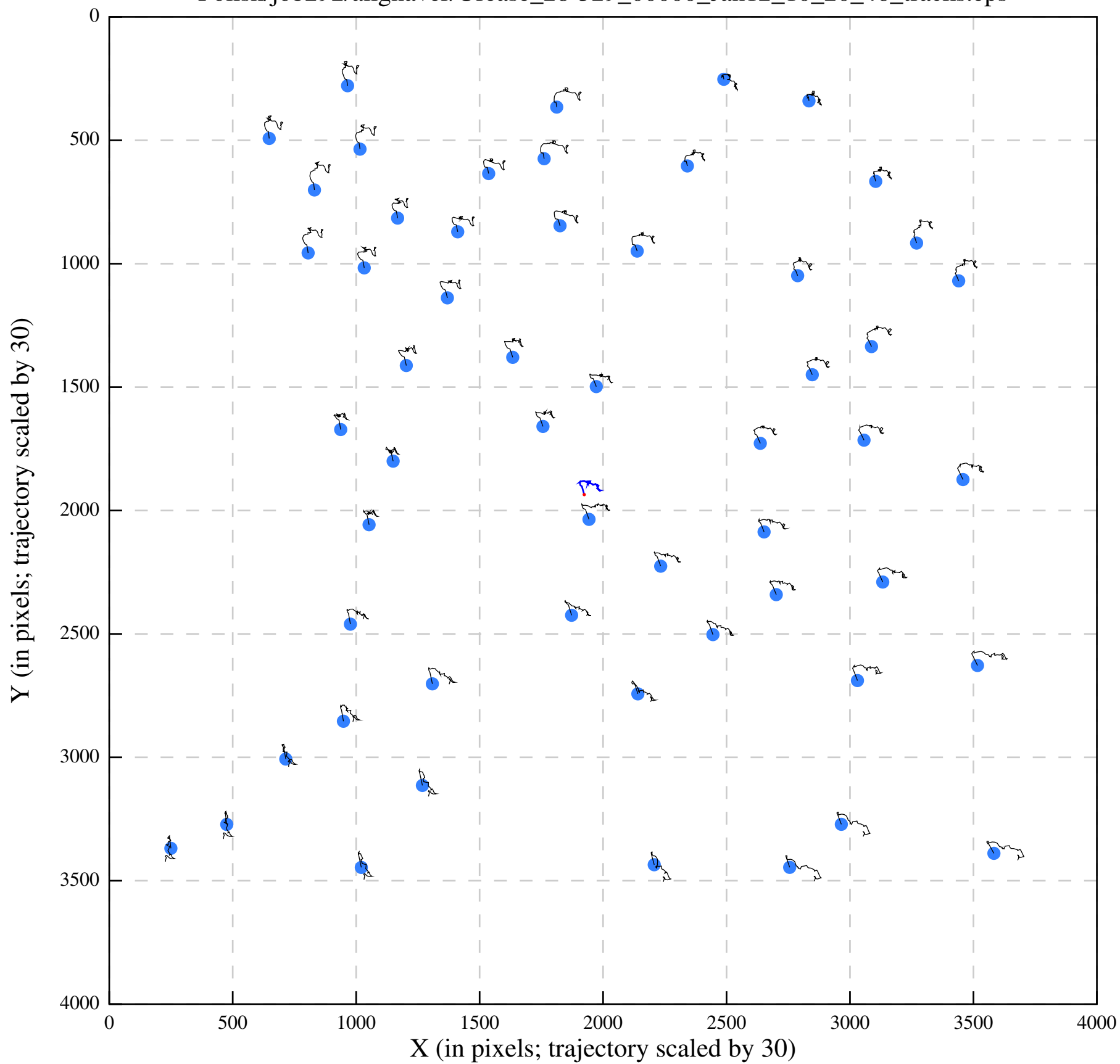
Polish/job292/alignaver/Urease_28-529_00000_Jan12_10_20_46_tracks.eps
