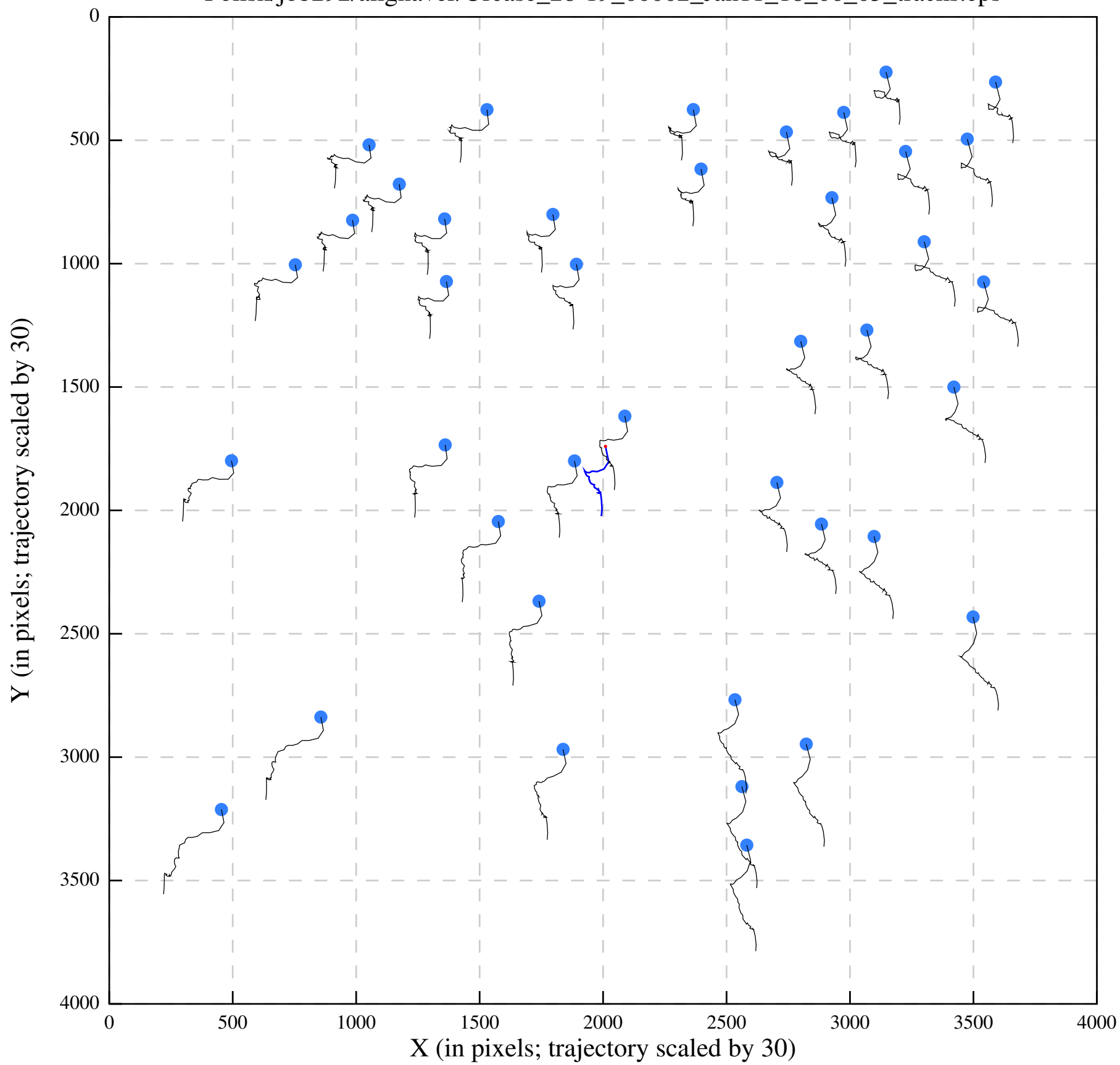
Polish/job292/alignaver/Urease_28-19_00002_Jan11_18_06_05_tracks.eps
