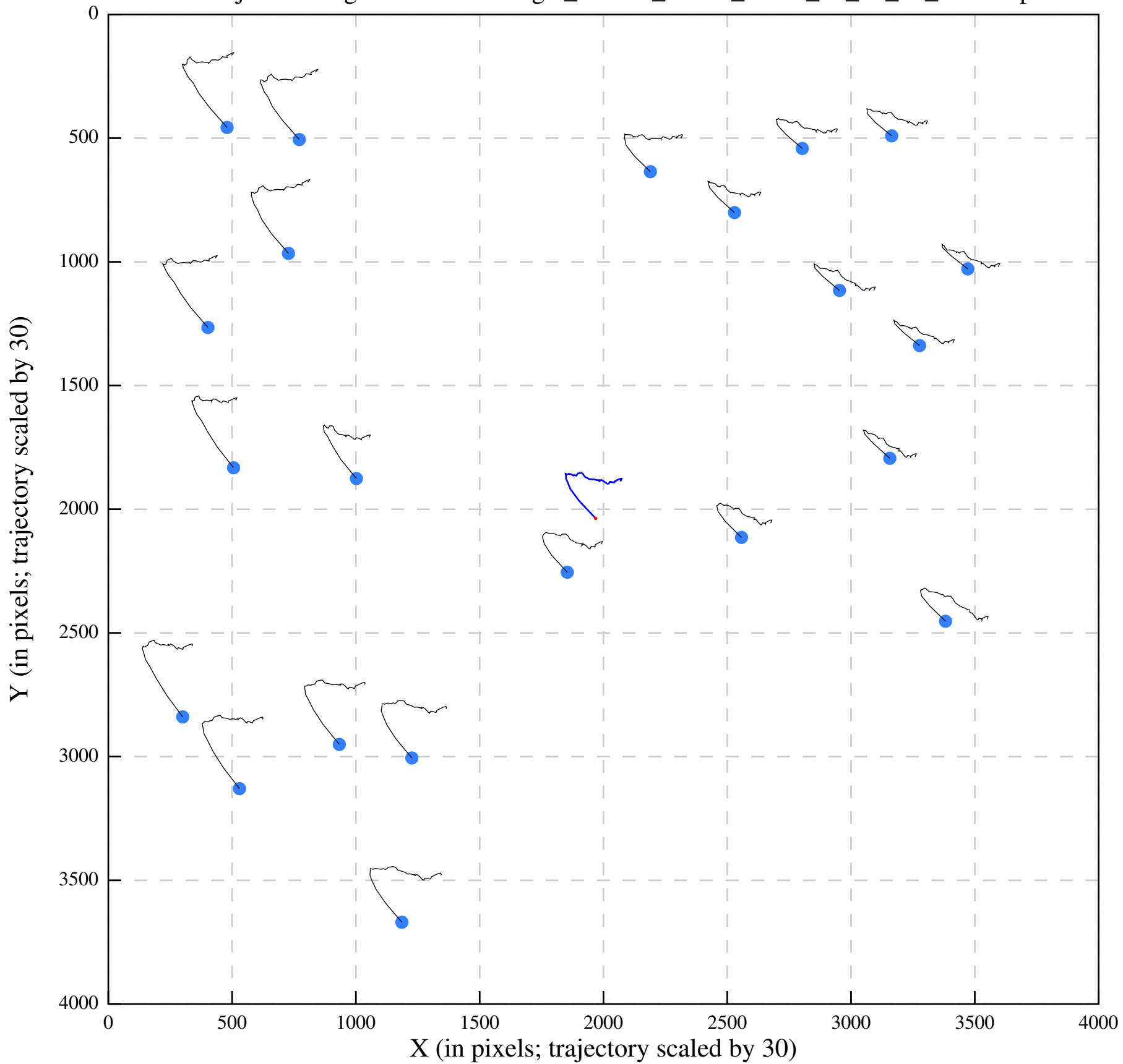
Polish/job292/alignaver/UreaseSingle_47-297_00000_Jan14_11_15_22_tracks.eps
