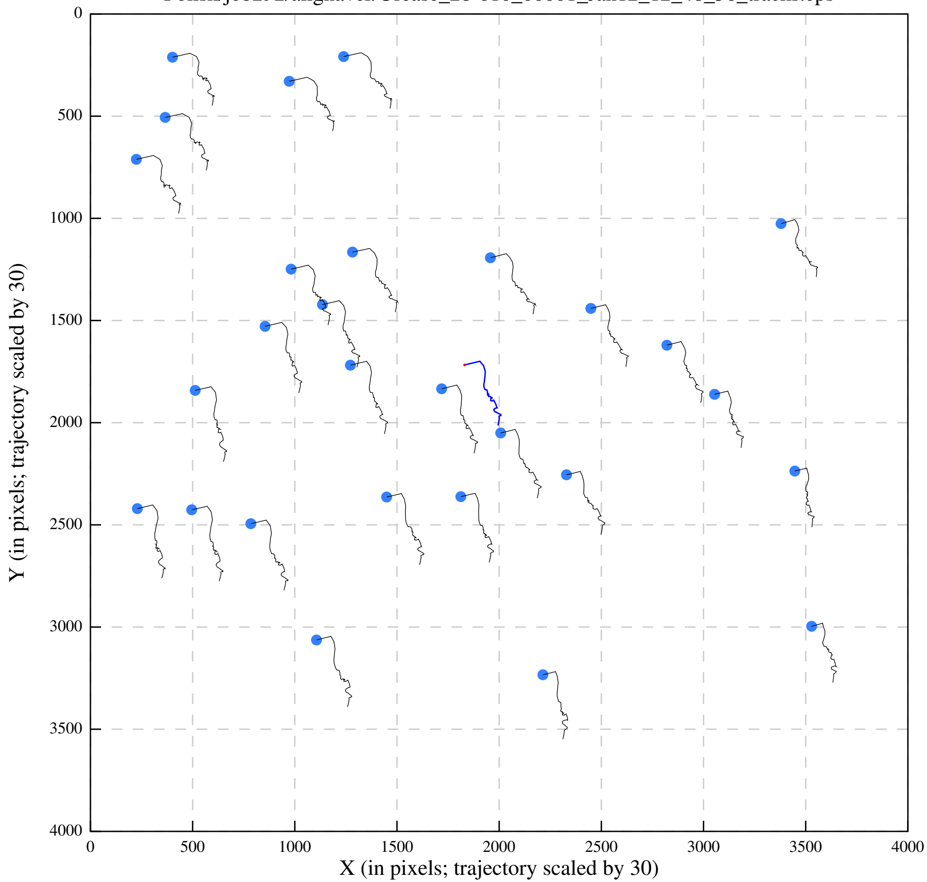
Polish/job292/alignaver/Urease_28-610_00001_Jan12_12_48_56_tracks.eps
