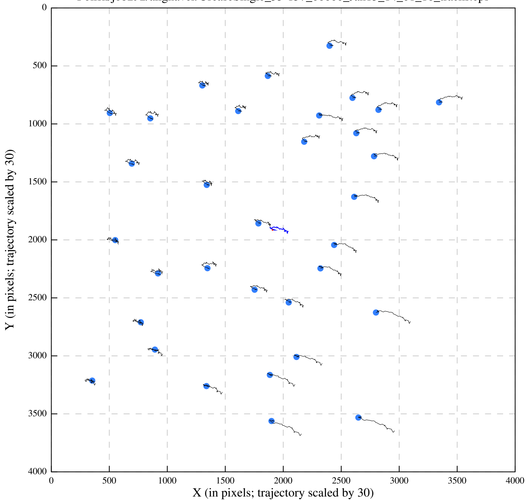
Polish/job292/alignaver/UreaseSingle_35-157_00000_Jan13_14_01_16_tracks.eps
