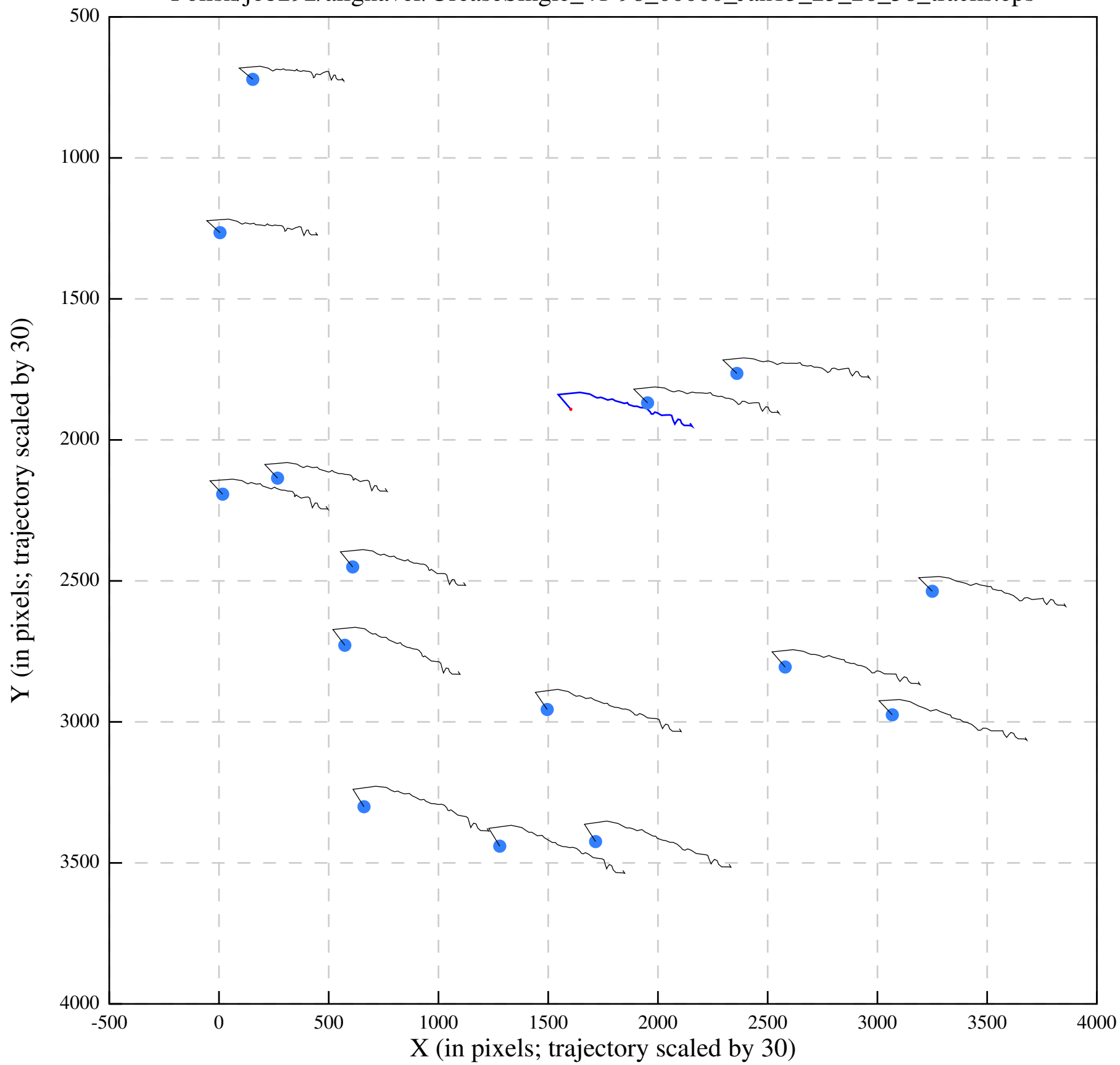
Polish/job292/alignaver/UreaseSingle_41-98_00000_Jan13_23_26_58_tracks.eps
