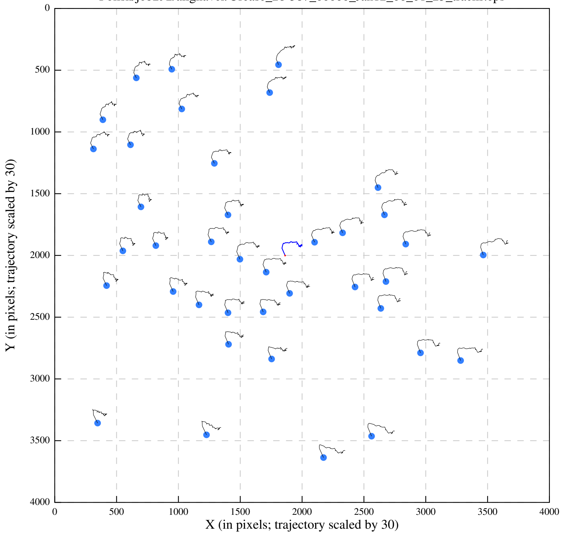
Polish/job292/alignaver/Urease_28-387_00000_Jan12_06_01_23_tracks.eps
