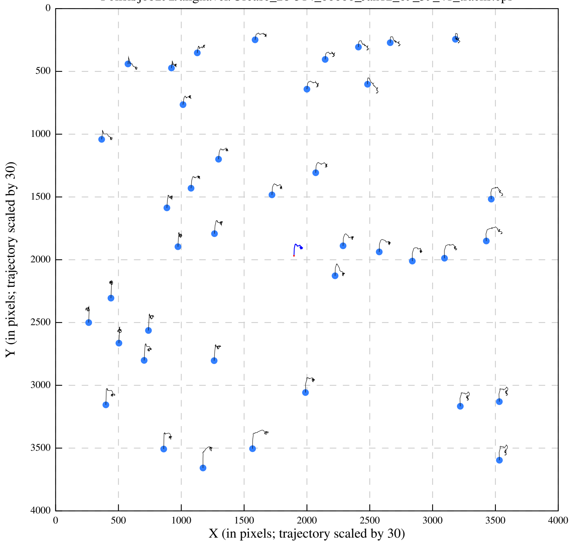
Polish/job292/alignaver/Urease_28-514_00000_Jan12_09_59_41_tracks.eps
