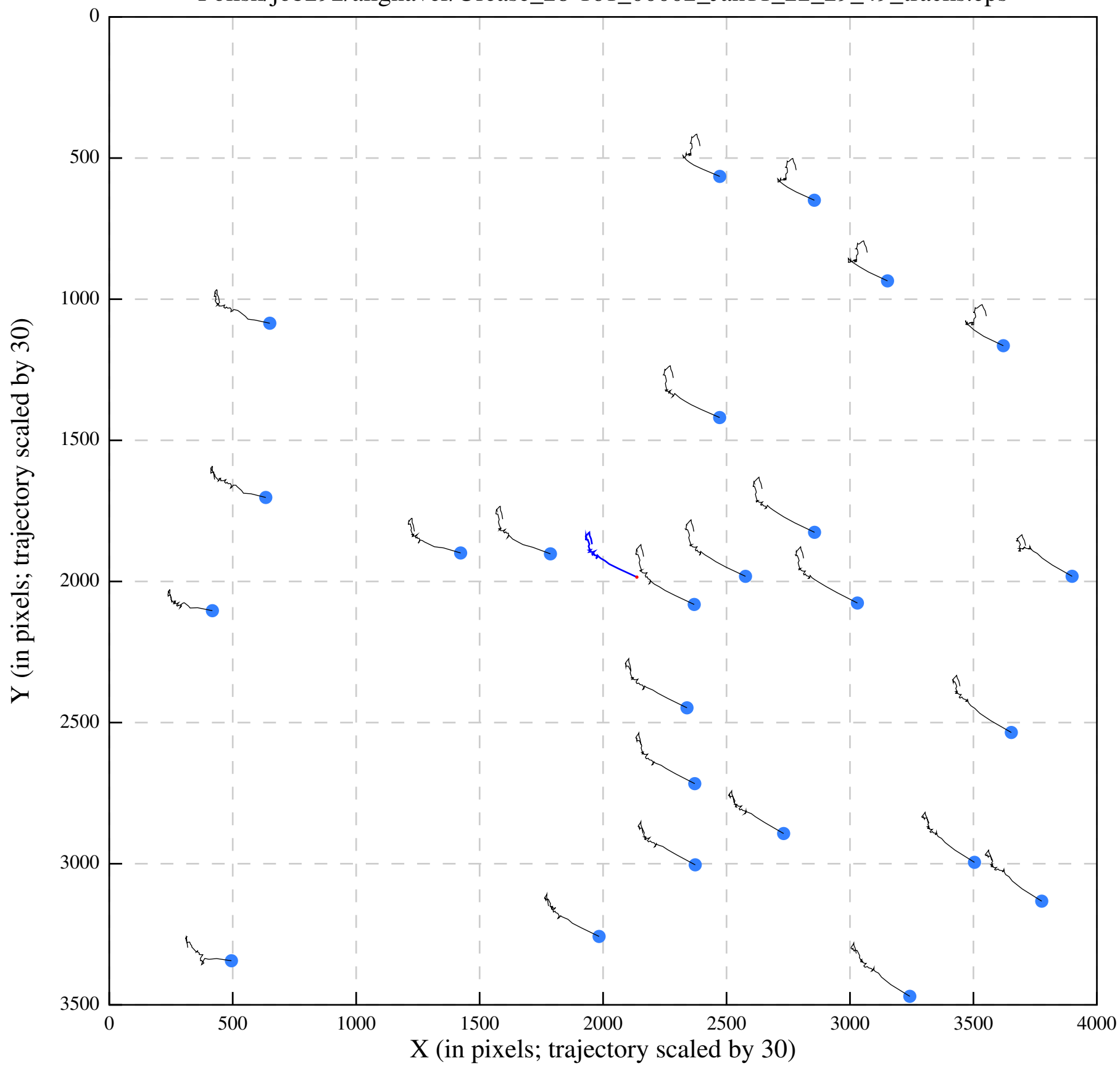
Polish/job292/alignaver/Urease_28-161_00002_Jan11_22_29_49_tracks.eps
