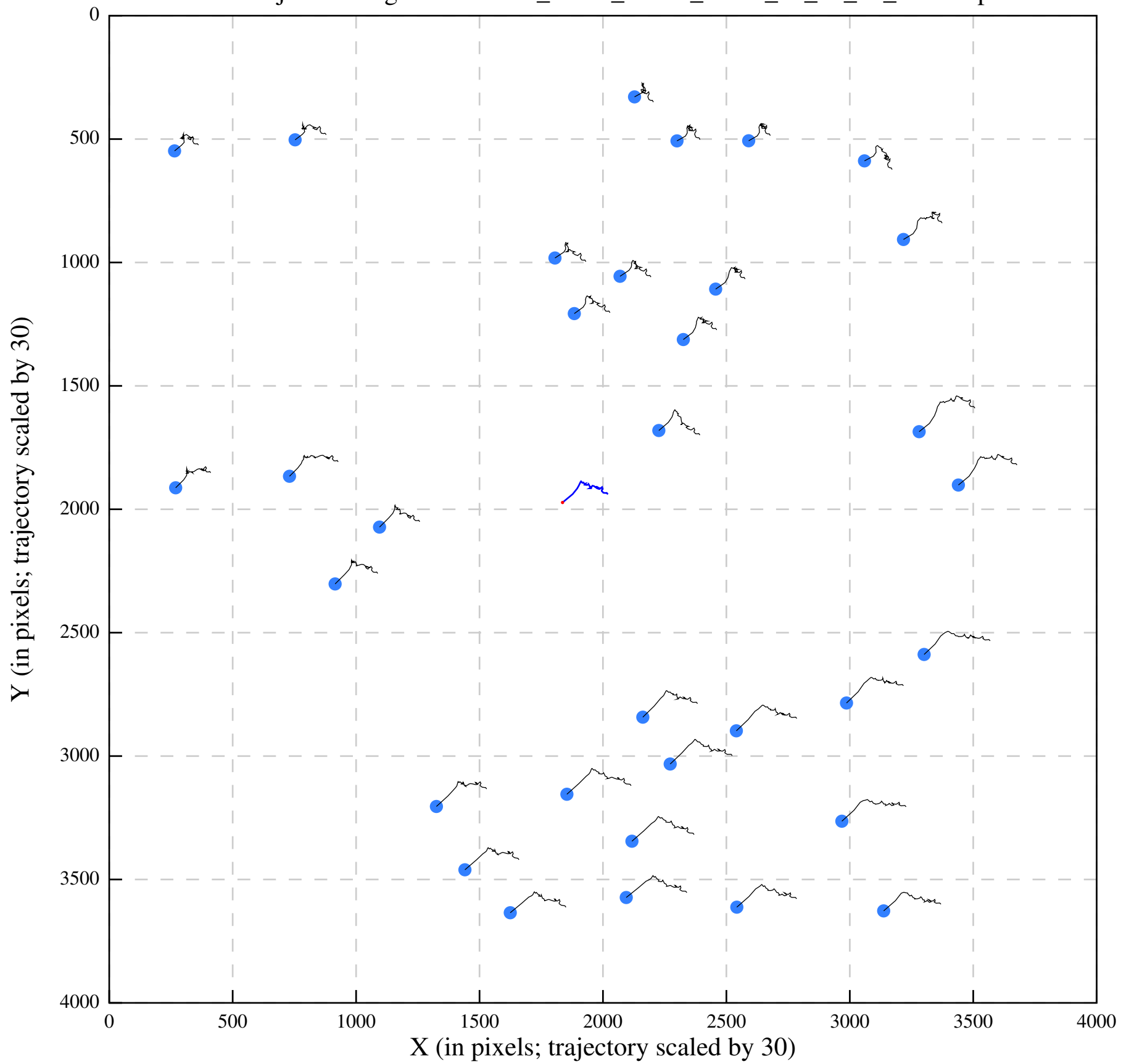
Polish/job292/alignaver/Urease_28-53_00000_Jan11_18_59_07_tracks.eps
