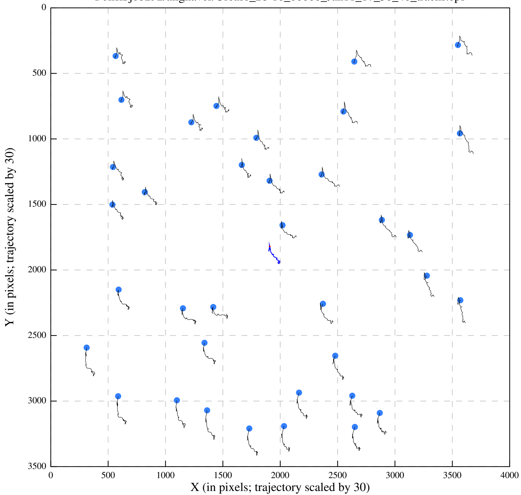
Polish/job292/alignaver/Urease_28-10_00000_Jan11_17_50_40_tracks.eps
