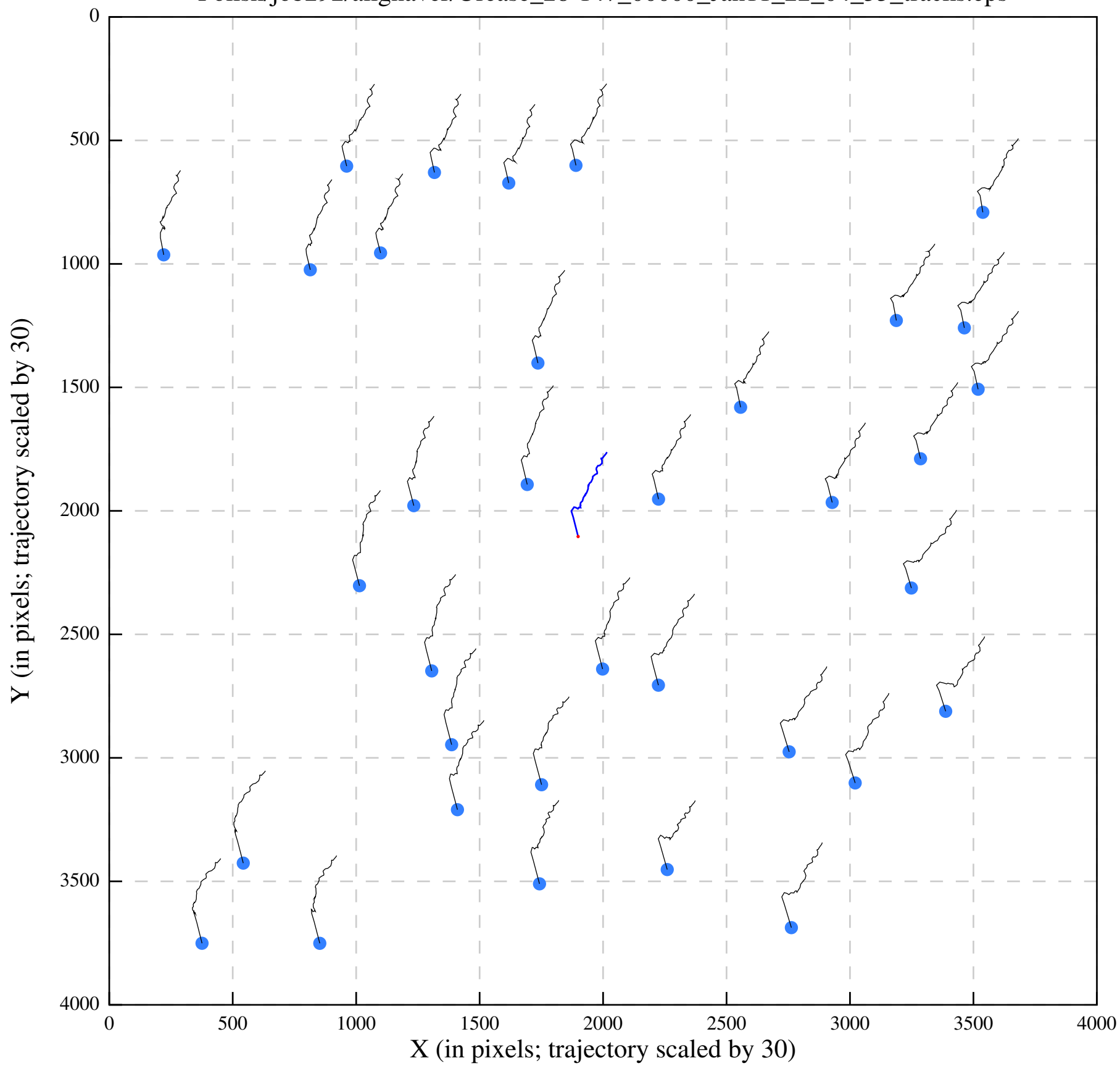
Polish/job292/alignaver/Urease_28-147_00000_Jan11_22_04_55_tracks.eps
