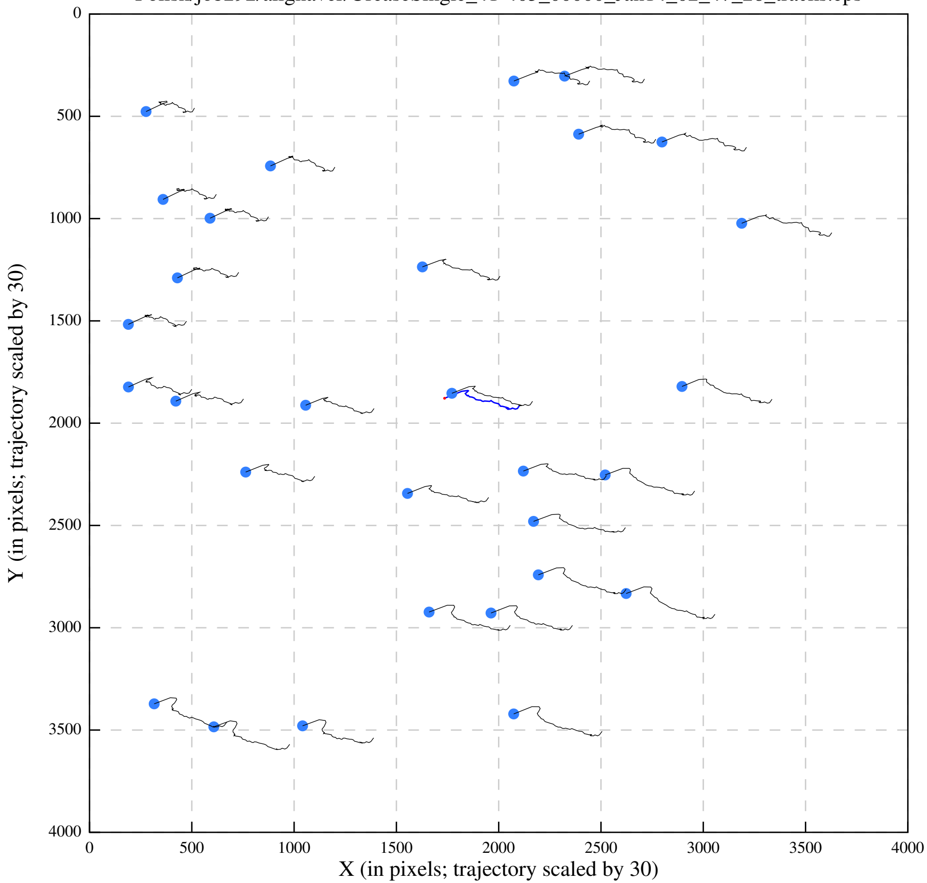
Polish/job292/alignaver/UreaseSingle_41-405_00000_Jan14_02_47_28_tracks.eps
