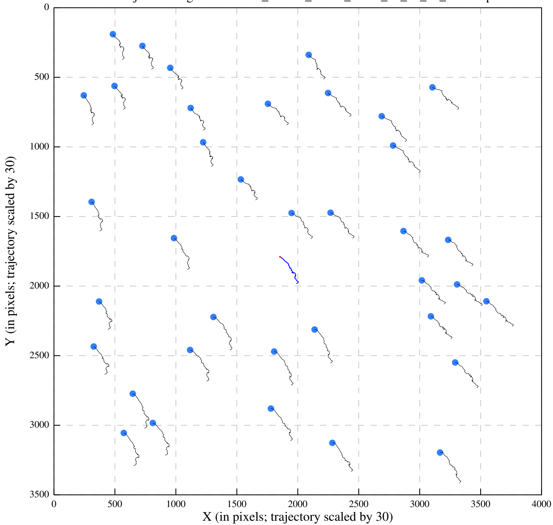
Polish/job292/alignaver/Urease_28-304_00001_Jan12_03_15_01_tracks.eps
