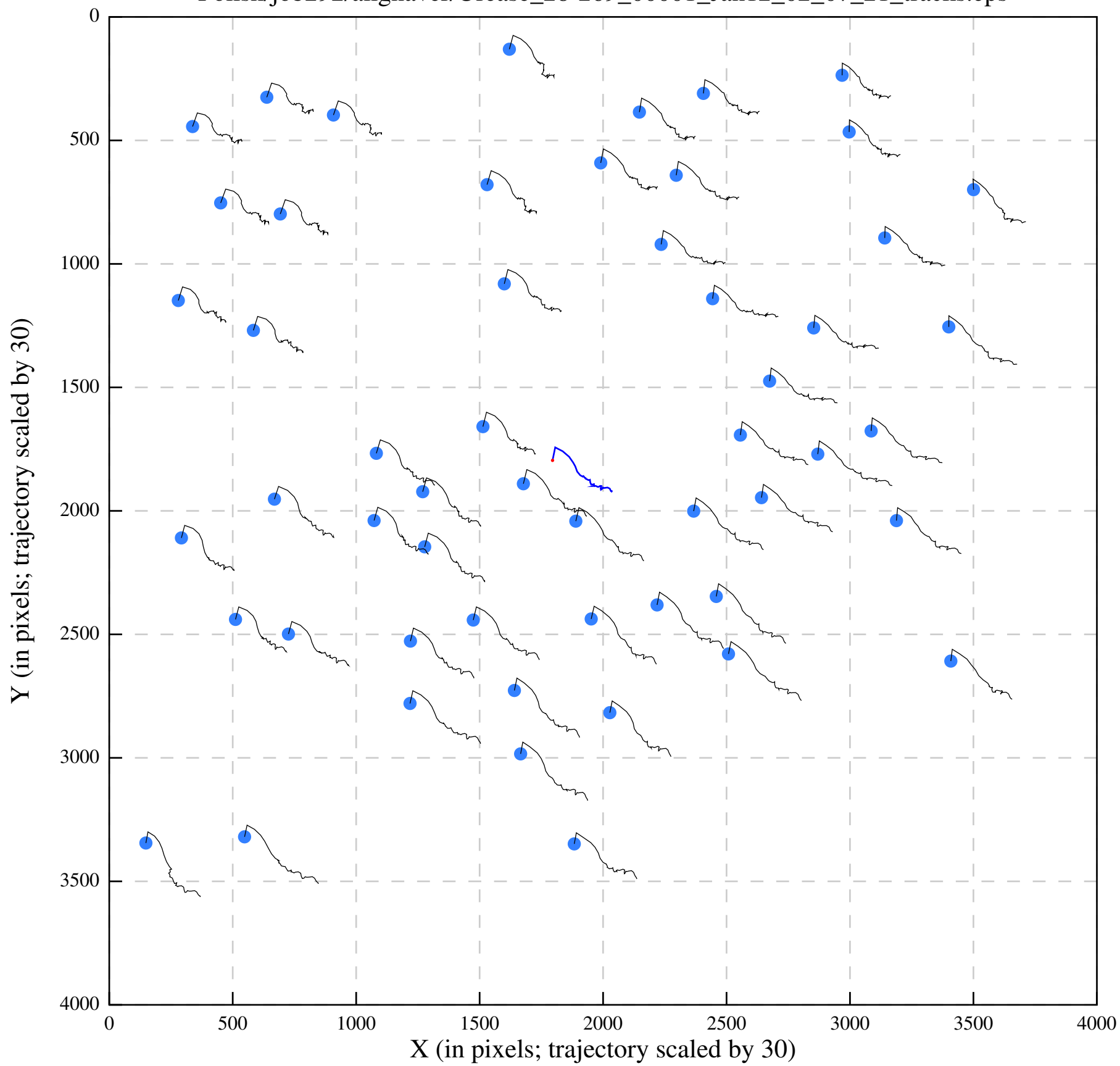
Polish/job292/alignaver/Urease_28-269_00001_Jan12_02_07_21_tracks.eps
