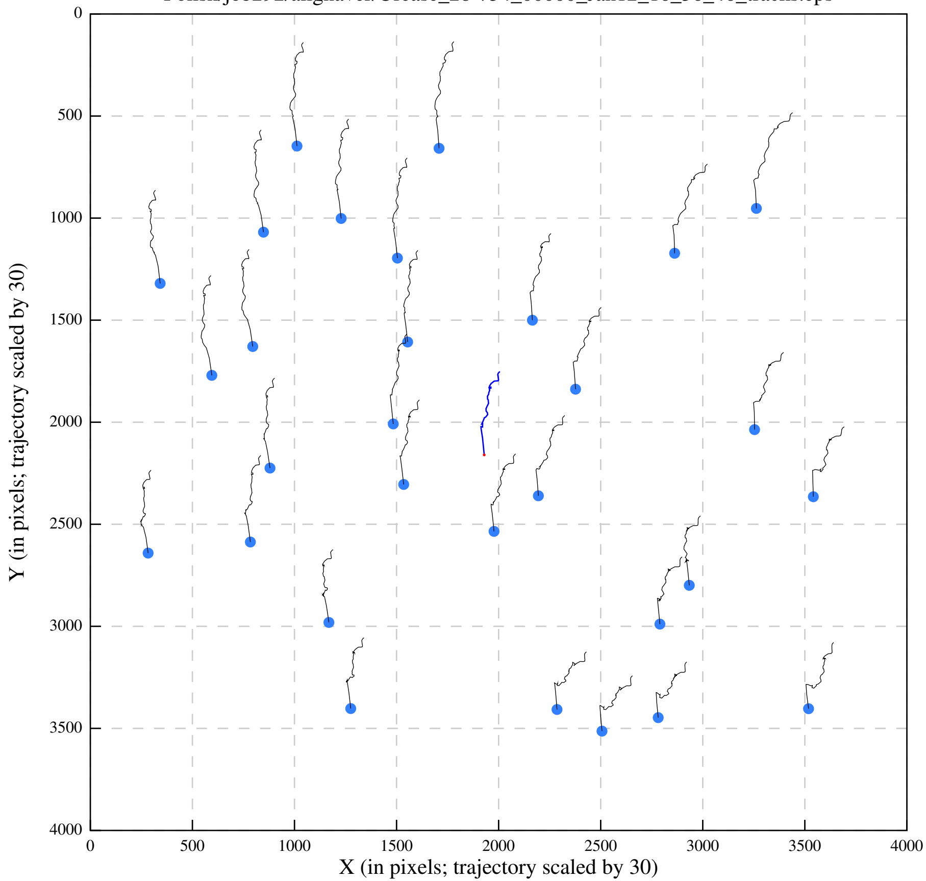
Polish/job292/alignaver/Urease_28-734_00000_Jan12_16_36_46_tracks.eps
