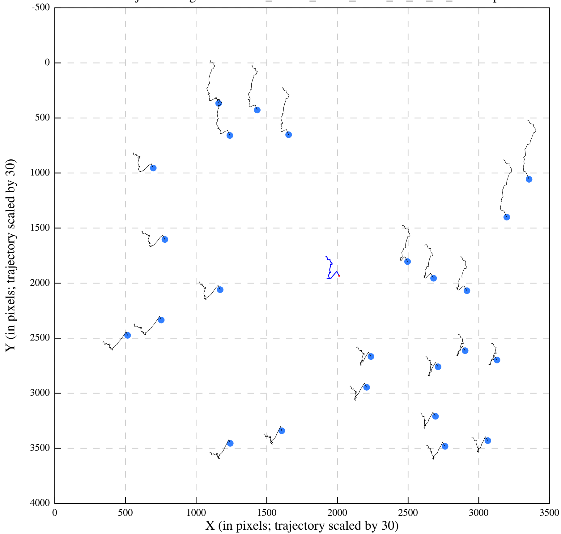
Polish/job292/alignaver/Urease_28-737_00002_Jan12_16_43_50_tracks.eps
