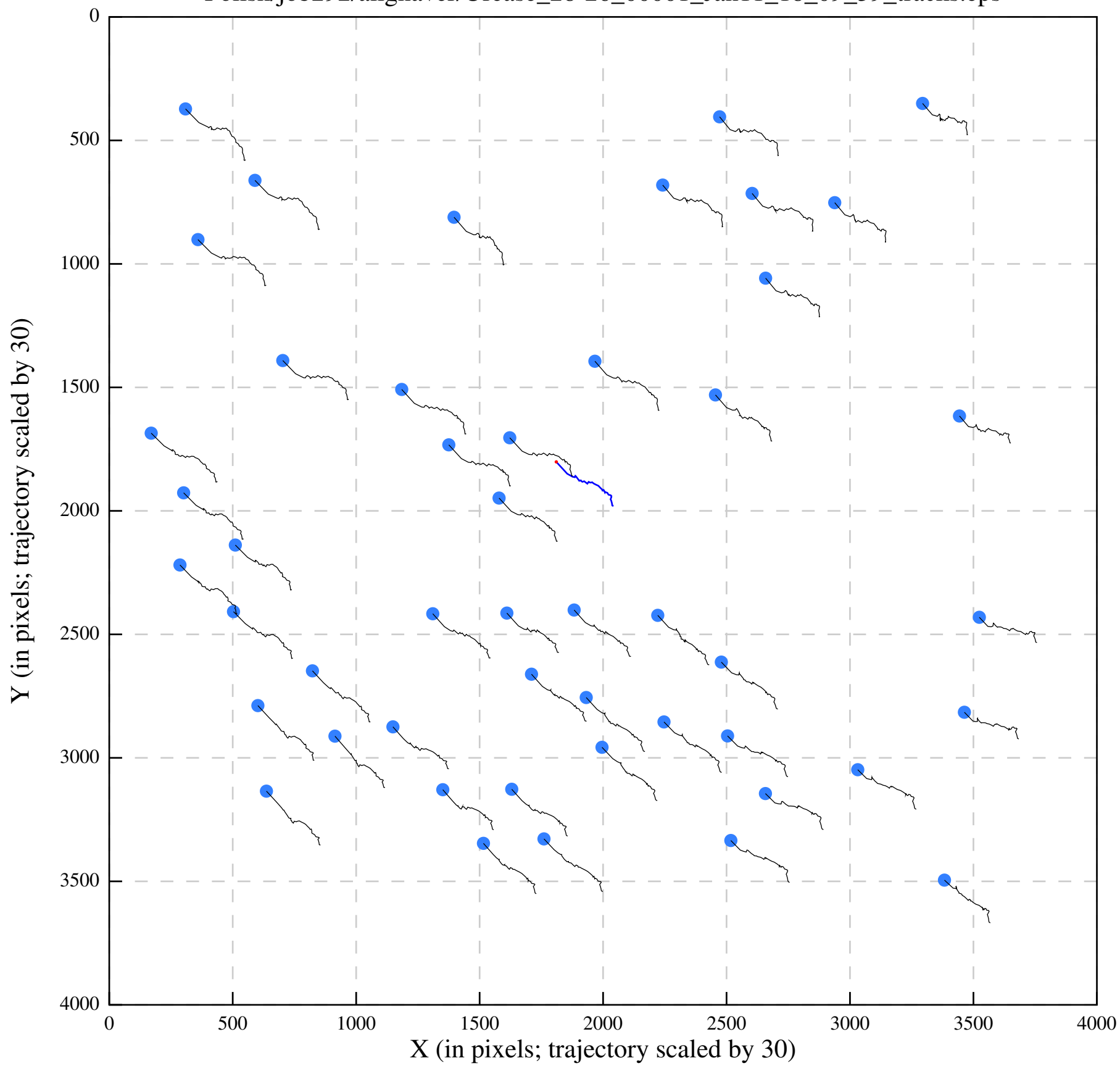
Polish/job292/alignaver/Urease_28-26_00001_Jan11_18_09_39_tracks.eps
