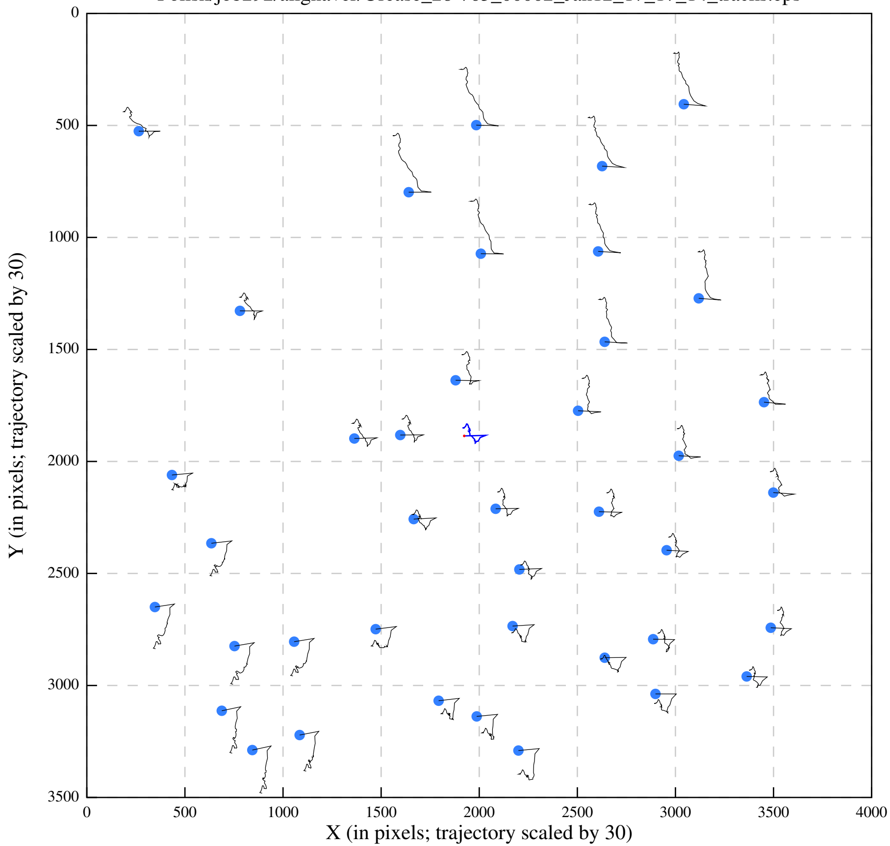
Polish/job292/alignaver/Urease_28-763_00002_Jan12_17_17_14_tracks.eps
