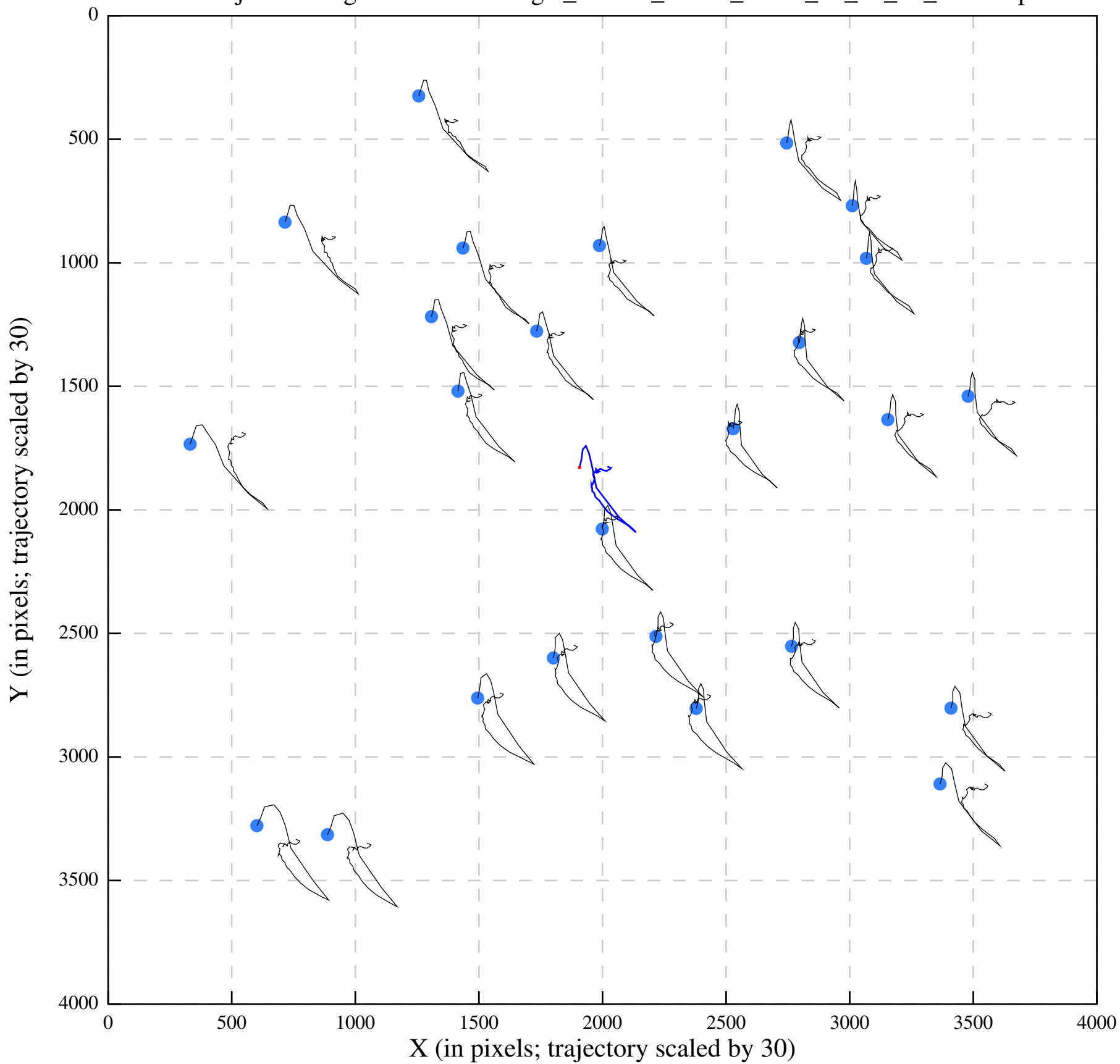
Polish/job292/alignaver/UreaseSingle_47-639_00000_Jan14_15_20_35_tracks.eps
