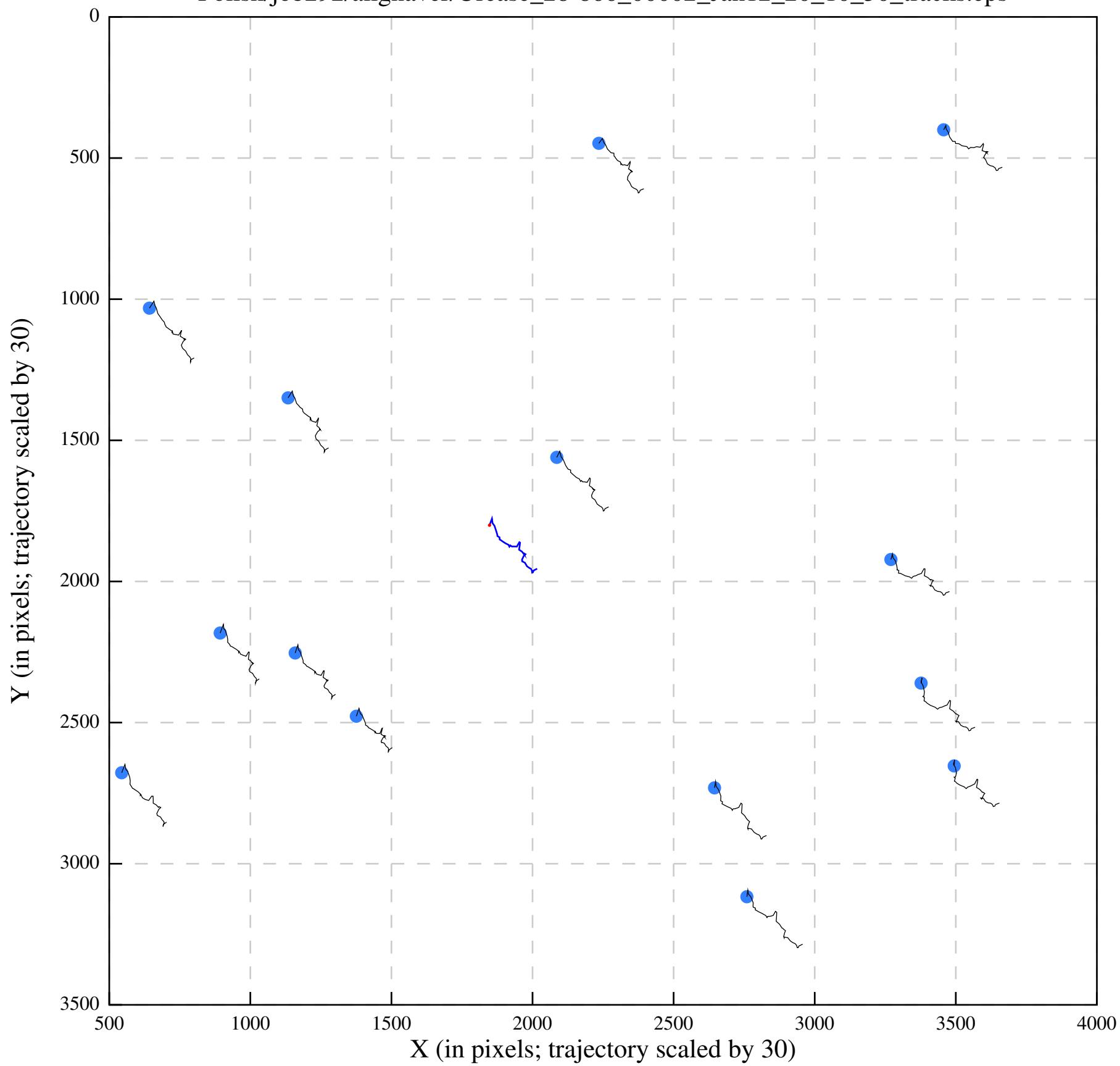
Polish/job292/alignaver/Urease_28-866_00002_Jan12_20_10_50_tracks.eps
