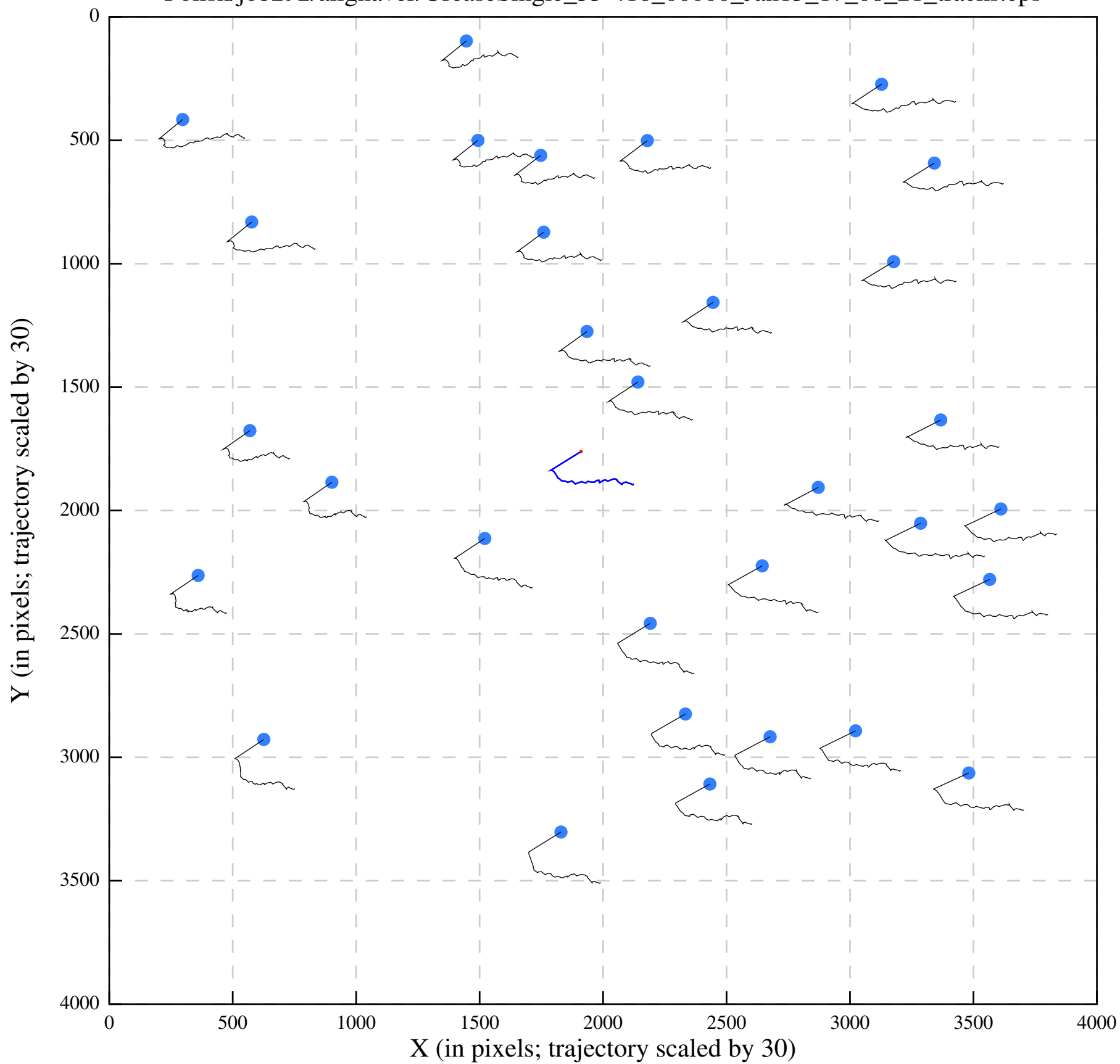
Polish/job292/alignaver/UreaseSingle_35-416_00000_Jan13_17_08_21_tracks.eps
