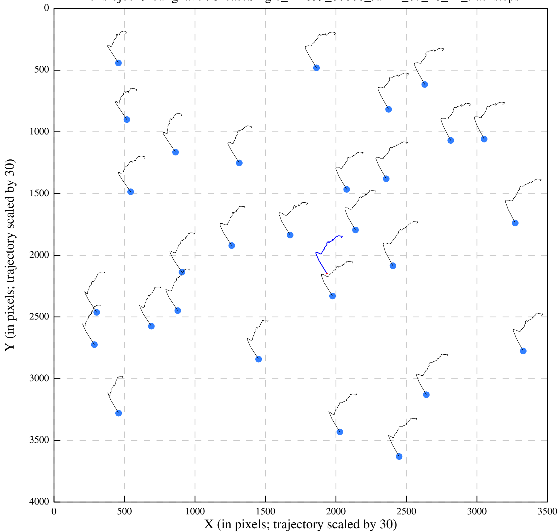
Polish/job292/alignaver/UreaseSingle_41-839_00000_Jan14_07_48_42_tracks.eps
