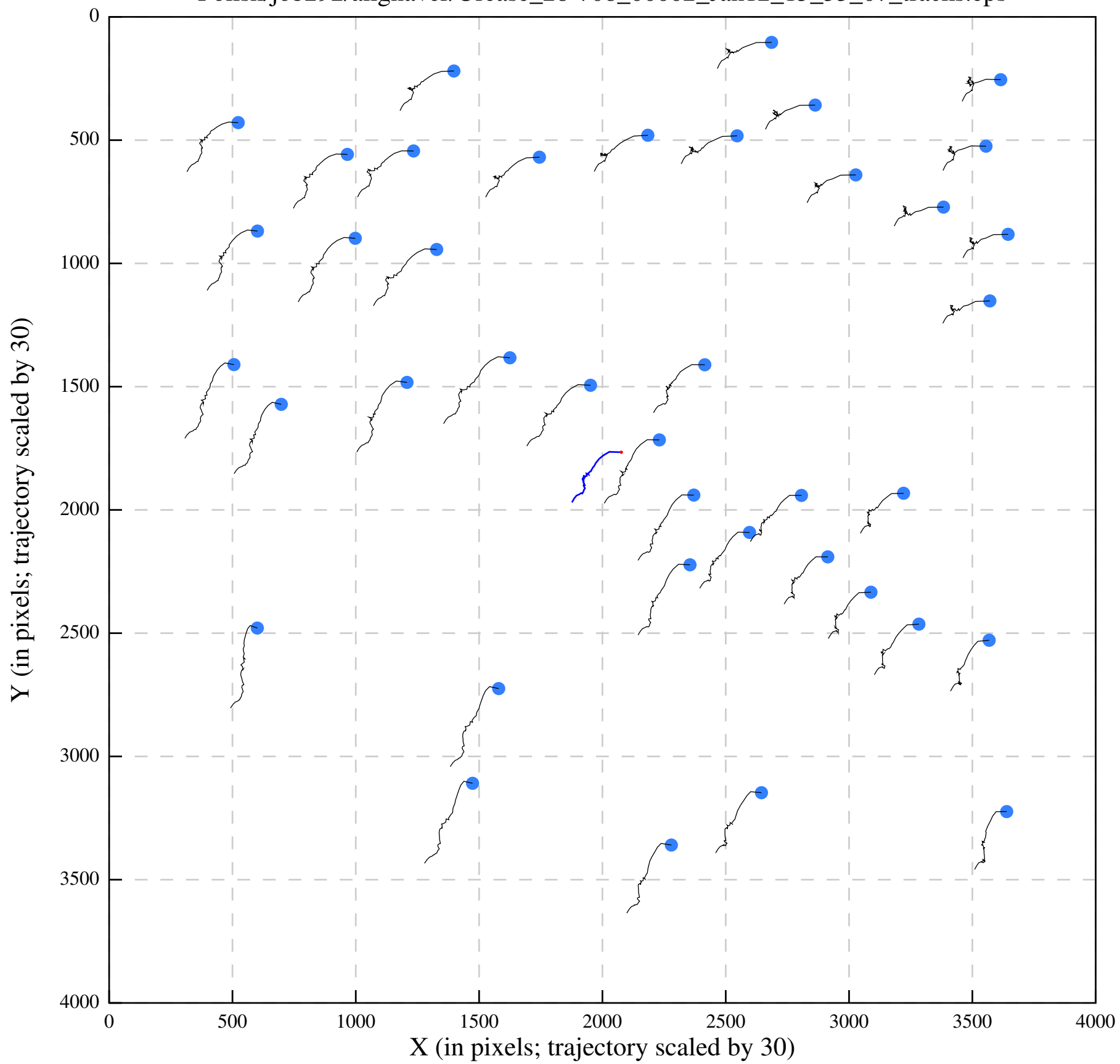
Polish/job292/alignaver/Urease_28-708_00002_Jan12_15_33_07_tracks.eps
