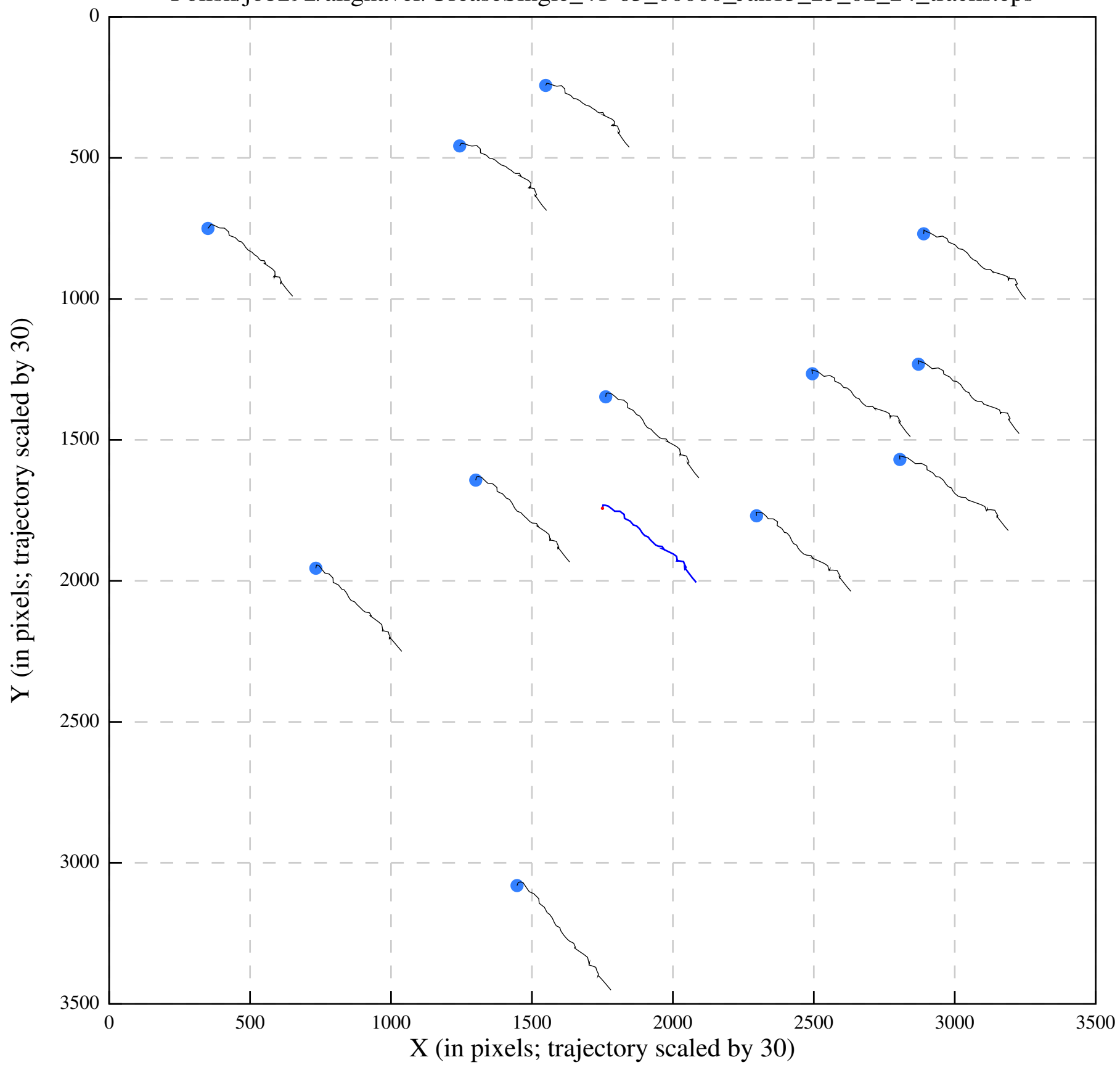
Polish/job292/alignaver/UreaseSingle_41-63_00000_Jan13_23_02_24_tracks.eps
