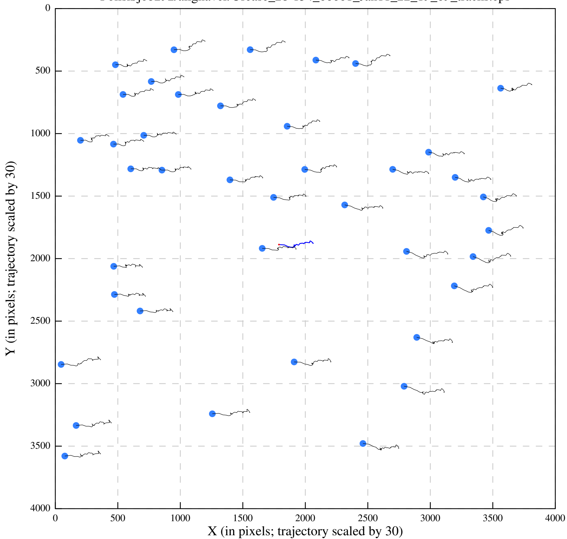
Polish/job292/alignaver/Urease_28-154_00001_Jan11_22_19_09_tracks.eps
