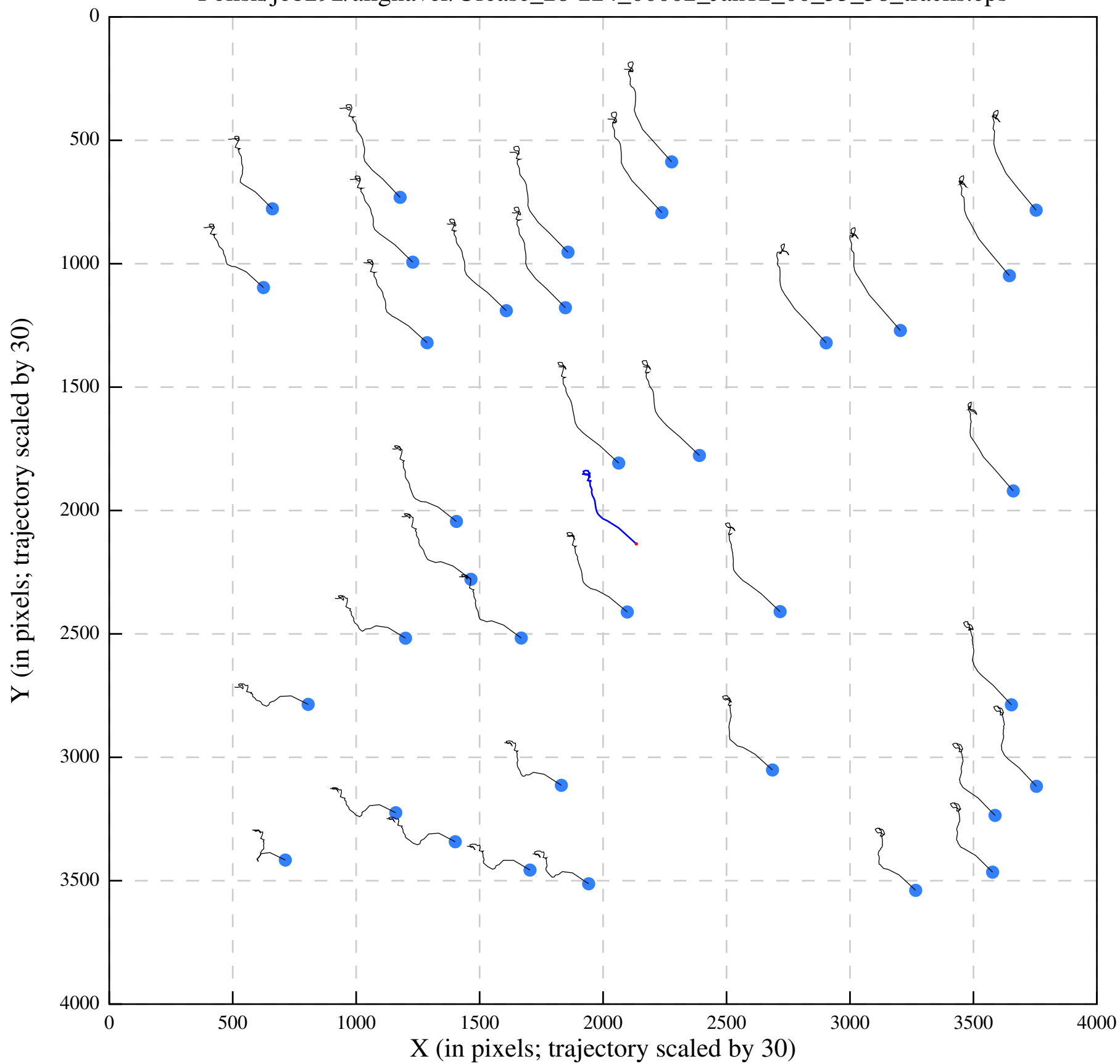
Polish/job292/alignaver/Urease_28-224_00002_Jan12_00_33_38_tracks.eps
