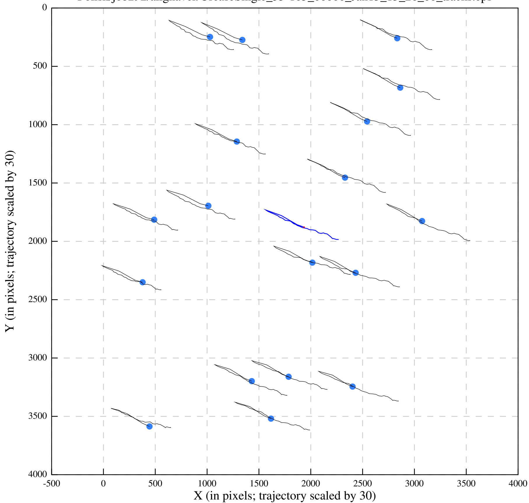
Polish/job292/alignaver/UreaseSingle_35-105_00000_Jan13_13_26_00_tracks.eps
