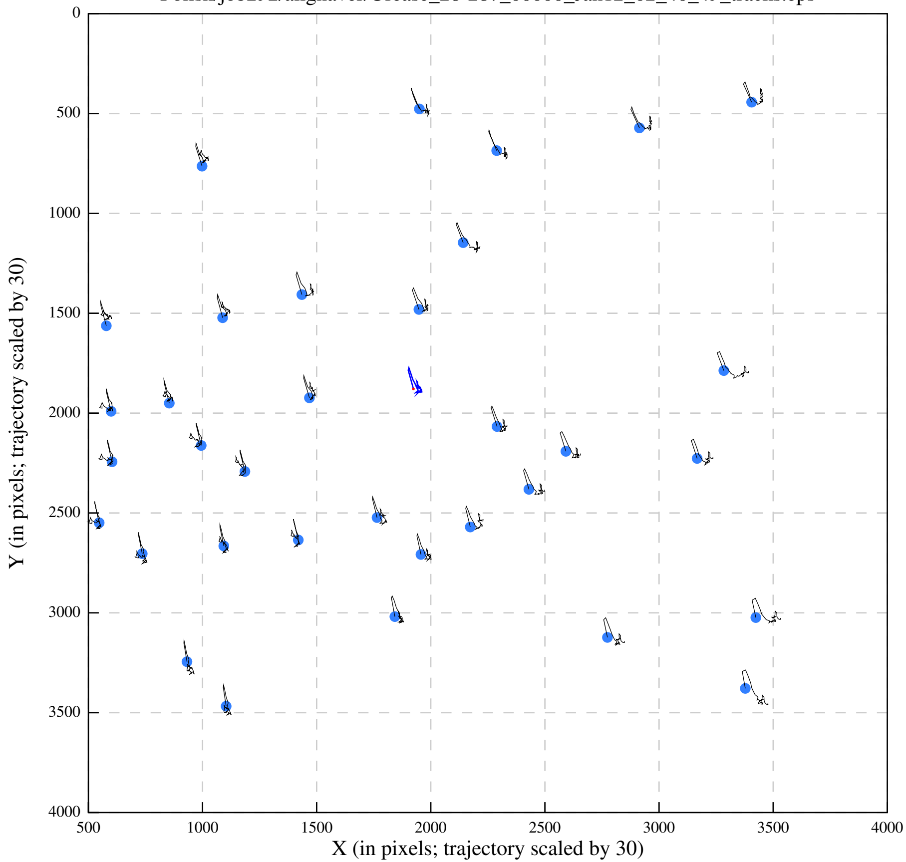
Polish/job292/alignaver/Urease_28-287_00000_Jan12_02_40_49_tracks.eps
