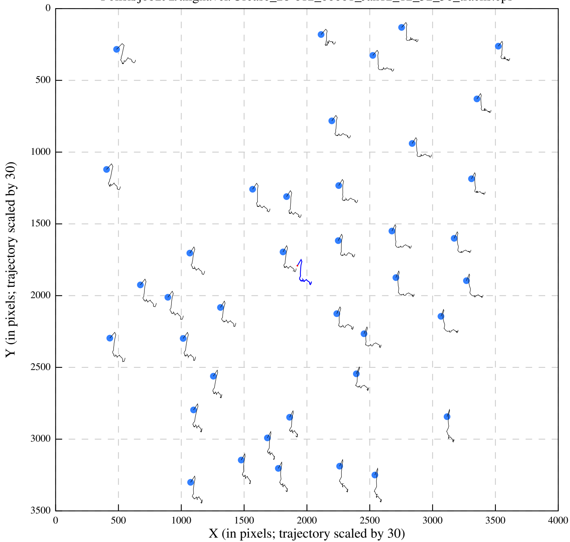
Polish/job292/alignaver/Urease_28-612_00001_Jan12_12_52_56_tracks.eps
