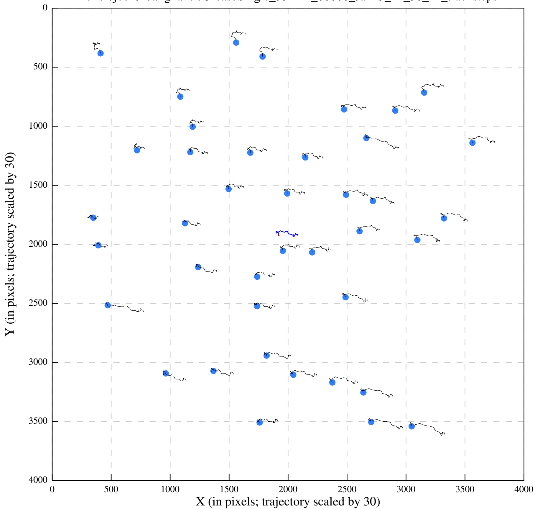
Polish/job292/alignaver/UreaseSingle_35-212_00000_Jan13_14_38_14_tracks.eps
