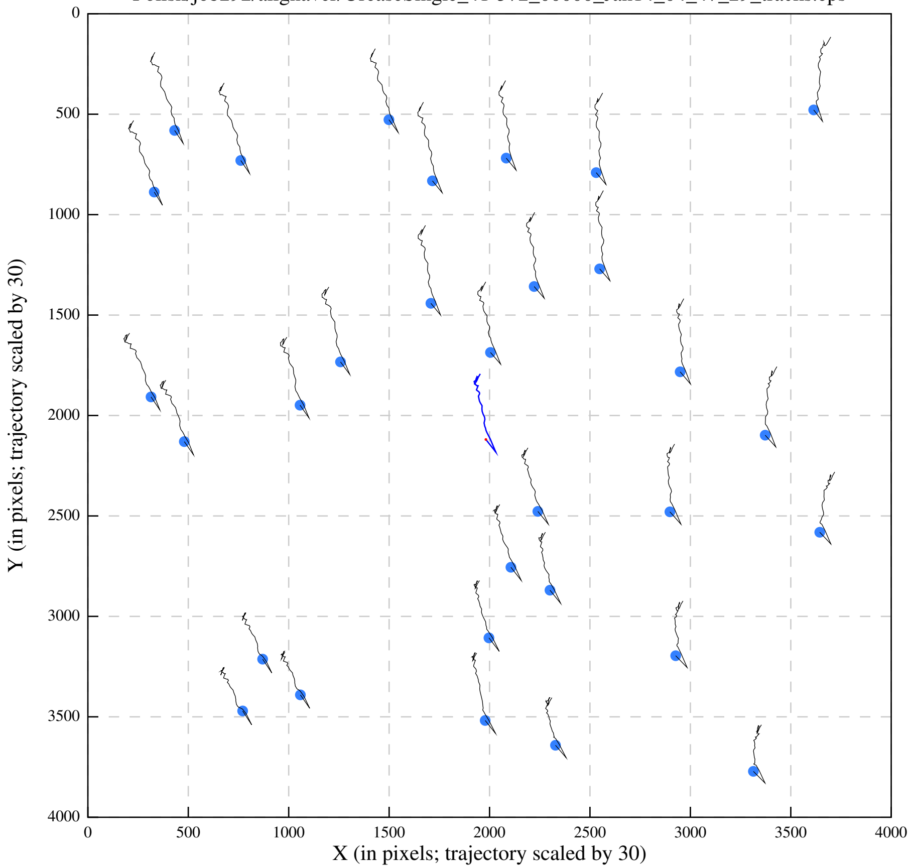
Polish/job292/alignaver/UreaseSingle_41-572_00000_Jan14_04_47_29_tracks.eps
