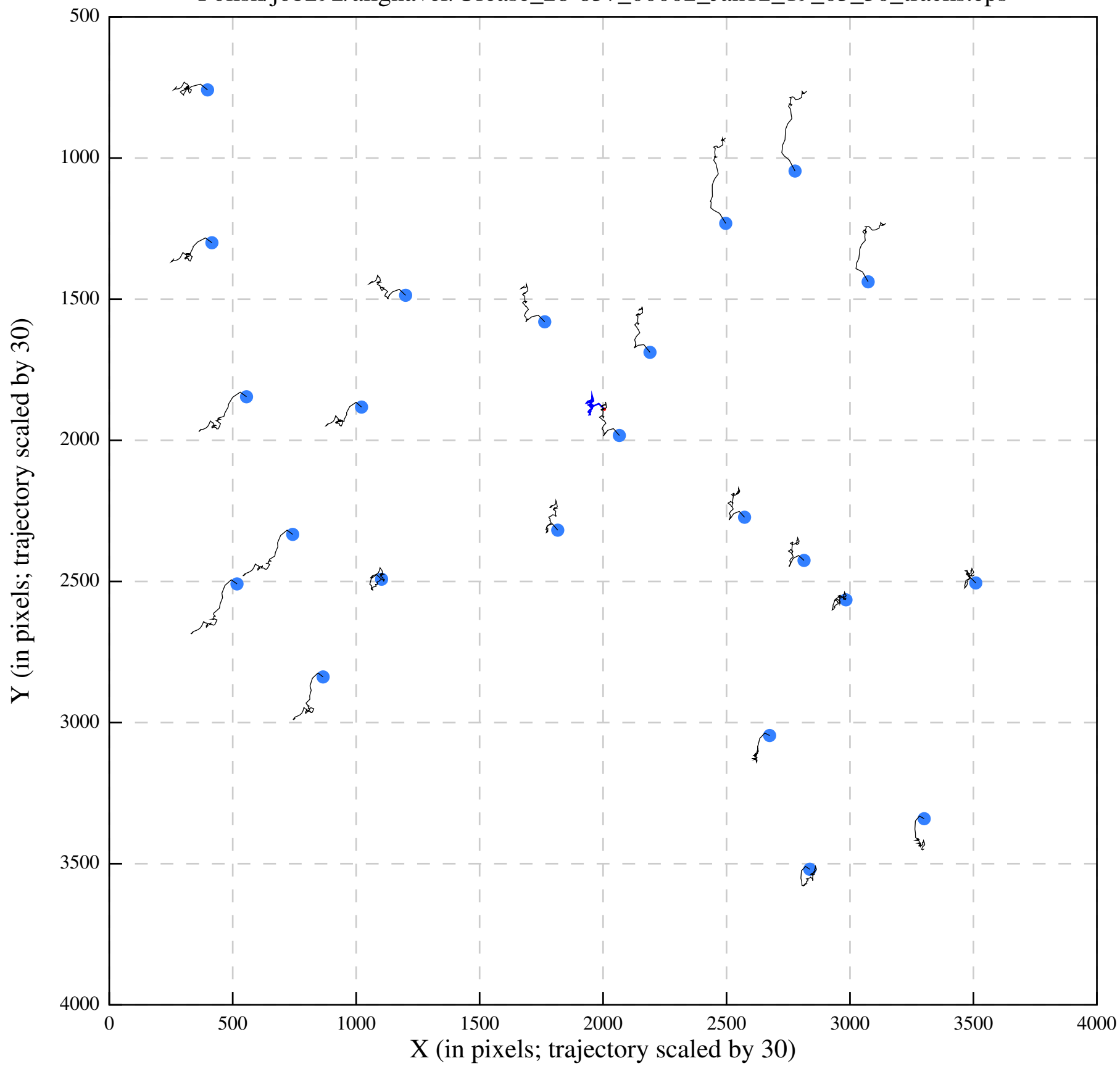
Polish/job292/alignaver/Urease_28-837_00002_Jan12_19_05_30_tracks.eps
