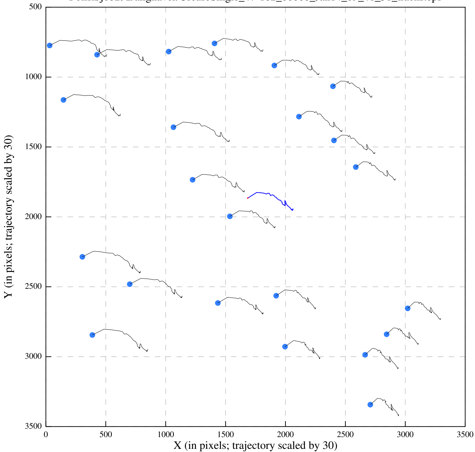
Polish/job292/alignaver/UreaseSingle_47-162_00000_Jan14_09_41_31_tracks.eps
