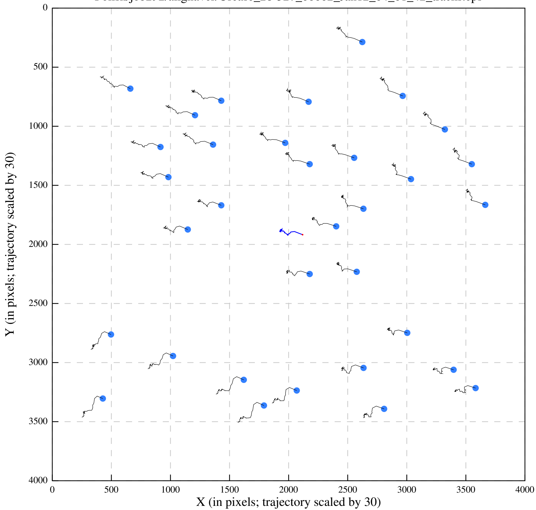
Polish/job292/alignaver/Urease_28-327_00002_Jan12_04_01_42_tracks.eps
