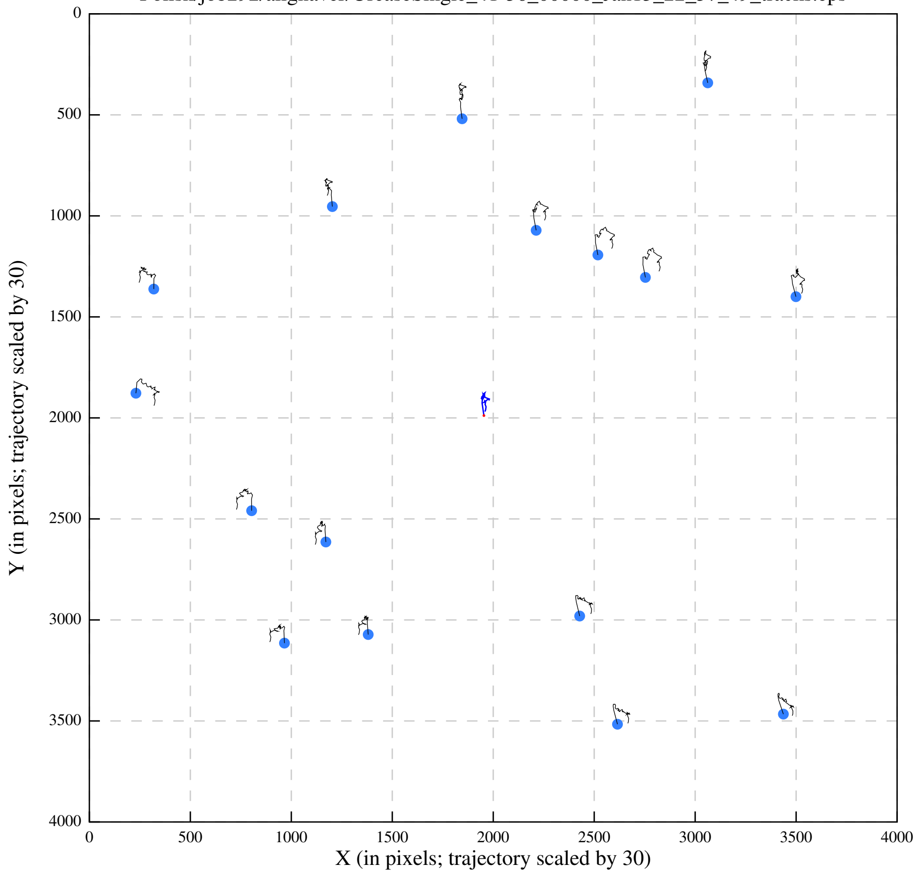
Polish/job292/alignaver/UreaseSingle_41-56_00000_Jan13_22_57_49_tracks.eps
