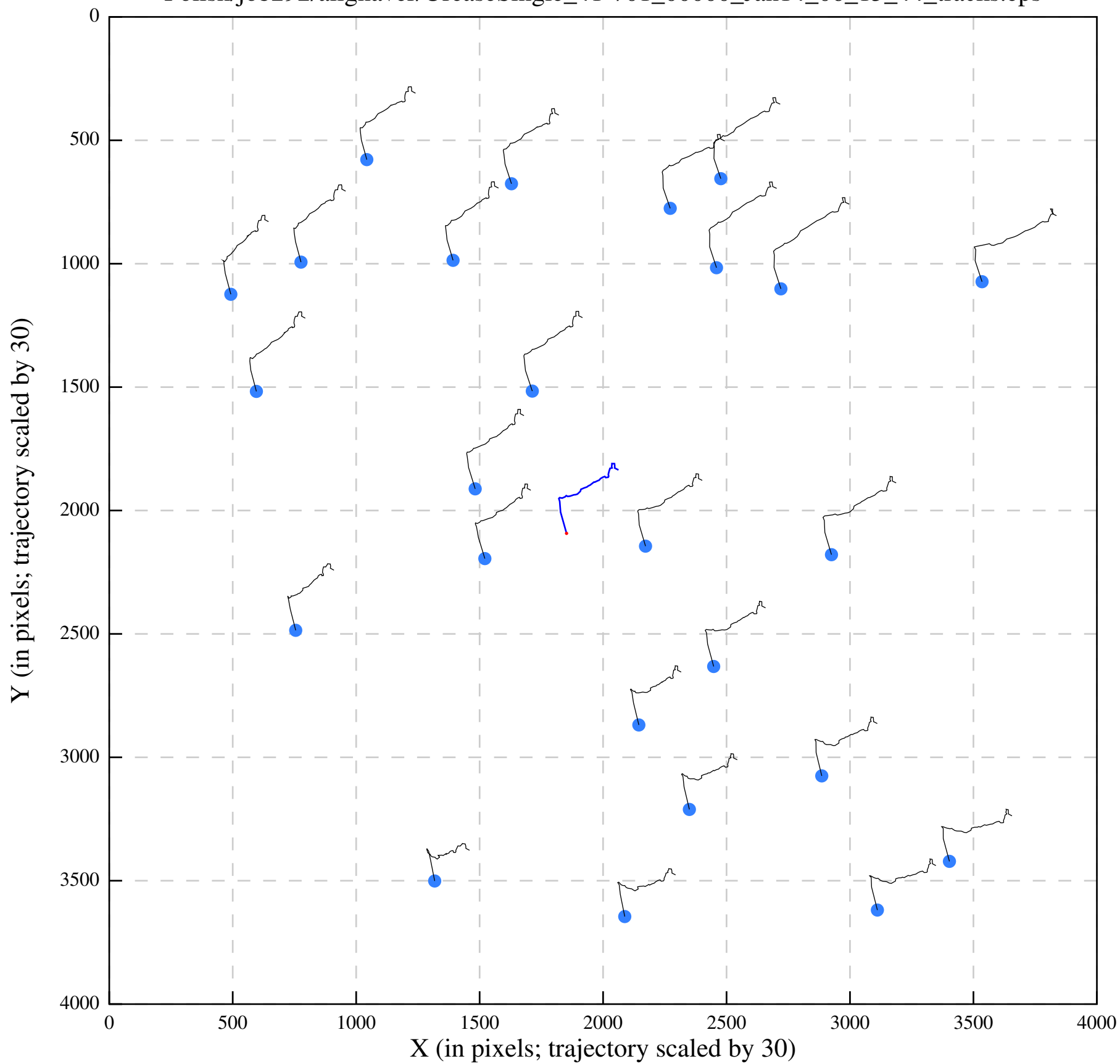
Polish/job292/alignaver/UreaseSingle_41-701_00000_Jan14_06_15_44_tracks.eps
