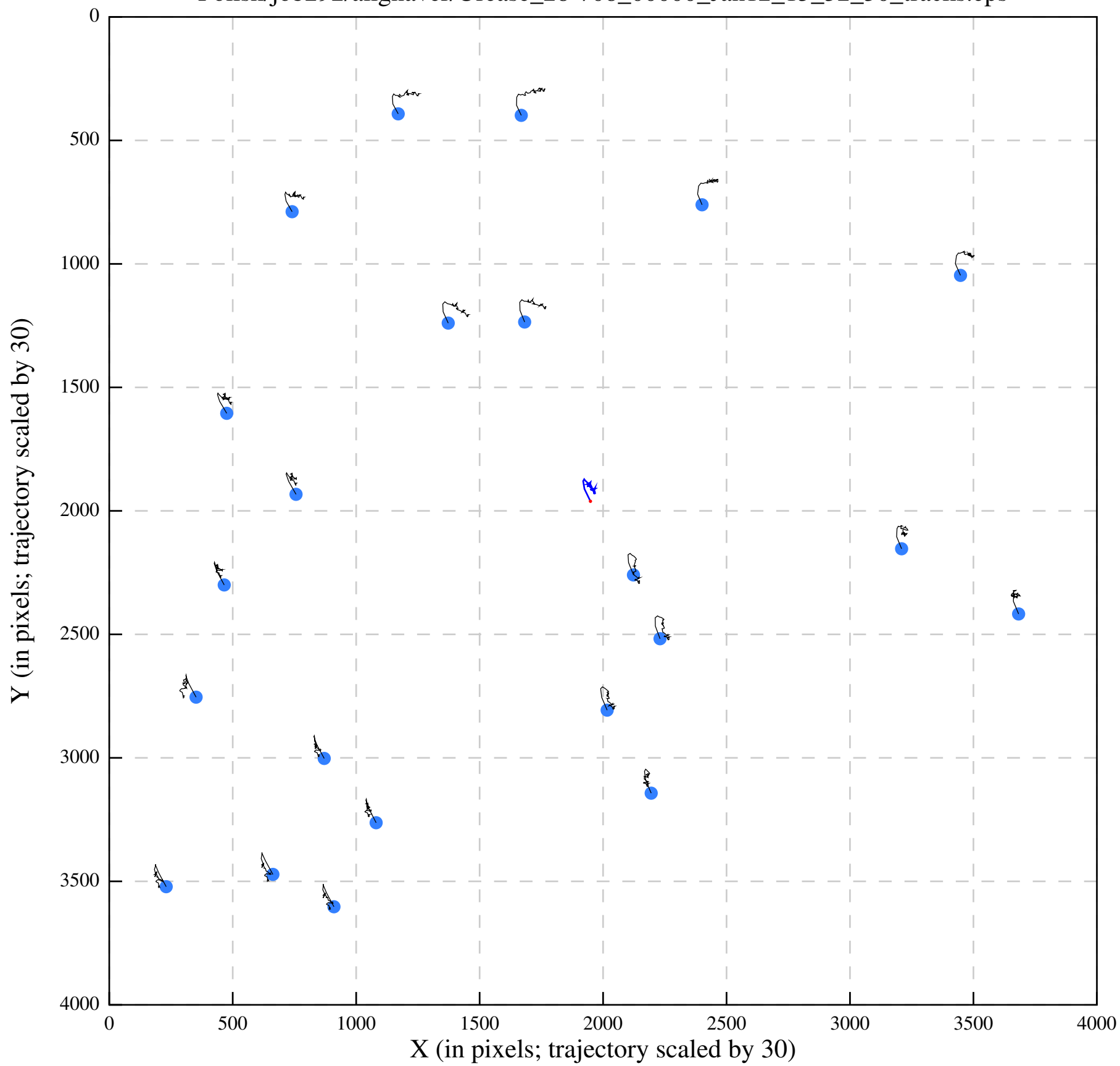
Polish/job292/alignaver/Urease_28-708_00000_Jan12_15_32_30_tracks.eps
