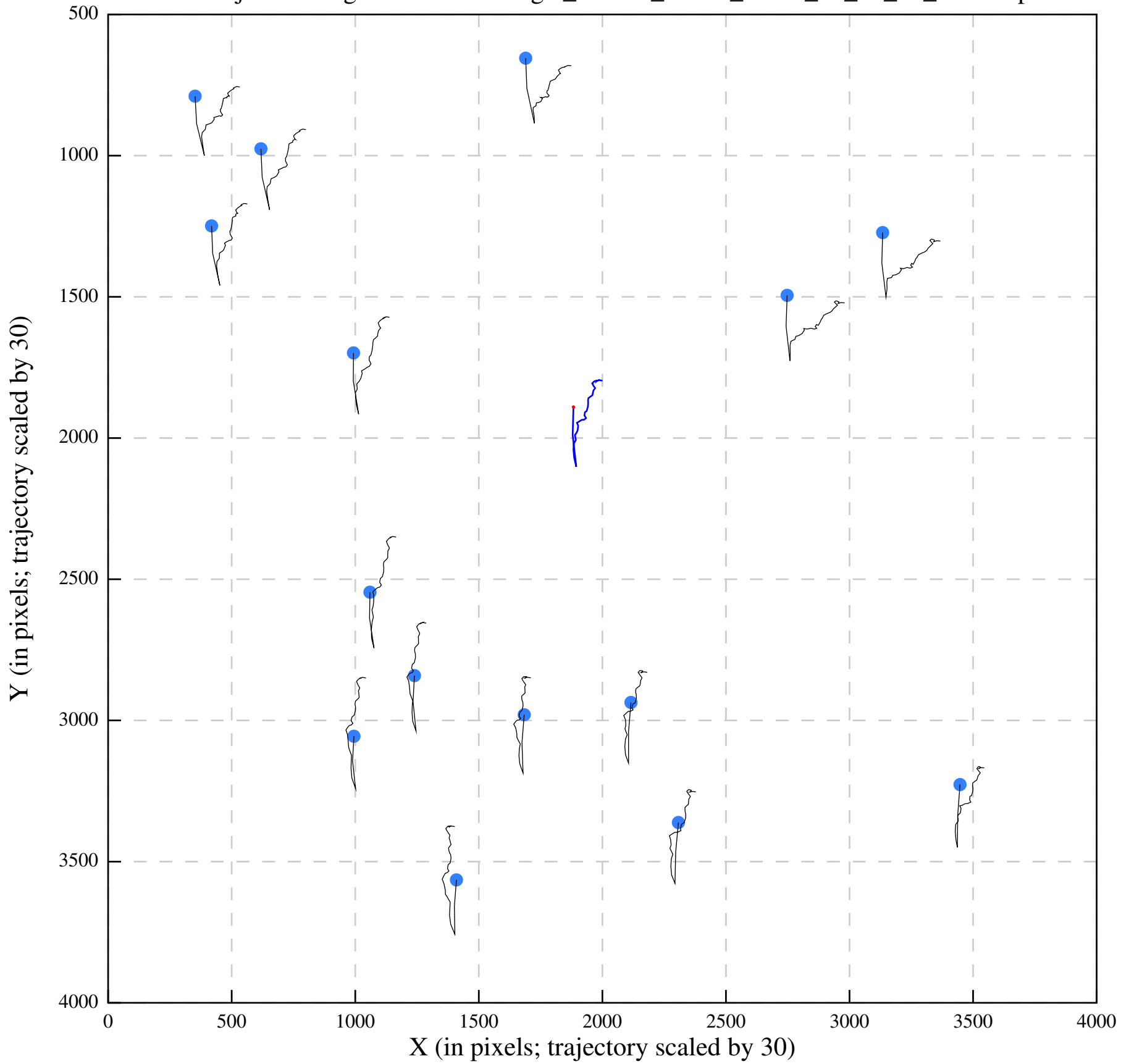
Polish/job292/alignaver/UreaseSingle_35-316_00000_Jan13_15_52_50_tracks.eps
