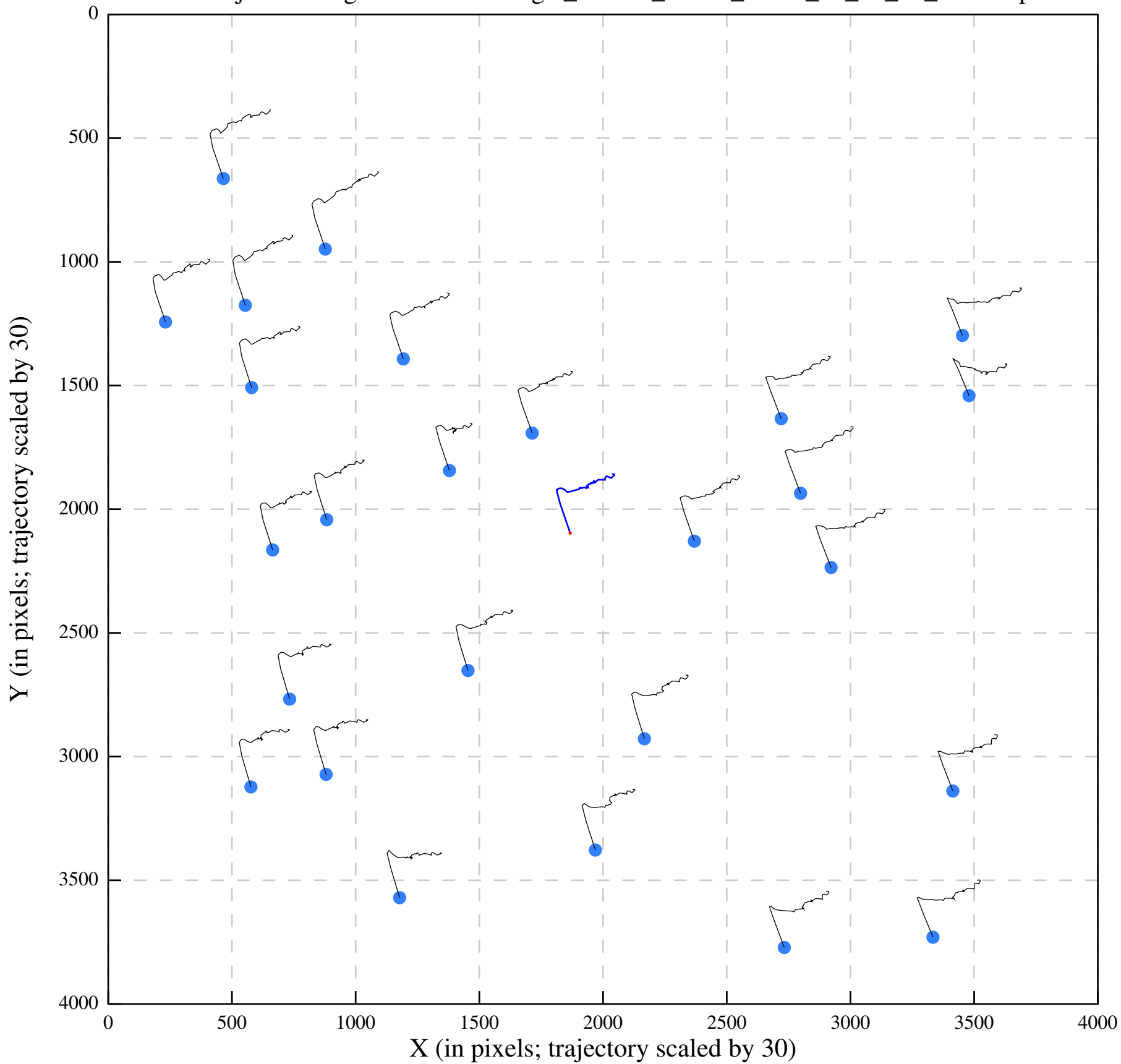
Polish/job292/alignaver/UreaseSingle_41-105_00000_Jan13_23_31_36_tracks.eps
