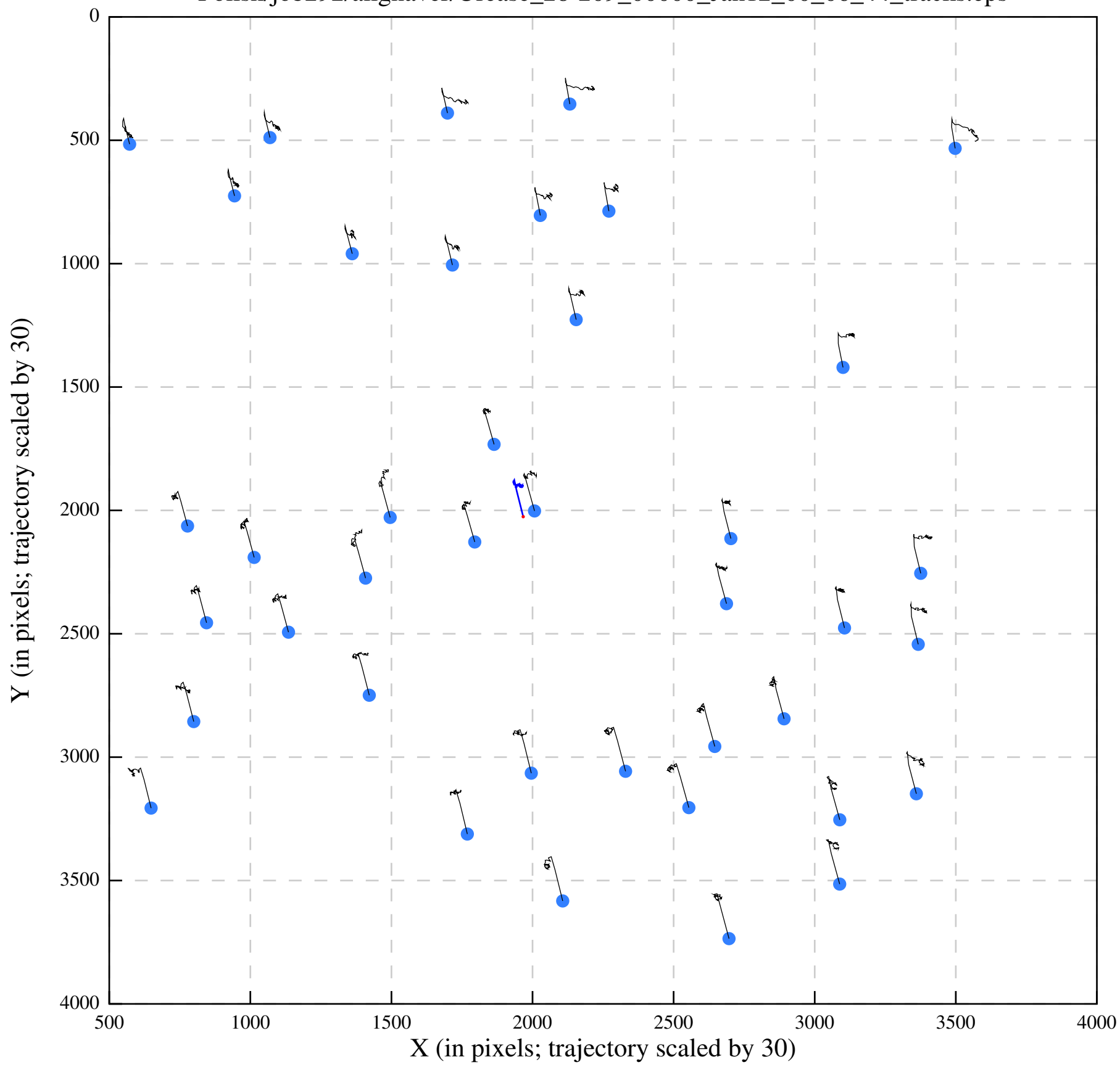
Polish/job292/alignaver/Urease_28-209_00000_Jan12_00_06_44_tracks.eps
