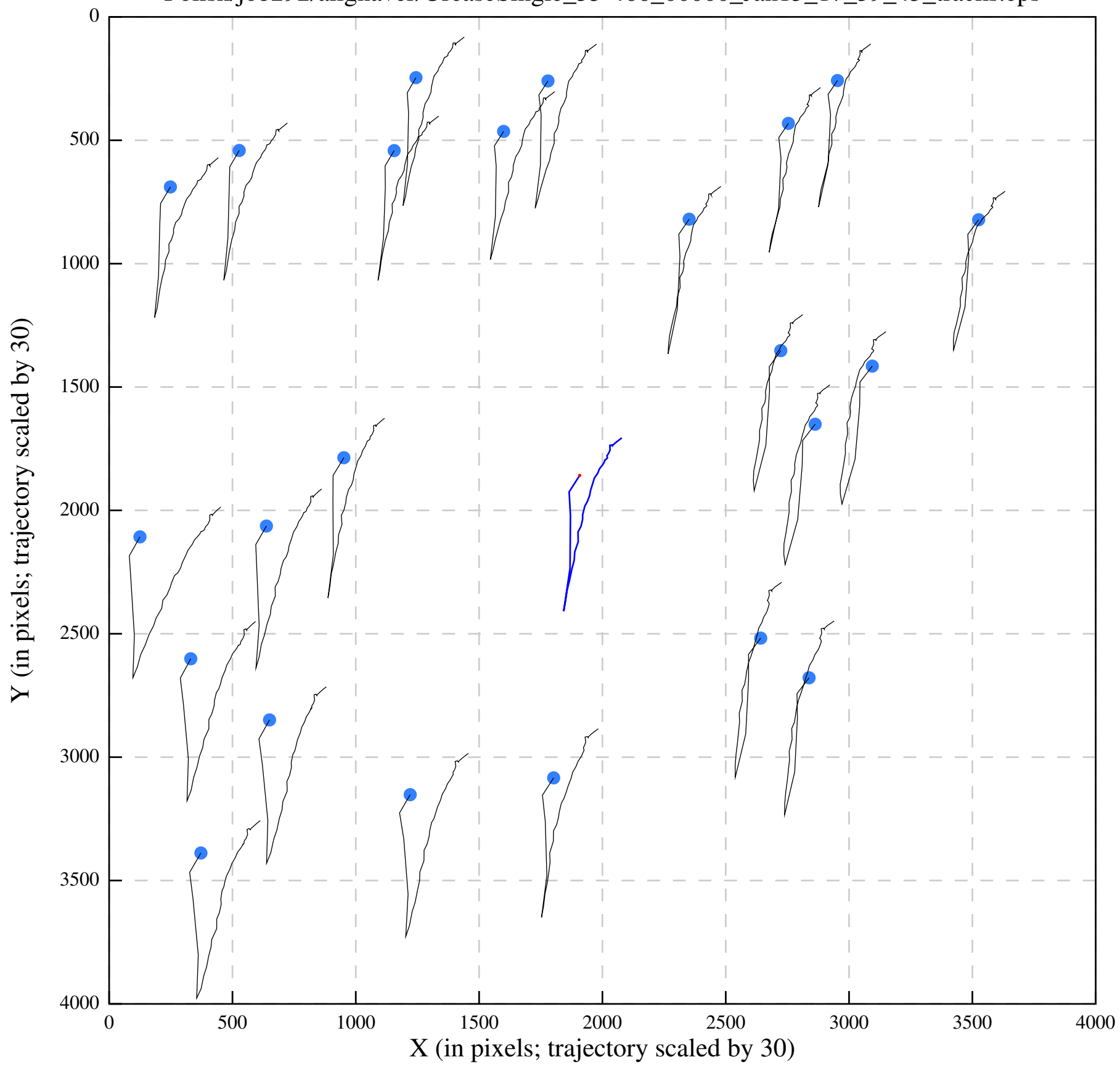
Polish/job292/alignaver/UreaseSingle_35-466_00000_Jan13_17_39_43_tracks.eps
