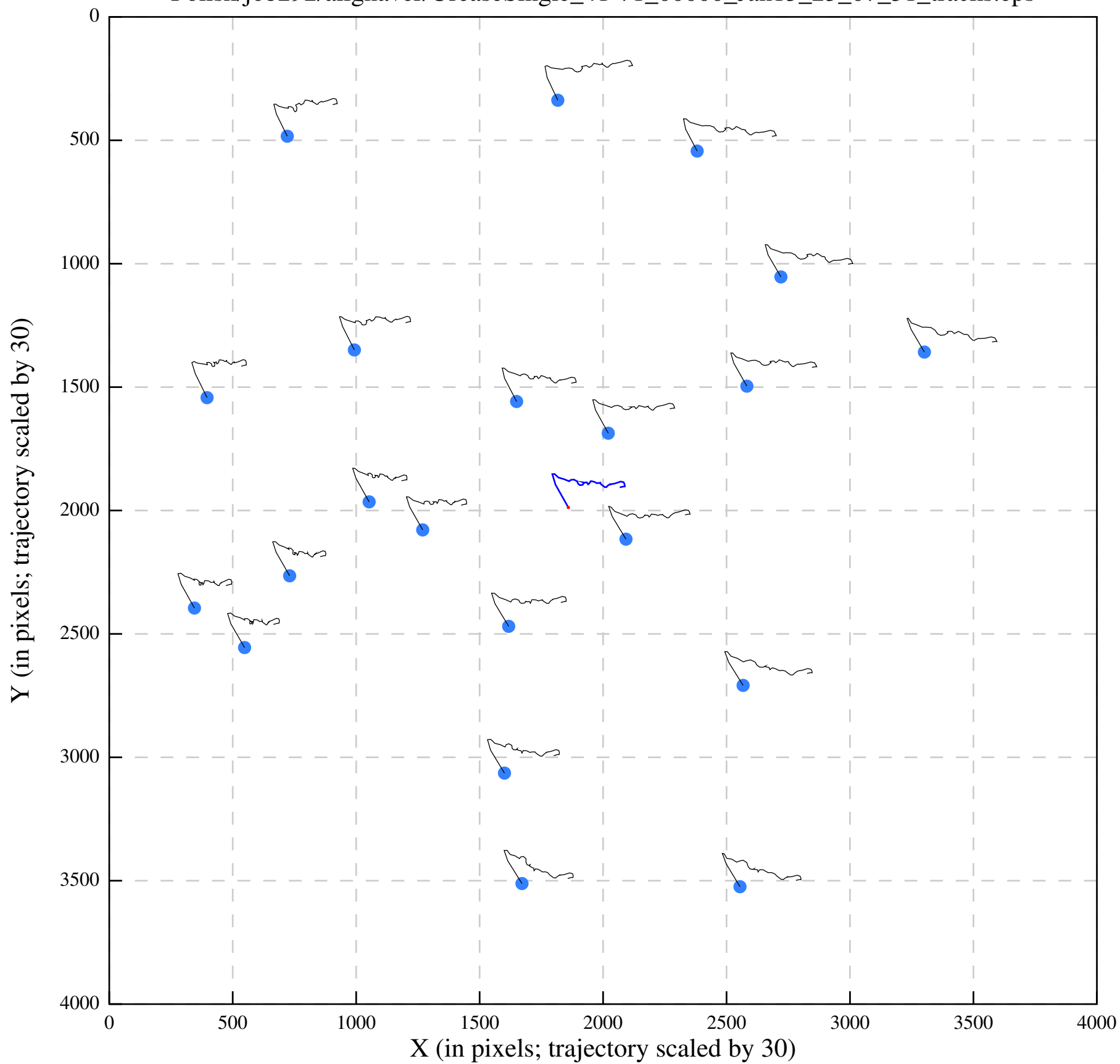
Polish/job292/alignaver/UreaseSingle_41-71_00000_Jan13_23_07_31_tracks.eps
