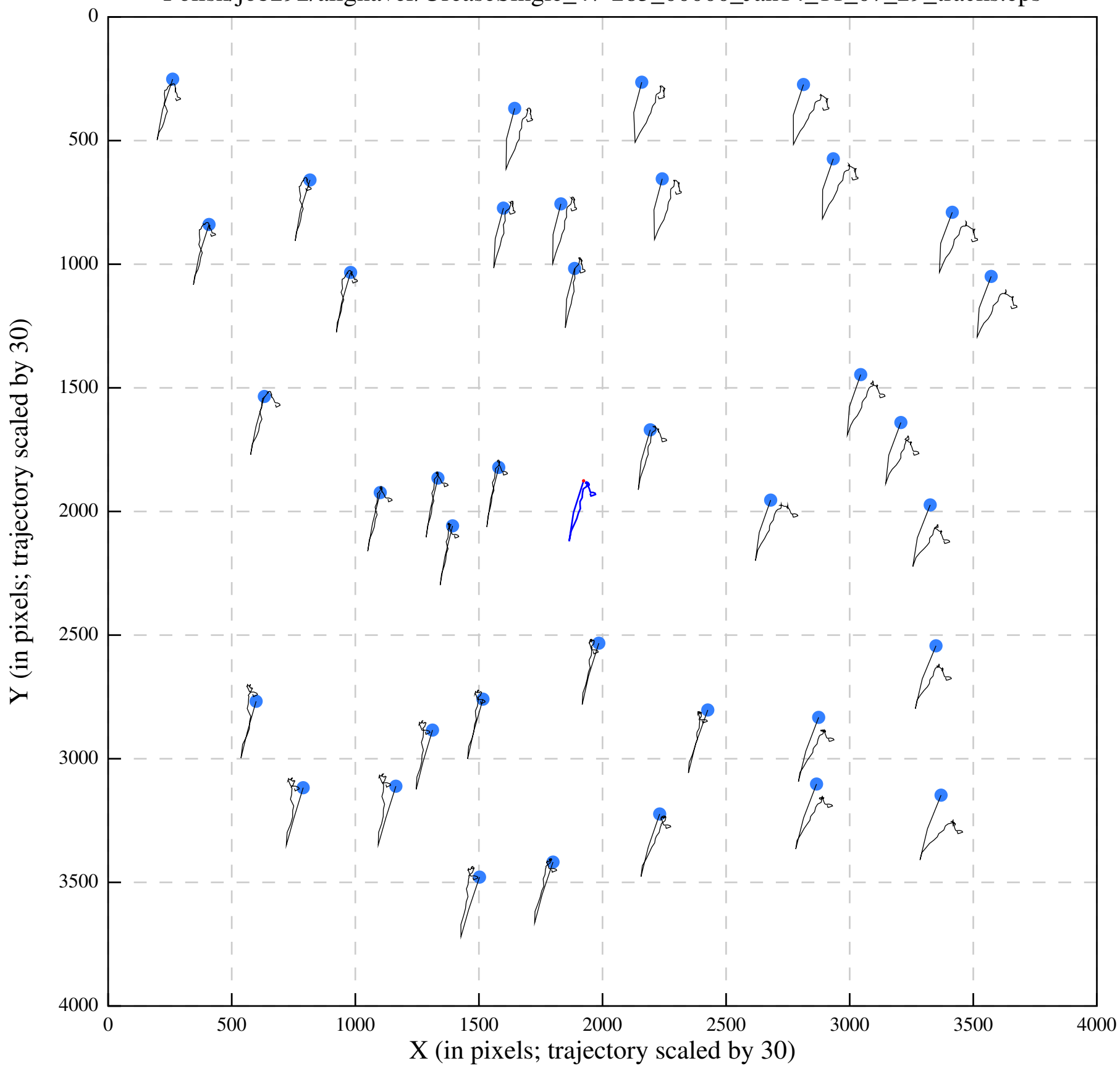
Polish/job292/alignaver/UreaseSingle_47-285_00000_Jan14_11_07_29_tracks.eps
