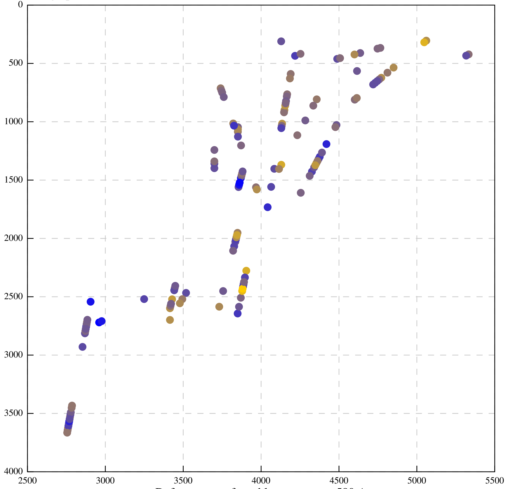
Defocus range from blue to orange: 580 A
