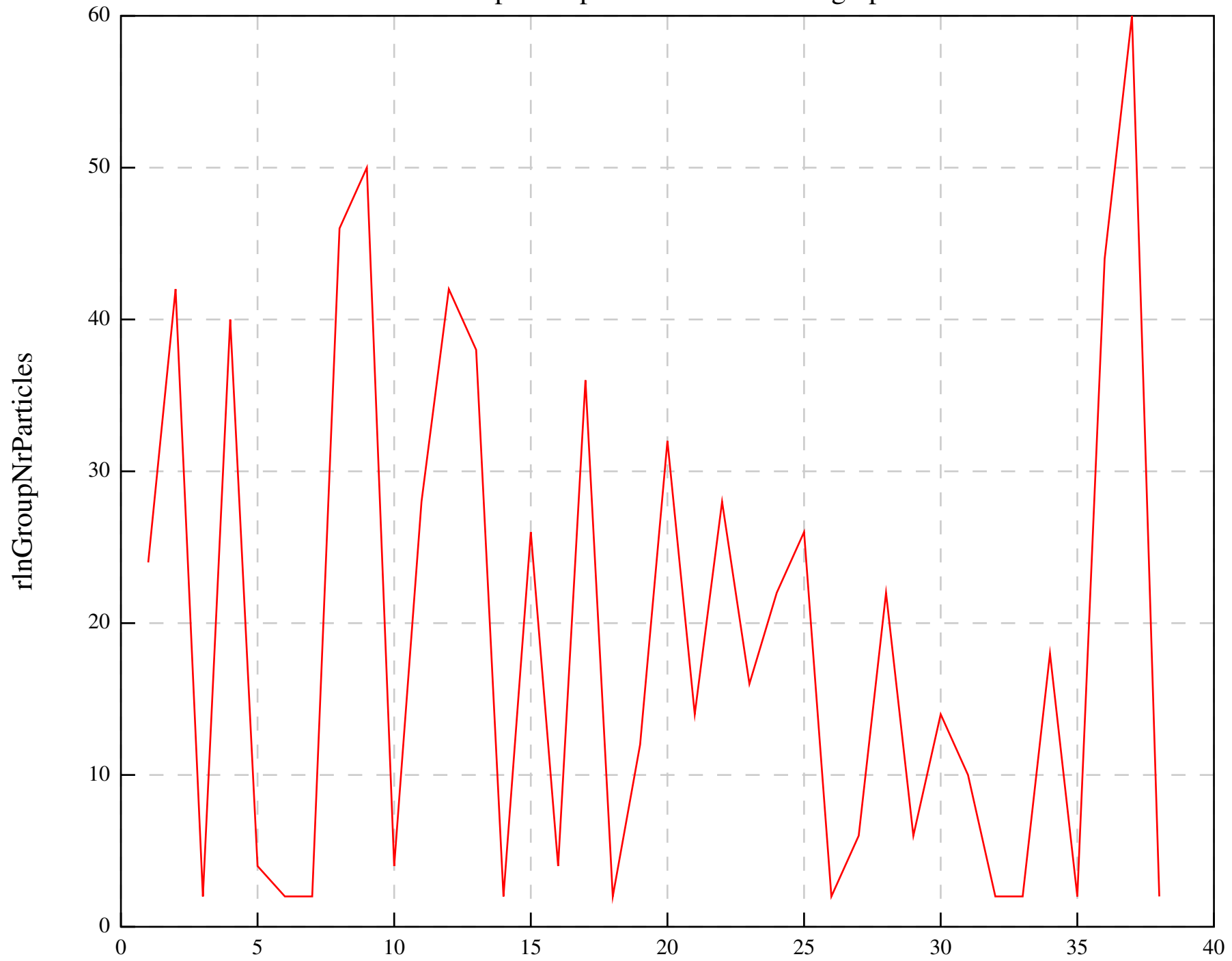
Nr of picked particles for all micrographs
