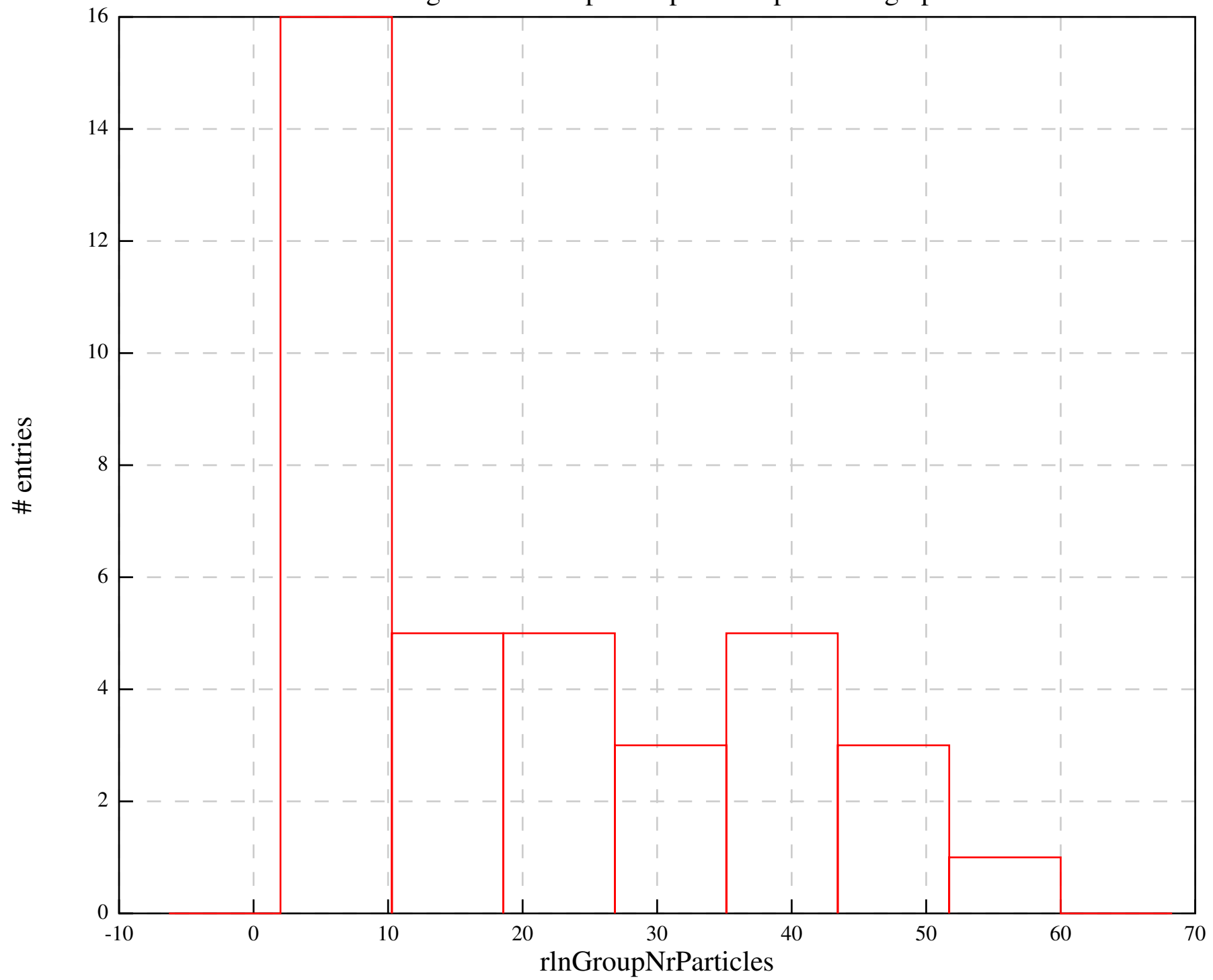
Histogram of nr of picked particles per micrograph
