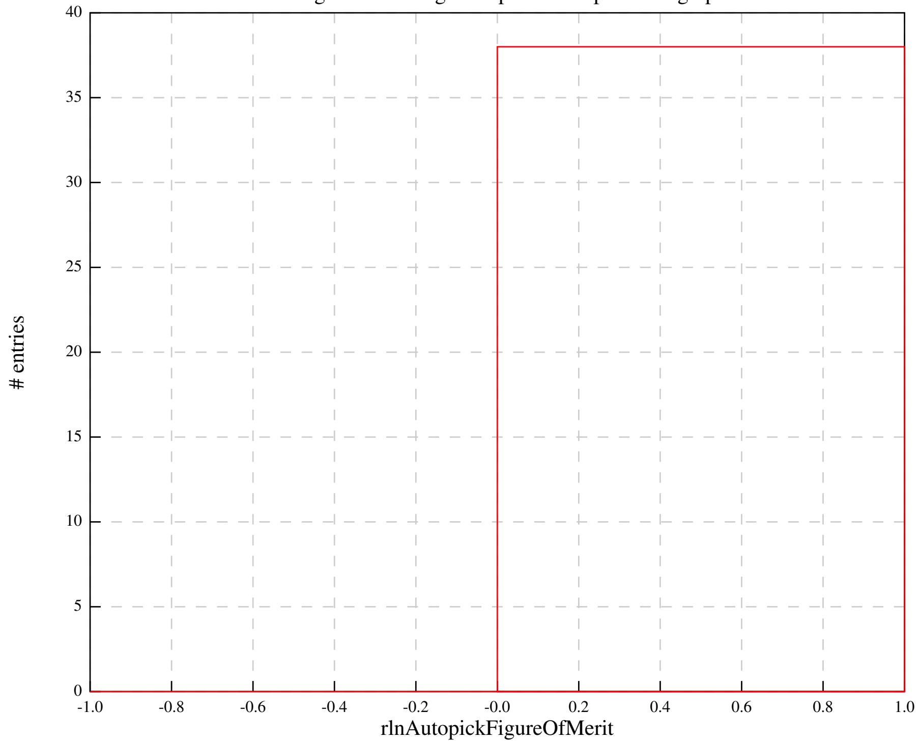
Histogram of average autopick FOM per micrograph
