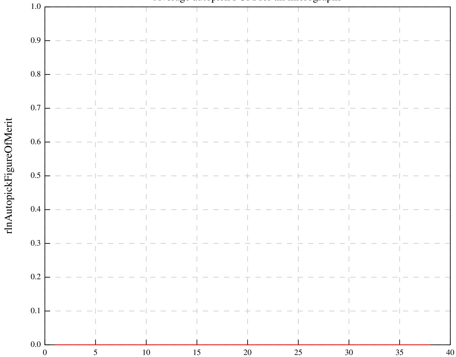
Average autopick FOM for all micrographs
