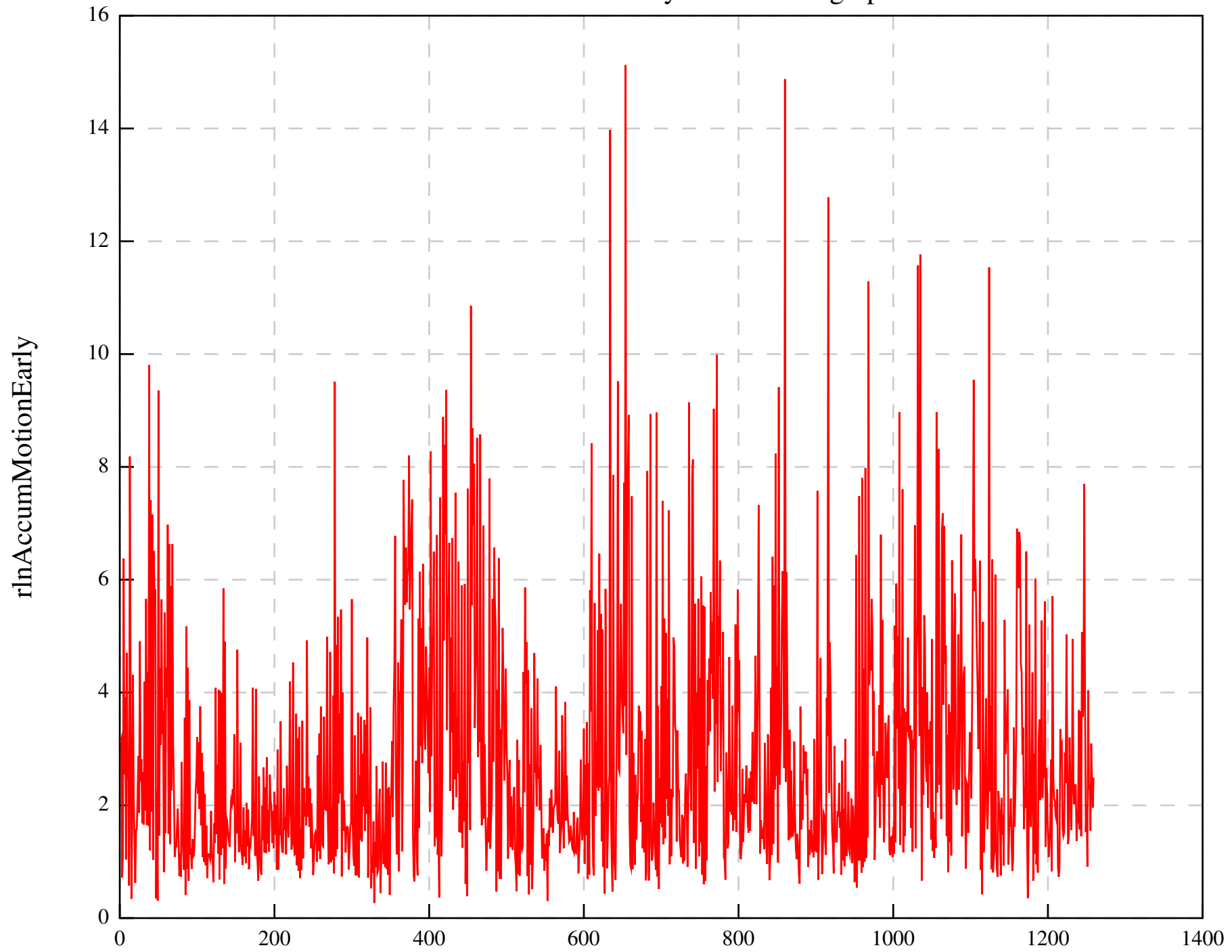
rlnAccumMotionEarly for all micrographs
