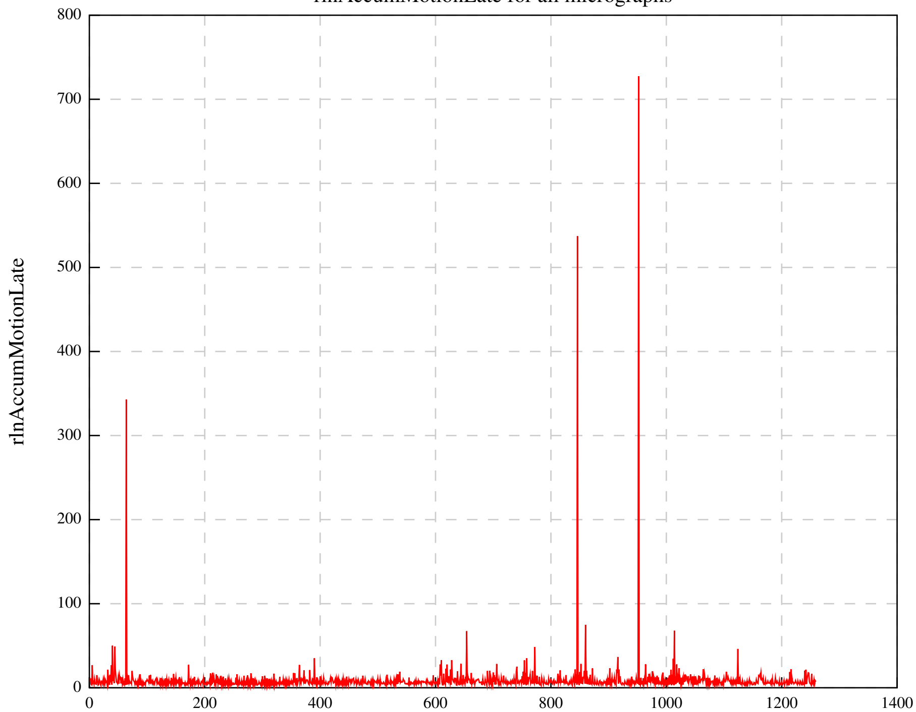
rlnAccumMotionLate for all micrographs
