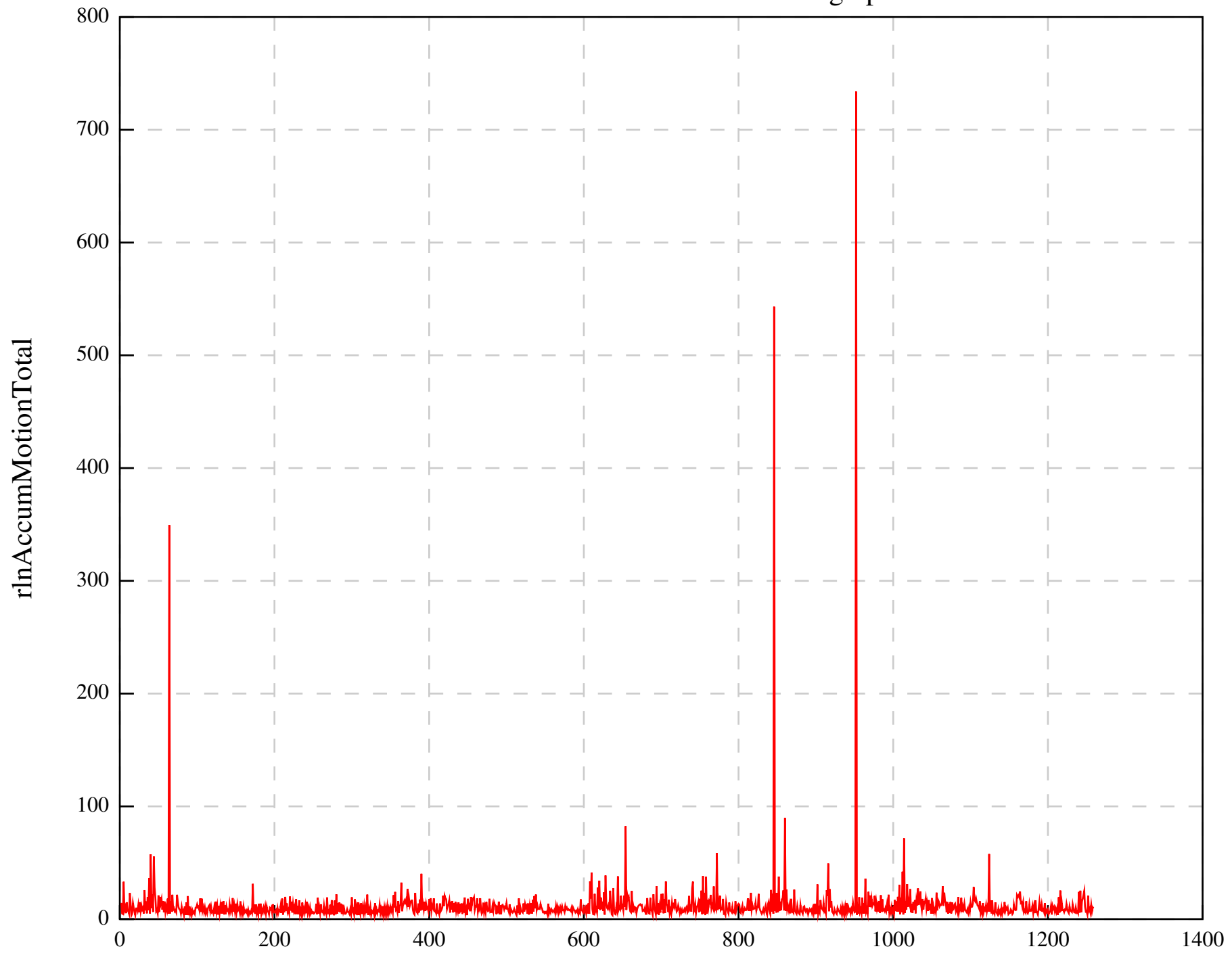
rlnAccumMotionTotal for all micrographs
